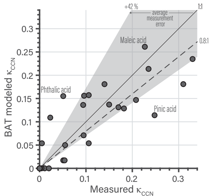
Figure 12. Single-component organic aerosol measurements of \kappa_{\text{CCN}} are compared against those predicted by corresponding BAT model simulations of CCN activation. The gray shading represents \pm 42\% average uncertainty in the measured \kappa_{\text{CCN}} . The dashed line is a linear fit with a zero intercept, \kappa_{\text{CCN,BAT}} = \kappa_{\text{CCN,measured}} \times 0.799 [\pm 0.059] with a Pearson's R^2 of 0.66. The model–measurement RMSE was 0.055. The BAT simulations assume a 100 nm diameter equivalent volume of organic matter at the CCN activation point. The droplet surface tension is calculated as a volume-weighted mean. A list of the 30 measurement points is given in Table S6 of the SI, with the data obtained from the following studies: Broekhuizen et al. (2004); Brooks et al. (2004); Petters et al. (2006); Petters and Kreidenweis (2007); Petters et al. (2009, 2016); Frosch et al. (2010); Huff Hartz et al. (2006); Pradeep Kumar et al. (2003); Raymond (2003); Suda et al. (2014); Svenningsson et al. (2006).
