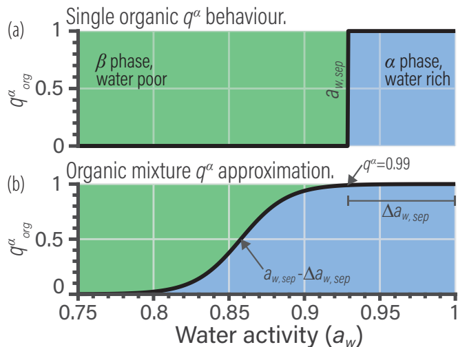
Figure 5. Example of the liquid–liquid phase partitioning for 1-hexanol as a function of water activity, expressed by q_{org}^{\alpha} . The q_{org}^{\alpha} value is only relevant for mixtures that exhibit a miscibility gap. (a) The sharp transition present in a two-component water–organic mixture. (b) The broadening of the organic q_{org}^{\alpha} to better represent behavior in multicomponent organic mixtures (Eq. 21).
