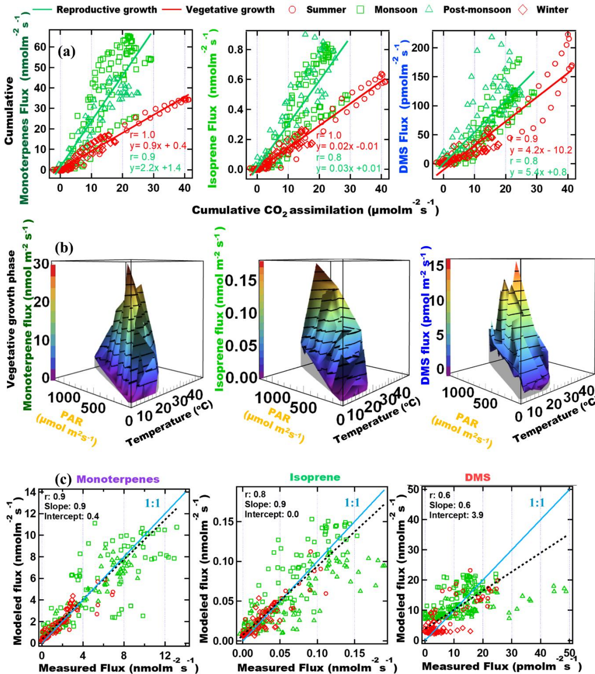
Figure 3(a): Cumulative BVOC emission fluxes versus cumulative \text{CO}_2 assimilation. Cumulative fluxes were calculated for every hour of the day and accumulated from sunrise until that hour, (b) 3-D plot showing the correlation of the emission fluxes with instantaneous chamber temperature and PAR for vegetative growth phase and (c) Modeled versus measured VOC emission fluxes using parameterization presented in Table 3
