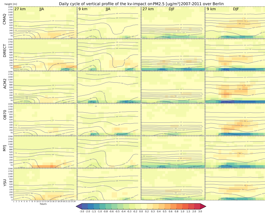
Figure 25. The impact of the urbanization induced Kv enhancement (i.e. increase of vertical eddy diffusivity) on the diurnal cycle of the PM 2.5 profile over Berlin for JJA (columns 1–2) and DJF (columns 3–4) evaluated over the 27 km (columns 1 and 3) and 9 km (columns 2 and 4) domains. Rows correspond to individual Kv -methods. Colors mean the difference, contours stand for the absolute concentrations (from the total-impact). Units in \mu\text{g m}^{-3} .
