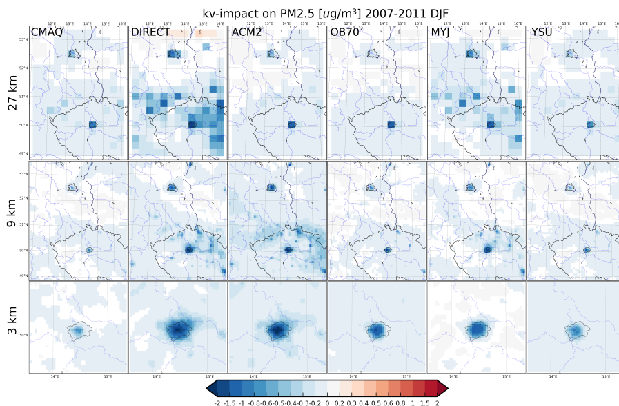
Figure 24. Same as Fig. 23 but for DJF.
