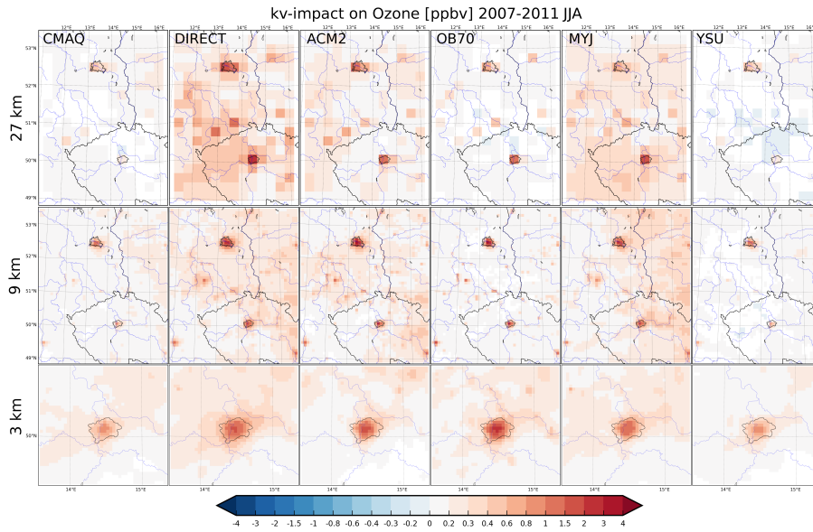
Figure 18. The impact of urbanization induced Kv enhancement (i.e. increase of vertical eddy diffusivity) on surface O_3 concentrations in ppbv for the 27, 9 and 3 km resolutions (top to bottom) for JJA for the six Kv methods (CMAQ, DIRECT, ACM2, OB70, MYJ and YSU). The geographic location of Berlin and Prague is indicated by their administrative boundary. Shaded areas represent statistically significant changes on the 98% level using two tailed t-test.
