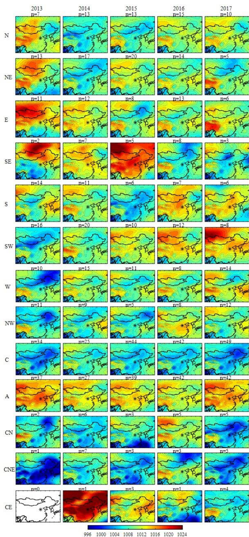
Fig. S8. Pressure field characteristics and occurrence days (n) of weather type N to CE in 2013-2017.
