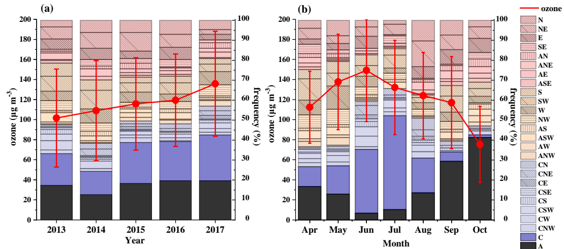
Fig. 3. Interannual (a) and monthly (b) averaged concentrations of ozone and frequencies of 26 weather types from April-October 2013-2017. The red dots represent the mean values, the vertical red lines indicate the standard deviations, and stacked charts represent the percentages of various weather types (2013 and 2014 are averaged for 14 cities; 2015-2017 are averaged for 58 cities). The pink, orange, light blue, dark blue and black areas represent the weather categories N-E-S direction, S-W-N direction, LP, C and A, respectively.
