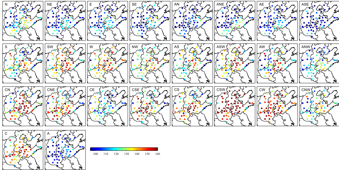
Fig. 6. Spatial distribution of average MDA8 O 3 for the 26 weather types. The first, second, and third rows correspond to the weather categories N-E-S direction, S-W-N direction and LP, respectively, and the fourth row includes both categories C and A.
