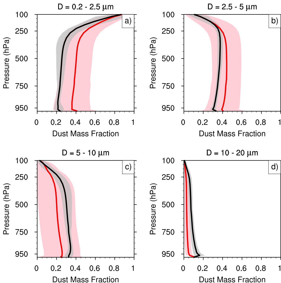
1 2 Figure 7: Vertical distribution of dust mass fractions as a function of particle size for the model ensemble (red lines) and DustCOMM 3 (black lines). The grey and pink shading shows the 95% uncertainty confidence interval for DustCOMM and model ensemble, 4 respectively.
