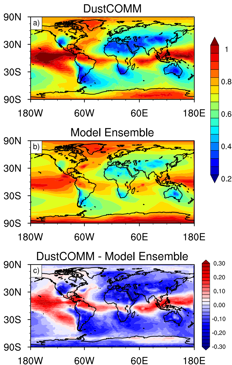
1 2 Figure 9: Spatial distributions of column-integrated dust mass extinction efficiency ( \text{MEE} - \text{m}^2\text{g}^{-1} ), weighted by the dust vertical 3 distribution, for (a) DustCOMM, (b) the model ensemble, and (c) the difference between the two (DustCOMM -Model Ensemble).
