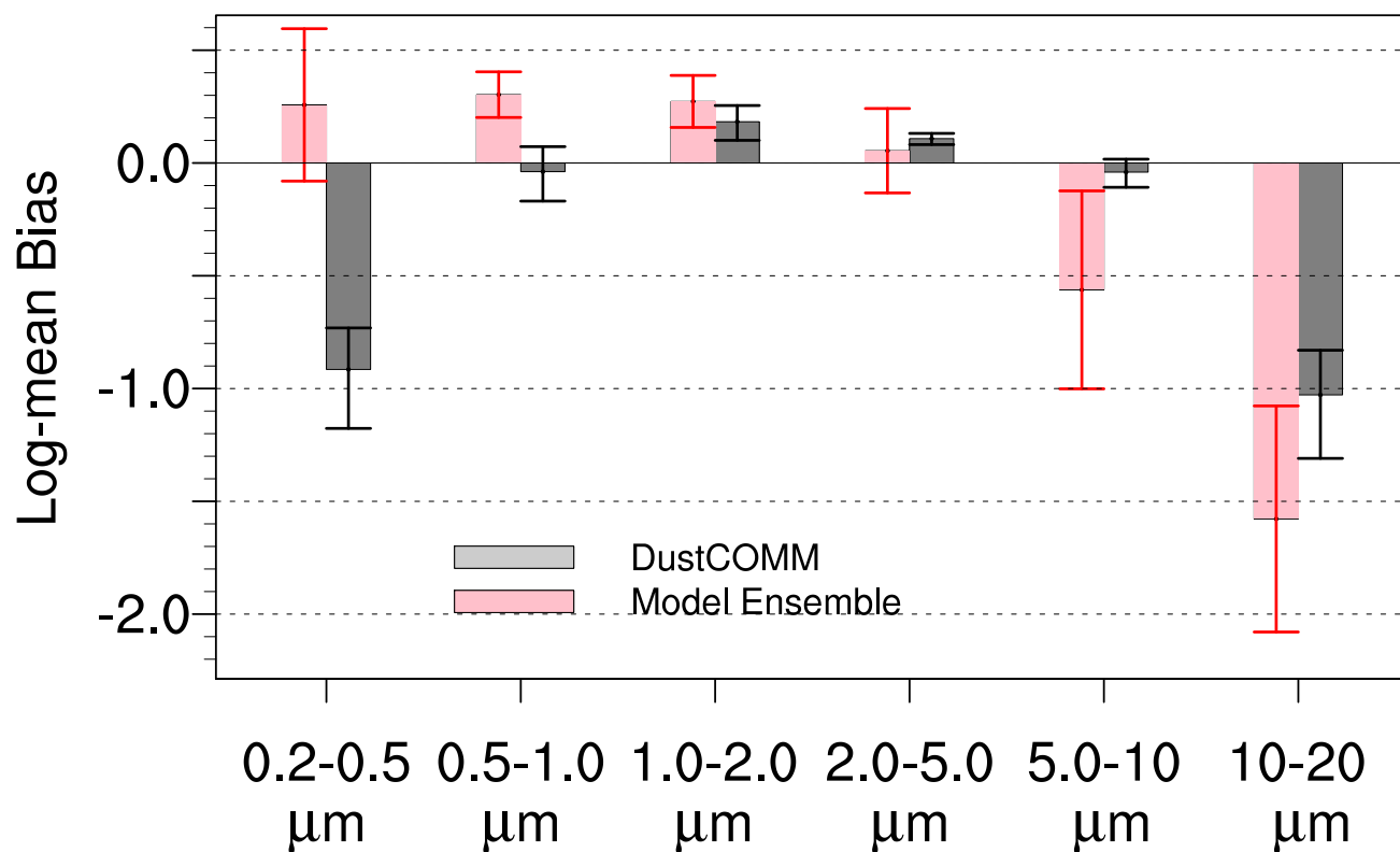
1 2 Figure 4: Average log-mean bias between measurements and DustCOMM (grey) or model ensemble (pink) estimates of dust size 3 distributions (shown in Figures 2 and 3), for different particle bins. The vertical bars represent the 95% confidence interval.
