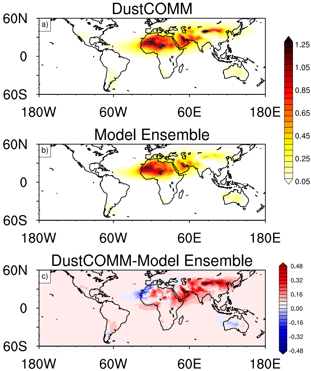
3 4 Figure 10: Spatial distributions of the atmospheric dust column loading ( \text{g m}^{-2} ) for the (a) DustCOMM and (b) model ensemble 5 estimates, and (c) the difference between the two (DustCOMM -Model Ensemble).
