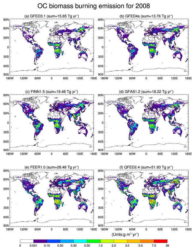
Fig. 1. Figure 2. The spatial distribution of annual total organic carbon biomass burning emissions for 2008 estimated by six biomass burning emission datasets (units: g m -2 yr -1 ).
