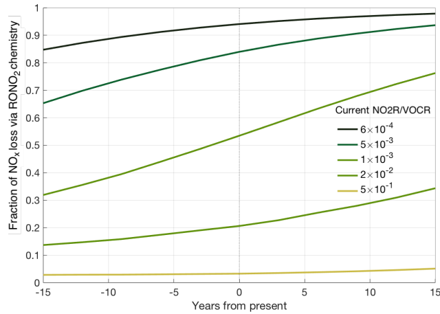
Figure 5. Predicted trends in fractional \text{NO}_x loss over time, calculated from the estimated \text{NO}_2\text{R}/\text{VOCR} ratio assuming a constant -6.5\% \text{ yr}^{-1} decrease in anthropogenic VOC concentrations, a 5.5\% \text{ yr}^{-1} decrease in \text{NO}_x concentrations, and a 1.5\% \text{ yr}^{-1} increase in biogenic VOC concentrations.
