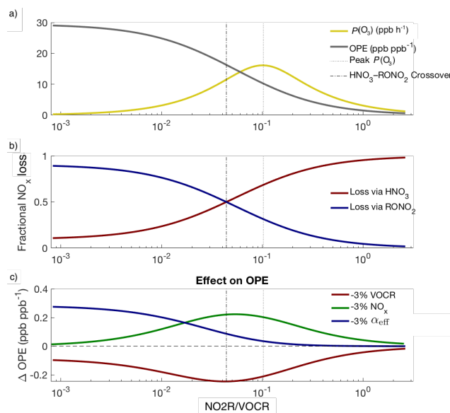
Figure 6. Theoretical picture of NO x and O 3 chemistry, calculated using variable NO x concentrations and fixed VOCR, P(\text{HO}_x) , and \alpha_{\text{eff}} . Panel a shows how P(\text{O}_3) and OPE change as NO x changes; Panel b shows how the fractional NO x loss changes as NO 2 R/VOCR decreases; Panel c shows that changes to NO x and VOCR have their greatest effect on OPE not when P(\text{O}_3) is at a maximum, but at the crossover point between the RONO 2 -dominated and HNO 3 -dominated regimes.
