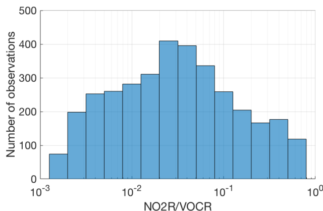
Figure 2. Comparison Number of the relative production rates of \text{RONO}_2 and \text{HNO}_3 as a function of \text{NO}_2\text{R}/\text{VOCR} . Used data points are restricted to in each bin for which the continental summertime boundary layer (i.e., over land, less than 1.5 km above ground level, and average temperature > 10^\circ\text{C} ). The top panel shows the fraction of \text{NO}_x loss attributable to occurring via \text{RONO}_2 chemistry, as well as a least-squares fit to the data and the expected behavior if \alpha_{\text{eff}} , f_{\text{NO}_{\text{eff}}} , Y_{\text{RO}_2\text{eff}} were constant could be calculated . The bottom panel shows the ratio of \Sigma\text{RONO}_2 to the sum of \text{HNO}_3 and \Sigma\text{RONO}_2 . In each panel, the blue diamonds show the median in each bin and the vertical lines show the interquartile range.
