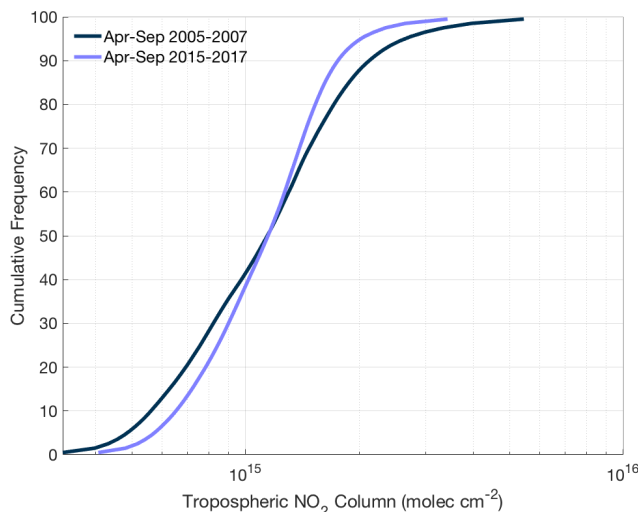
Figure 8. Cumulative frequency distribution of OMI tropospheric NO 2 columns over the continental United States using the BEHR v3.0A retrieval for summer (Apr–Sep) in 2005–2007 and 2015–2017.
