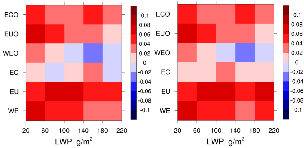
Figure 6. The differences between \text{CER}_{2.1\mu\text{m}}\text{-AOD (AI)} slope and \text{CER}_{3.7\mu\text{m}}\text{-AOD (AI)} slope under all LWP bins over three anthropogenic regions (EC, EU, and WE) and their adjacent oceans (ECO, EUO, and WEO).
