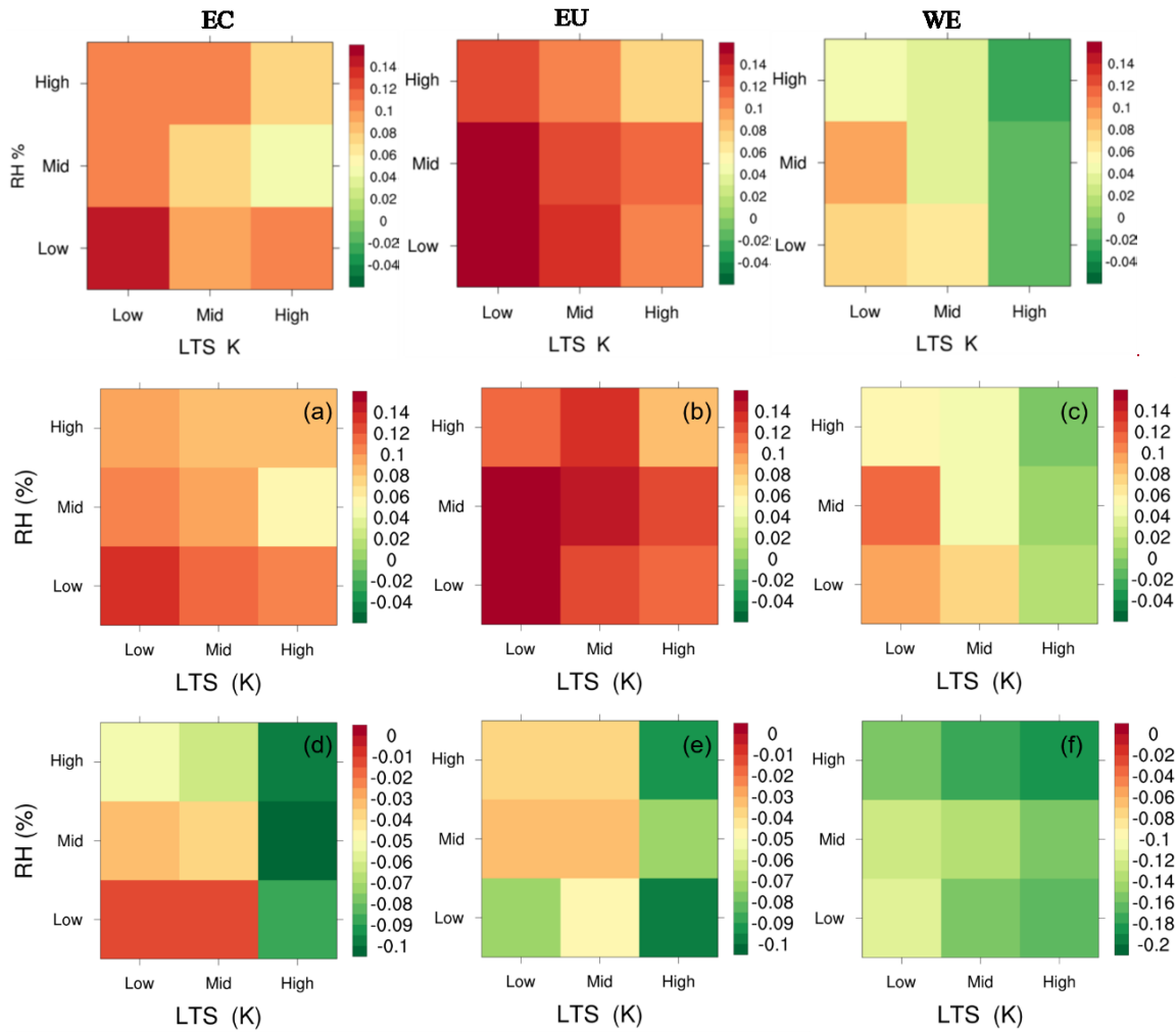
Figure 9. The slopes of CER versus AOD(AI) on log-log scale under low, medium, and high LTS and RH_{CT} conditions, respectively, over (a) EC, (b) EU, (c) WE, (d) ECO, (e) EUO, and (f) WEO and (EC, EU, and WE).
