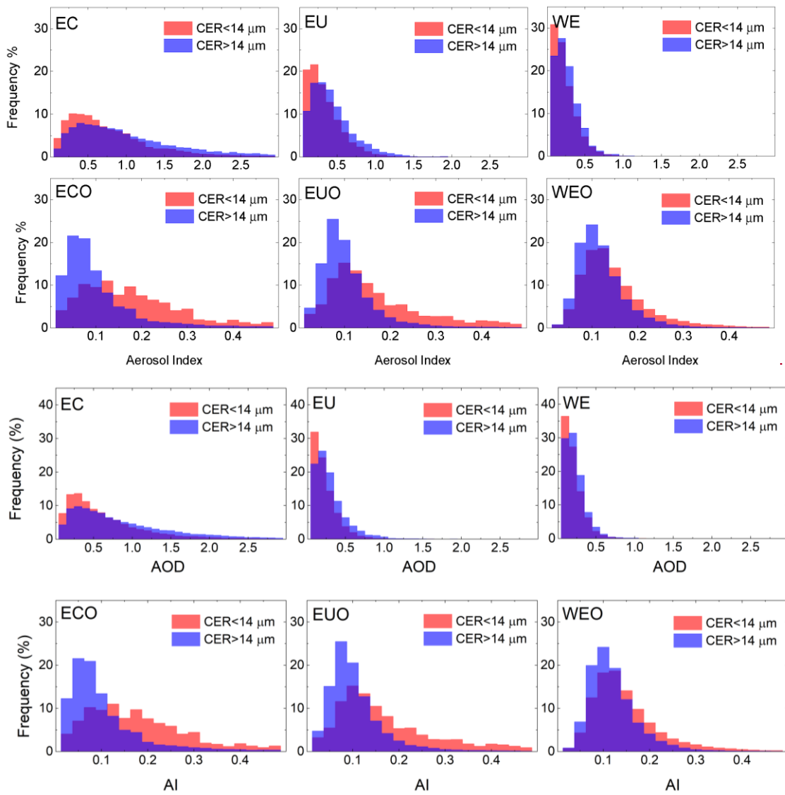
Figure 8. Probability density functions of AOD (AI) for CER > 14 \mu\text{m} (blue) and CER < 14 \mu\text{m} (red) over three anthropogenic regions (EC, EU, and WE) and their adjacent oceans (ECO, EUO, and WEO).
