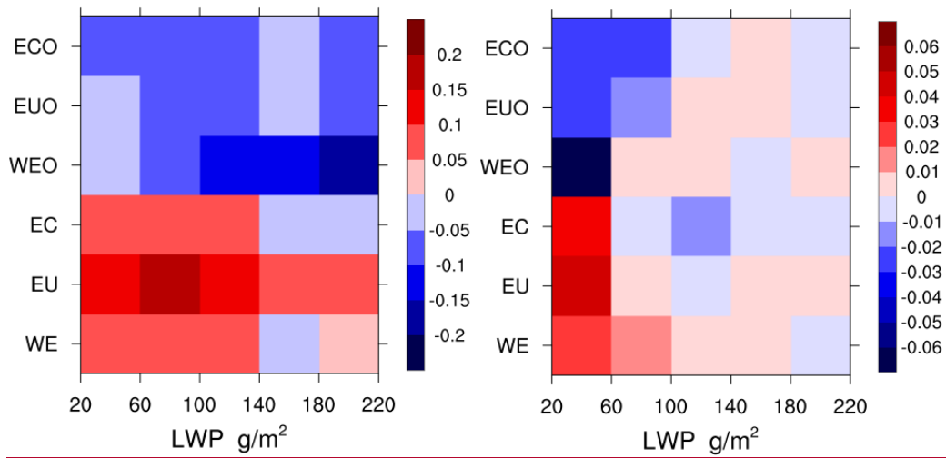
Figure 2. The computed slopes of (a) CER versus aerosol loading (AOD for land, AI for ocean)AI (Ma et al., 2018) and (b) LWP versus AI-aerosol loading on log-log scale over six regions, in which data are stratified according to LWP.
