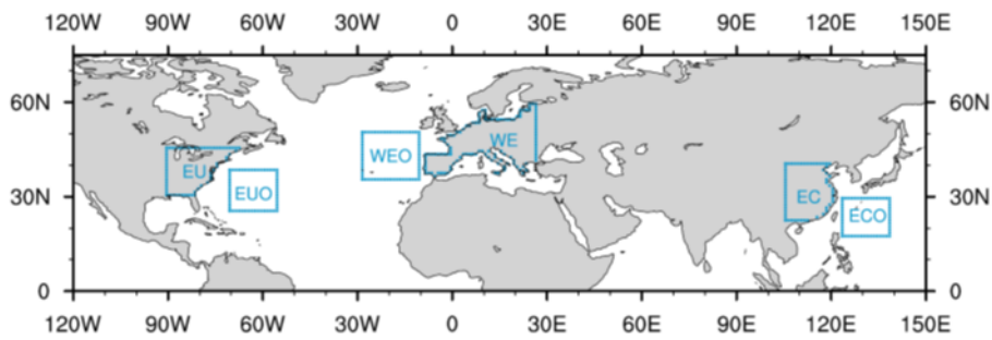
740 Figure 1. Regions analyzed in this study: three anthropogenic regions (EC, EU, and WE) and their adjacent oceans (ECO, EOU, and WEO).
