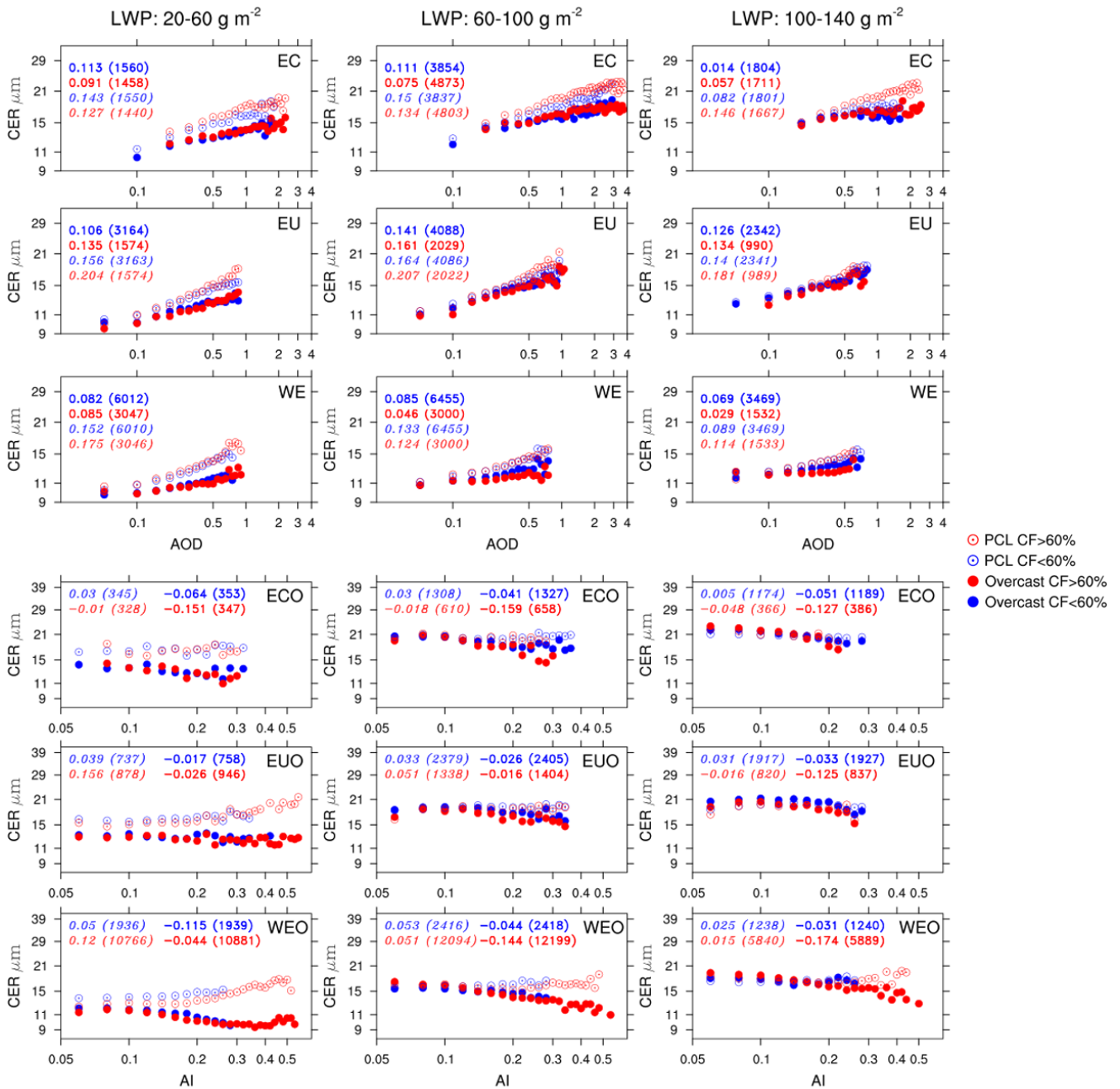
Figure 5. Cloud effective radius (CER) varies with aerosol loading (AOD for land, AI for ocean)-aerosol index (AI) under three liquid water path (LWP) categories (20~60, 60~100, 100~140 g m -2 ). The figures from top to bottom show the CER-AOD/AI correlation over different regions (EC, EU, WE, ECO, EUO, WEO). The circles (dots) show the mean CER from PCL (overcast) retrieval at each categories of AOD (AI) bin in case of PCL (overcast) retrieval CF > 60% (red) and CF < 60% (blue), respectively . The slopes on log-log scale along with the total number of samples (bracketed) for these four categories are also provided in each panel, in which the numbers in italic (bold) represent PCL (overcast) retrieval.
