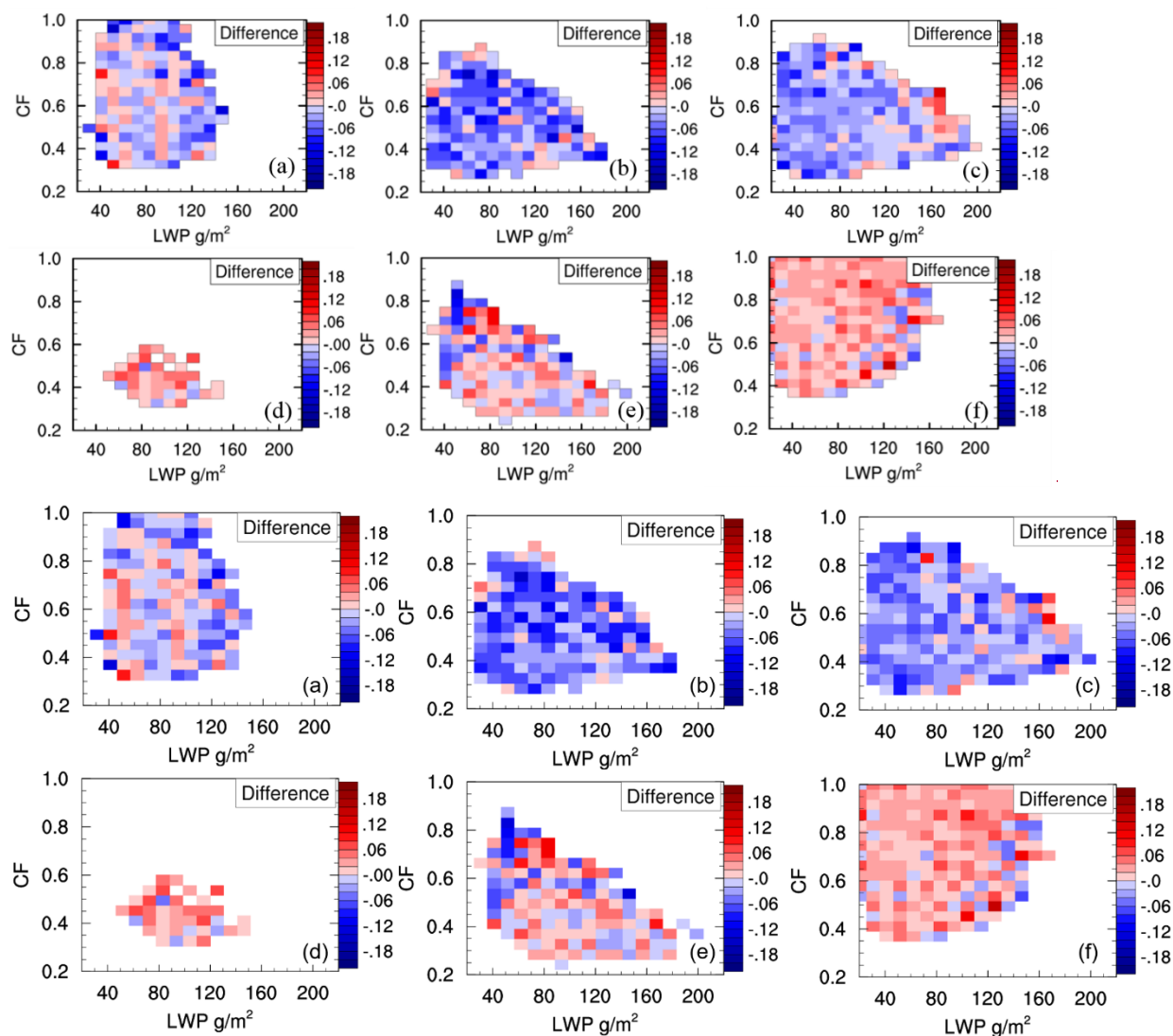
Figure 4. The difference of TOA albedo for polluted ( \text{AOD}/\text{AI} > 75\text{th percentile} ) and clean case ( \text{AOD}/\text{AI} < 25\text{th percentile} ) ( \Delta\alpha ) over (a) EC, (b) EU, (c) WE, (d) ECO, (e) EUO, and (f) WEO, in which data are stratified according to both LWP (x axis) and CF (y axis).
