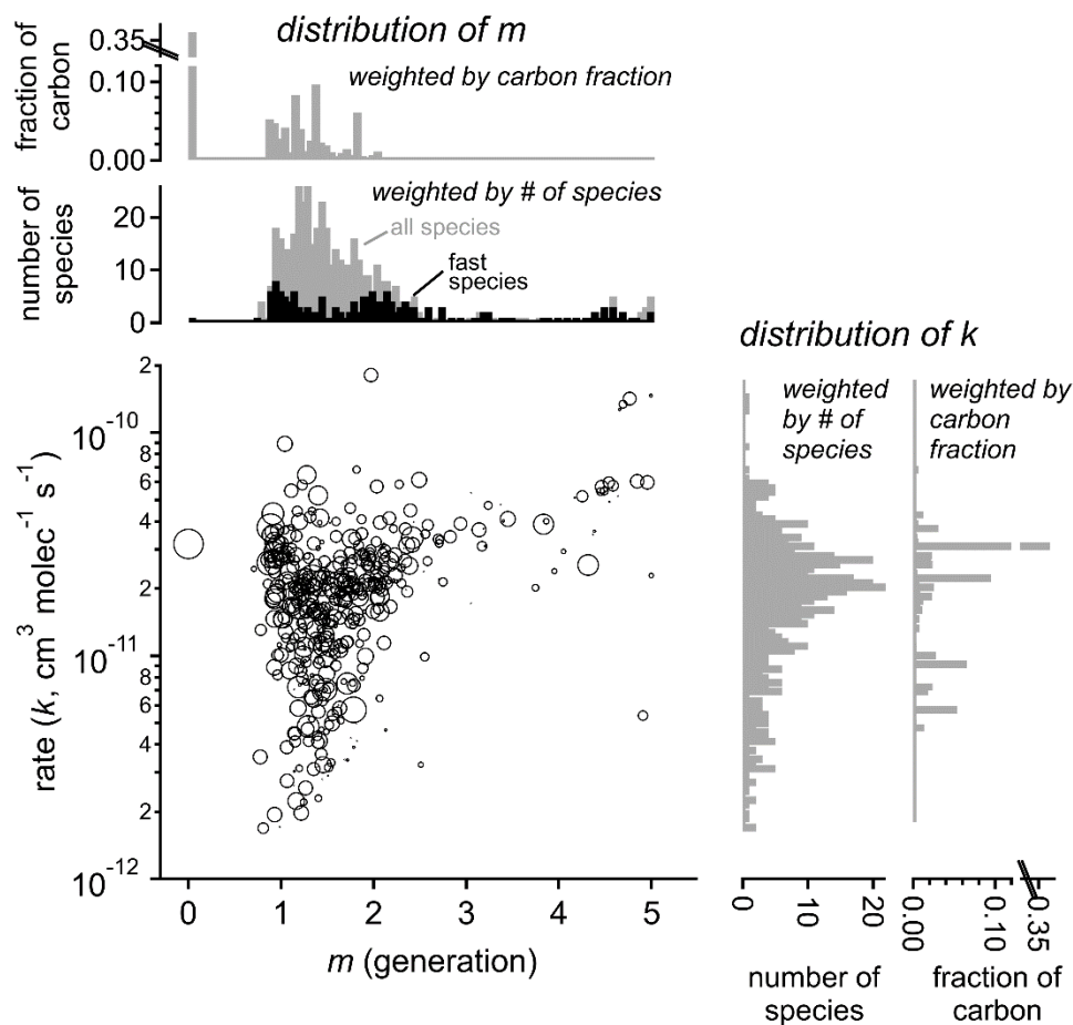
660 Figure 11 Parameterized rate constant and generation number for 463 species detected during the chamber experiment OH-initiated oxidation of trimethylbenzene. Marker area corresponds to \log(\text{ppb carbon}) of detected species, averaged over the duration of the experiment. “Fast-reacting” species, defined as having an effective rate constant at least 75% that of the precursor, are highlighted as black bars in the histogram of m . These tend to center on integer values of generation number.
