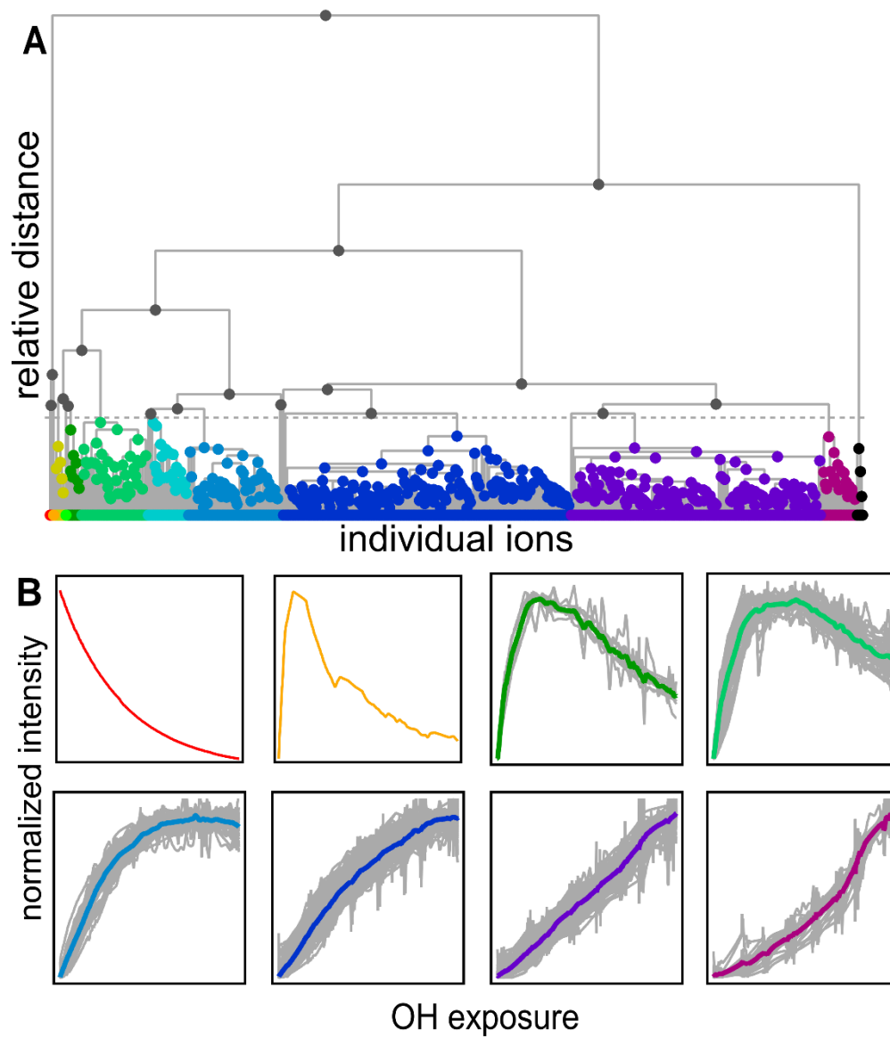
550 Figure 7A. Hierarchical cluster relationship of all measured species from the chamber experiment. Clusters are colored at a relative distance cut-off (gray dashed line) that separates 1,2,4-trimethylbenzene from all other products, with gray lines showing linkages between species and clusters. The individual clusters are distinguished by different colors. B. Time series of eight example clusters. The x-axis in each plot is OH exposure, and the y-axis is the normalized intensity. The cluster average
