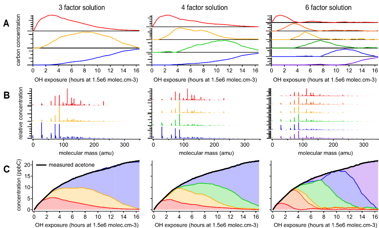
Figure 4 Positive matrix factorization of chamber data, showing solutions with three, four, and six factors. A. Time series of PMF factors. B. Compositional profiles of factors, shown as combined mass spectra from all instruments with CO, CH 2 O, and CIMS measurements at their exact molecular masses and OA shown with a molecular mass of -1. C. Apportionment of the concentration of acetone (a long-lived oxidation product signal) across all factors. Within each column, the assigned color of each factor is consistent. As in the PMF analysis of the synthetic data set (Figure 3), factors do not correspond to generations, and long-lived species (such as acetone) are assigned to successively later-peaking factors over the course of the time series.
