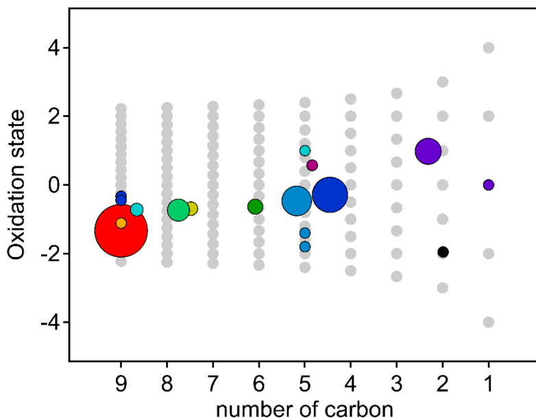
575 Figure 8 Average oxidation state and number of carbon atoms per molecule for each cluster determined from HCA of chamber data. The individual clusters are distinguished by color, and the color scheme is the same as in Figure 7. The contribution of each species to the cluster average is weighted by parts-per-billion-carbon (averaged over the entire experiment). Marker area is proportional to the averaged concentration (parts-per-billion carbon) of all species in the cluster, with the marker size of the precursor (red) decreased by a factor of 2 for legibility. Clusters cover a substantially wider area of chemical space than PMF 580 factors (Figure 5).
