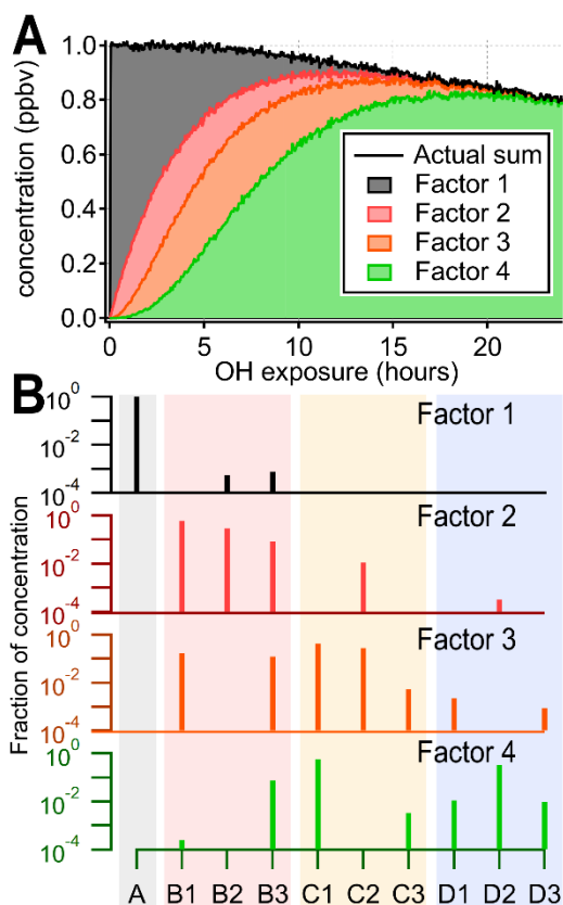
425 Figure 3 Results from PMF analysis of the synthetic data set, showing the 4-factor solution. A. Total intensity of synthetic data compared to stacked time-series of PMF factors. B. Profiles of PMF factors, illustrating that factors do not correspond to individual generations. The shaded background corresponds to generation: precursor (black), first-generation (red), second-generation (yellow), third-generation (blue). The color of the mass spectra corresponds to panel A. Solutions with different numbers of factors are given in the supplemental information.
