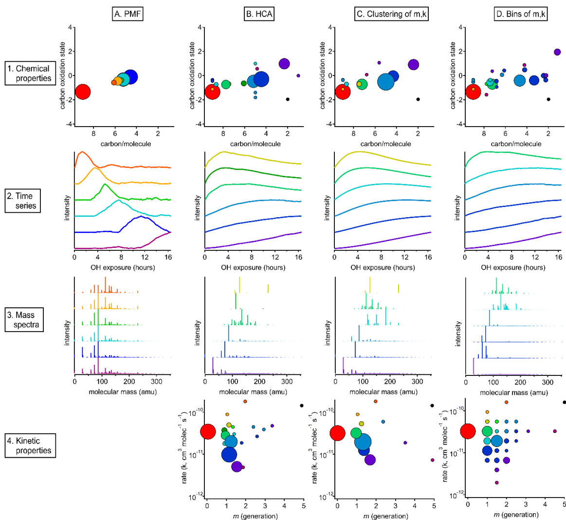
Figure 13 Overall comparison of groups derived from PMF, HCA, and GKP of chamber data. The columns show, from left to right, the results of A. PMF, B. HCA, C. GKP best-fits grouped using HCA, and D. measurements grouped by GKP fit parameters. The rows show, from top to bottom, 1. the average carbon oxidation state and number of carbon atoms per molecule for each group, 2. the time series of the six groups containing the most carbon, 3. the mass spectra of those six groups, and 4. the rate constant and generation number of each group. Within each column, each chemical group is assigned a specific color. This color scheme is the same for each plot within a column. The marker area is proportional to the averaged concentration (ppb carbon) of all species in the group, with the marker size of the precursor (red) decreased by a factor of 2 for legibility. The marker area scheme is consistent across all plots. PMF factors do not have kinetically realistic time series, therefore there is no plot A4.
