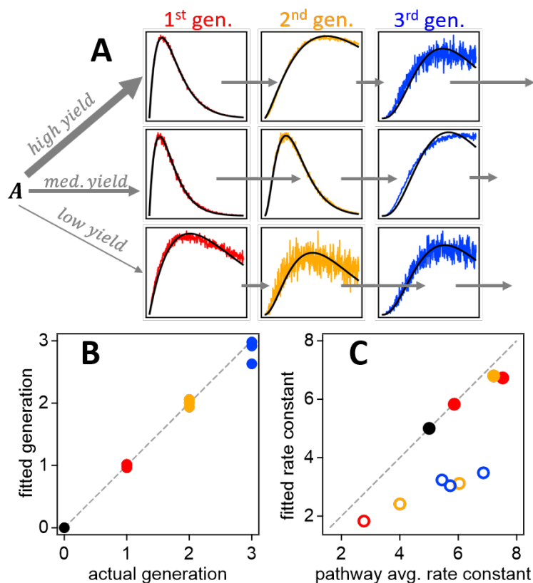
600 Figure 9 Best fit of the gamma kinetic parameterization to synthetic data (GKP, Eq.3). A. Time series of synthetic data (colored lines) and best-fit (black lines). First-generation species are shown in red, second-generation in yellow, and third-generation in blue. The relative rate constants are indicated by short arrows (slow rate constant) or long arrows (fast rate constant). B. Fitted generation compared to actual generation. The colors correspond to the generations shown in panel A. C. Effective rate
