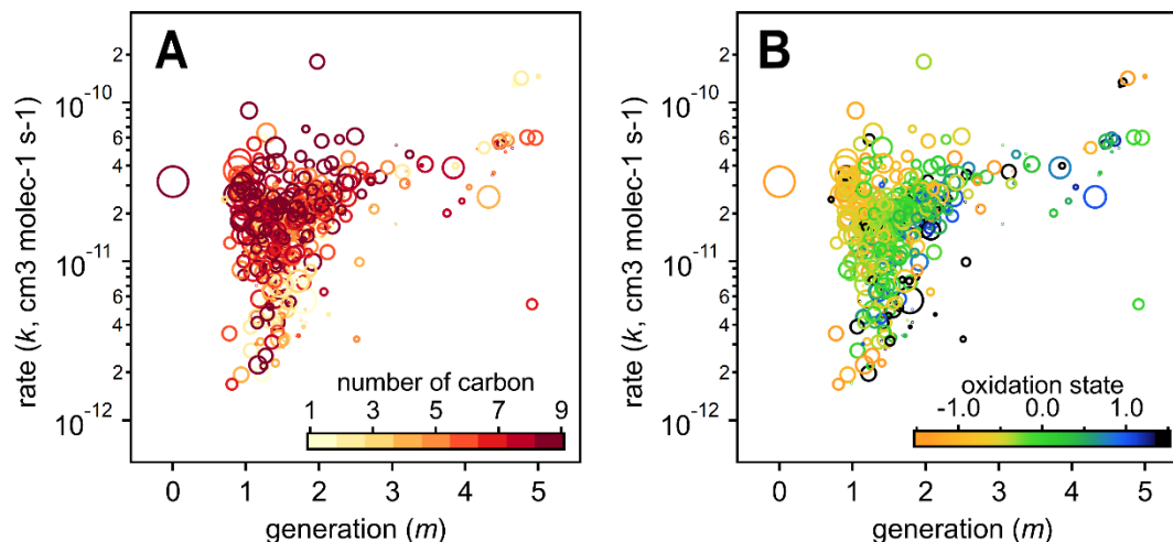
670 Figure 12 Relationships of kinetic parameters (from the GKP of chamber data) with key chemical properties of reactive species. A. Generation ( m ) and rate ( k ) values of 1,2,4-trimethylbenzene precursor and products, colored by number of carbon atoms. B. Same as A, but k and m colored by carbon oxidation state. Marker area corresponds to \log(\text{ppb carbon}) . The early generation and fast-reacting products tend to have higher numbers of carbon atoms and are less oxidized, while later generation and slow-reacting products tend to be smaller and more oxidized.
