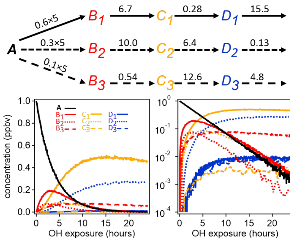
Figure 1 Schematic of reaction pathways with OH (top) of synthetic data and time series shown with linear and log concentration (bottom: left and right, respectively). Arrows represent a reaction with OH. Reaction rate constants with OH are written above the arrows (units are in 10^{-11} \text{ cm}^3 \text{ molecule}^{-3} \text{ s}^{-1} ). Precursor species A reacts at a rate of 5 \times 10^{-11} \text{ cm}^3 \text{ molecule}^{-3} \text{ s}^{-1} with yields of 0.6, 0.3, and 0.1 for the three pathways, respectively. Products of pathways 1, 2, and 3 are drawn with solid, short-dash, and long-dashed lines, respectively, and the first-, second-, and third-generation products are drawn in red, yellow, and blue. The total OH exposure is equal to 24 hours at an average OH concentration of 1.5 \times 10^6 \text{ molecule cm}^{-3} .
