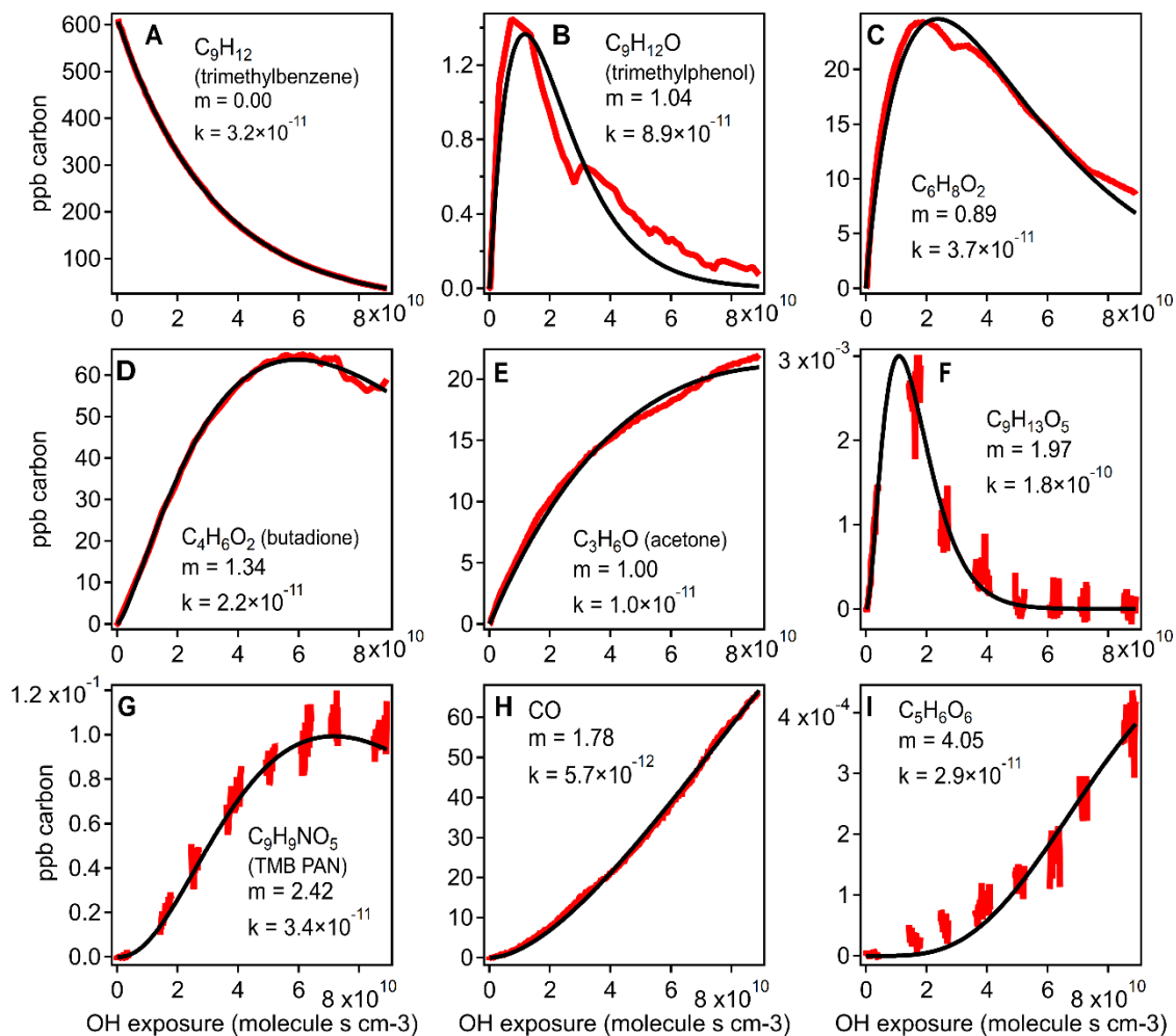
640 Figure 10 Measured species from chamber experiment (red) and GKP best fit (black). Data in panels A, C and E are from Vocus-2R-PTR; in panels B and D from PTR3- \text{H}_3\text{O}^+ , in panels F, G, and I from I - CIMS, and in panel H from TILDAS. The data gaps in panels F, G, and I arise from the I - CIMS instrument measuring particle-phase composition, measurements that are not considered in this work.
