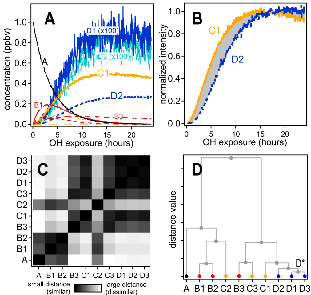
500 Figure 6 Hierarchical clustering procedure applied to synthetic data. First, second, and third-generation species are shown in red, yellow, and blue, respectively, and the precursor is shown in black. A. Time series data. B. Time series of species C1 and D2 normalized between 0 and 1. The gray shaded area is integrated to give the distance between the two time series. C. Matrix showing the relative distance between each pair of species. D. Hierarchical cluster relationship; D1 and D3 are the most similar species, and so are the first to be clustered together (forming a new cluster D*)
