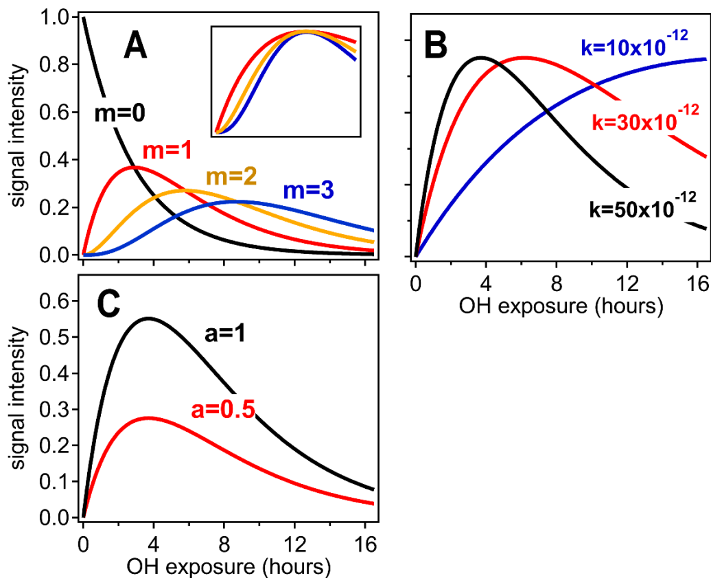
Figure 2 Illustration of the relationships between the different GKP parameters ( m , k , and a ) and the time dependence of a given species, using synthetic data. A. Parameterizations with different generation m . In the subpanel, the traces with m=2 and 385 m=3 have been scaled to allow comparison of the curvature, which differs with generation. B. Parameterizations with different rate constant k . Increasing k does not change the shape of the curve, but causes the maximum to occur at lower OH exposures. C. Parameterizations with different scaling constant a , which changes neither curvature nor location of the maximum, but only the height of the curve.
