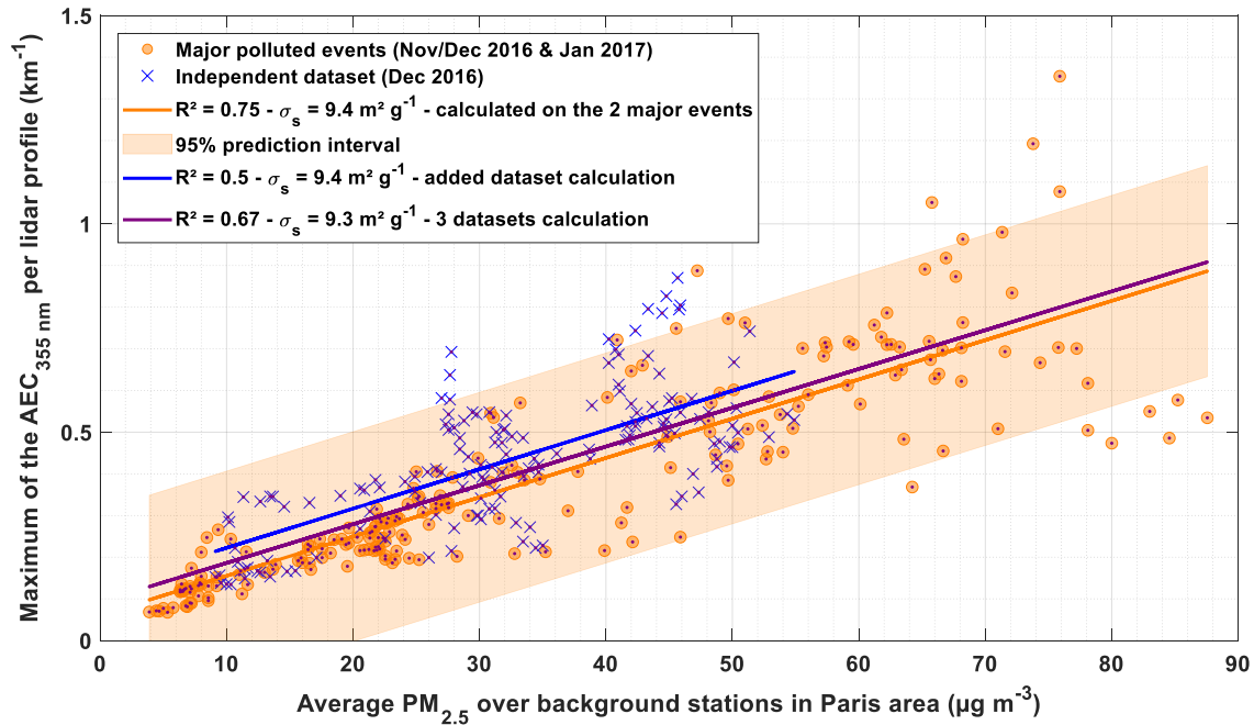
Figure 14: Relationship between \text{PM}_{2.5} (X-axis) and \text{AEC}_{\text{max}} within the PBL (Y-axis). Orange dots are the same dataset presented in Figure 13. Blue crosses are data sampled from the 5 to the 8 December 2016. The orange solid line corresponds to the linear regression computed from the orange points (same as Figure 13) and the light orange area illustrates its 95% confidence interval. The blue solid line is the result of the linear regression calculated on all the points (blue crosses and orange dots). The correlation coefficients can be found in the top left-hand corner.
