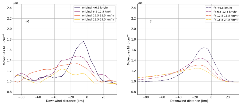
Figure 4. Mean total column cross-sections of the original and reconstructed plume shape for the ZMU fertilizer plant in Kirovo-Chepetsk, Russia. The left plot shows the original CrIS NH 3 total column distribution [2013-2017] as a function of wind speed. The cross-section is a cross-sectional average of the striped black square shown in Fig. 3. The right plot shows the mean cross-section of the reconstructed plume.
