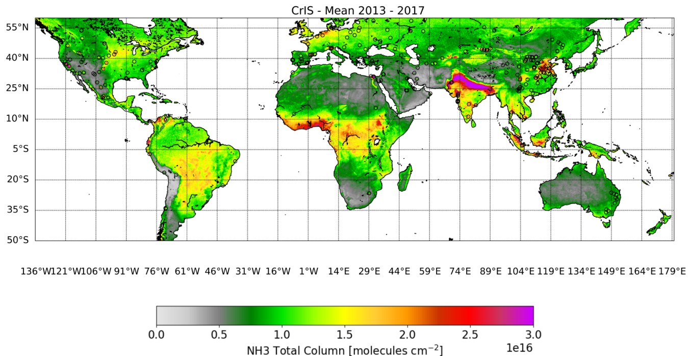
Figure 1. CrIS NH 3 5 year mean [2013-2017] total column [molecules cm -2 ] distribution at 0.05° x 0.05° [longitude, latitude] resolution, with the source locations of successful estimates shown by black circles centered around the source locations.
