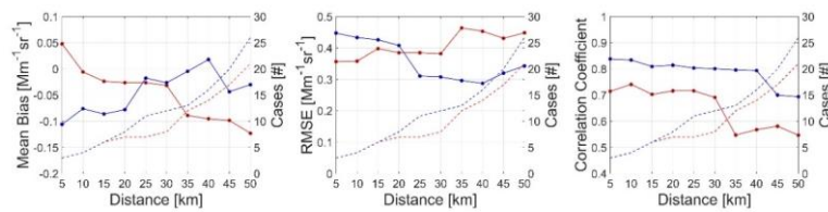
Figure 1: CATS backscatter coefficient at 1064nm with respect to EARLINET ground-based measurements, as a function of distance (km) between the closest CATS Level 2 Aerosol Profile and the respective "collocated" EARLINET station, for daytime (red line) and nighttime (blue line) ISS overpasses. Left: Mean Bias [ \text{Mm}^{-1}\text{sr}^{-1} ], center: RMSE [ \text{Mm}^{-1}\text{sr}^{-1} ] and right: Correlation Coefficient. Dashed lines correspond to the number of CATS-EARLINET correlative cases considered per each upper distance threshold between the CATS footprint and the locations of EARLINET stations.
