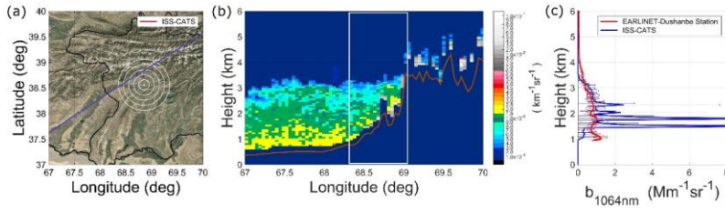
Figure 5: (a) Nighttime ISS orbit over the EARLINET Dushanbe station on the 25 th of May 2015 at 18:53:19 UTC and of closest distance between the footprint of CATS and the EARLINET- Dushanbe station of 24.3km. The white dot denotes the location of Dushanbe lidar system while the blue line shows the lidar footprint of CATS. (b) CATS Backscatter Coefficient at 1064 nm. (c) CATS (blue line) spatially and EARLINET-Dushanbe (red line) temporarily averaged backscatter coefficient profiles (1064 nm). The implemented EARLINET-Dushanbe time window of cloud-free measurements was between 18:00:00 and 20:00:00 UTC. The horizontal blue and red lines denote the variability (one standard deviation) of the CATS and EARLINET measured atmospheric scenes, respectively.
