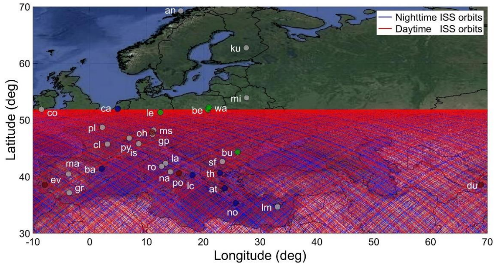
Figure 4: Distribution of EARLINET lidar stations over Europe and West Asia. Green dots: Continental stations used in the inter-comparison. Blue dots: Coastal stations used in the inter-comparison. Brown dots: Mountainous stations used in the inter-comparison. ISS orbits between 02/2015 and 09/2016 are overlaid in red for daytime and in blue for nighttime overpasses.
