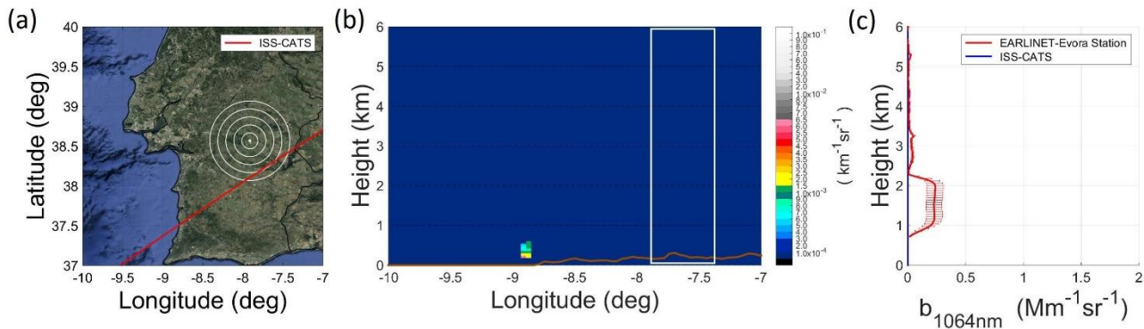
Figure 4: (a) Daytime ISS orbit over the EARLINET Évora station on the 31th of May 2016 at 19:43:31 UTC and of closest distance between the footprint of CATS and the EARLINET- Évora station of 39.42km. The white dot denotes the location of Évora lidar system while the red line shows the lidar footprint of CATS. (b) CATS Backscatter Coefficient at 1064 nm. (c) CATS (blue line) spatially and EARLINET-Évora (red line) temporally averaged backscatter coefficient profiles (1064 nm). The implemented EARLINET-Évora time window of cloud-free measurements was between 19:29:56 and 19:59:35 UTC. The horizontal blue and red lines denote the variability (one standard deviation) of the CATS and EARLINET measured atmospheric scenes, respectively. Figure 4: (a) Daytime ISS orbit over Évora EARLINET station on the 31th of May 2016 (red line). The white circle denotes the location of Évora lidar system, (b) CATS Backscatter Coefficient 1064nm and (c) CATS (blue line) and EARLINET-Évora (red line) backscatter coefficient profiles (1064 nm).
