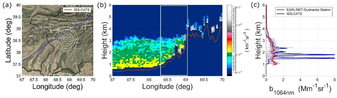
Figure 5: (a) Nighttime ISS orbit over the EARLINET Dushanbe station on the 25 th of May 2015 at 18:53:19 UTC and of closest distance between the footprint of CATS and the EARLINET- Dushanbe station of 24.3km. The white dot denotes the location of Dushanbe lidar system while the blue line shows the lidar footprint of CATS. (b) CATS Backscatter Coefficient at 1064 nm. (c) CATS (blue line) spatially and EARLINET-Dushanbe (red line) temporarily averaged backscatter coefficient profiles (1064 nm). The implemented EARLINET-Dushanbe time window of cloud-free measurements was between 18:00:00 and 20:00:00 UTC. The horizontal blue and red lines denote the variability (one standard deviation) of the CATS and EARLINET measured atmospheric scenes, respectively.
