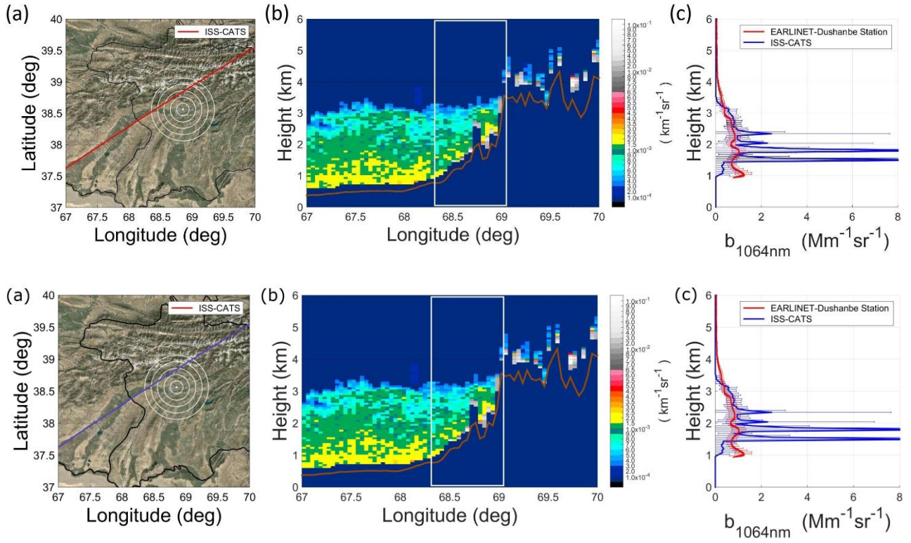
Figure 5: (a) Nighttime ISS orbit over the EARLINET Dushanbe station on the 25th of May 2015 at 18:53:19 UTC and of closest distance between the footprint of CATS and the EARLINET- Dushanbe station of 24.3km. The white dot denotes the location of Dushanbe lidar system while the blue line shows the lidar footprint of CATS. (b) CATS Backscatter Coefficient at 1064 nm. (c) CATS (blue line) spatially and EARLINET-Dushanbe (red line) temporarily averaged backscatter coefficient profiles (1064 nm). The implemented EARLINET-Dushanbe time window of cloud-free measurements was between 18:00:00 and 20:00:00 UTC. The horizontal blue and red lines denote the variability (one standard deviation) of the CATS and EARLINET measured atmospheric scenes, respectively. Figure 5: (a) Nighttime ISS orbit over Dushanbe EARLINET station on the 25th of May 2015 (blue-line). The white circle denotes the location of Dushanbe lidar system, (b) CATS Backscatter Coefficient 1064nm and (c) CATS (blue-line) and EARLINET-Dushanbe (red-line) backscatter coefficient profiles (1064 nm).
