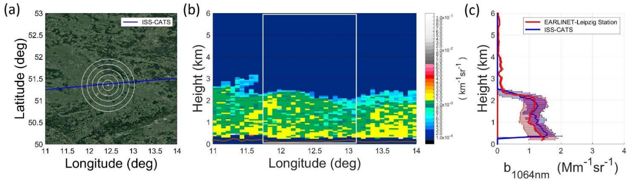
Figure 3: (a) Nighttime ISS orbit over the EARLINET Leipzig station on the 13th of September 2016 at 03:37:49 UTC and of closest distance between the footprint of CATS and the EARLINET- Leipzig station of 3.79km. The white dot denotes the location of Leipzig lidar system while the blue line shows the lidar footprint of CATS. (b) CATS Backscatter Coefficient at 1064 nm. (c) CATS (blue line) spatially and EARLINET-Leipzig (red line) temporally averaged backscatter coefficient profiles (1064 nm). The implemented EARLINET-Leipzig time window of cloud-free measurements was between 00:00:00 and 02:30:00 UTC. The horizontal blue and red lines denote the variability (one standard deviation) of the CATS and EARLINET measured atmospheric scenes, respectively. Figure 3: (a) Nighttime ISS orbit over EARLINET Leipzig station on the 13th of September 2016 (blue line). The white circle denotes the location of Leipzig lidar system, (b) CATS Backscatter Coefficient 1064nm and (c) CATS (blue line) and EARLINET-Leipzig (red line) backscatter coefficient profiles (1064 nm).
