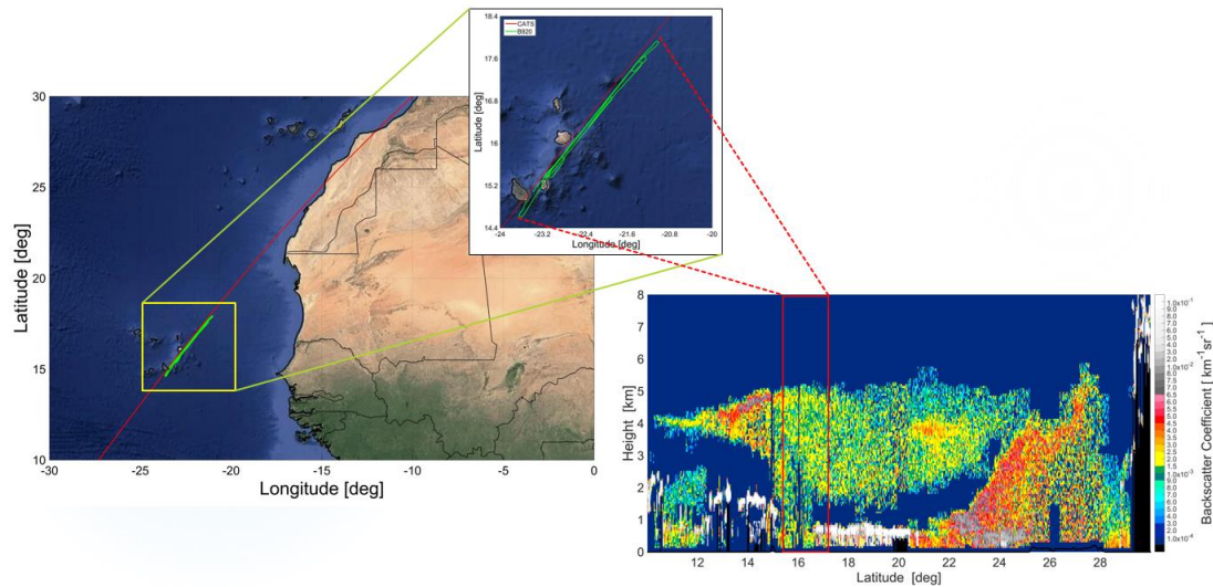
Figure 5: B920 flight on August 7 th , 2015 over Cape Verde, high collocated with ISS-CATS overpass. Left: B920 flight and ISS footprint (left), and CATS backscatter coefficient 1064nm scene (right).
