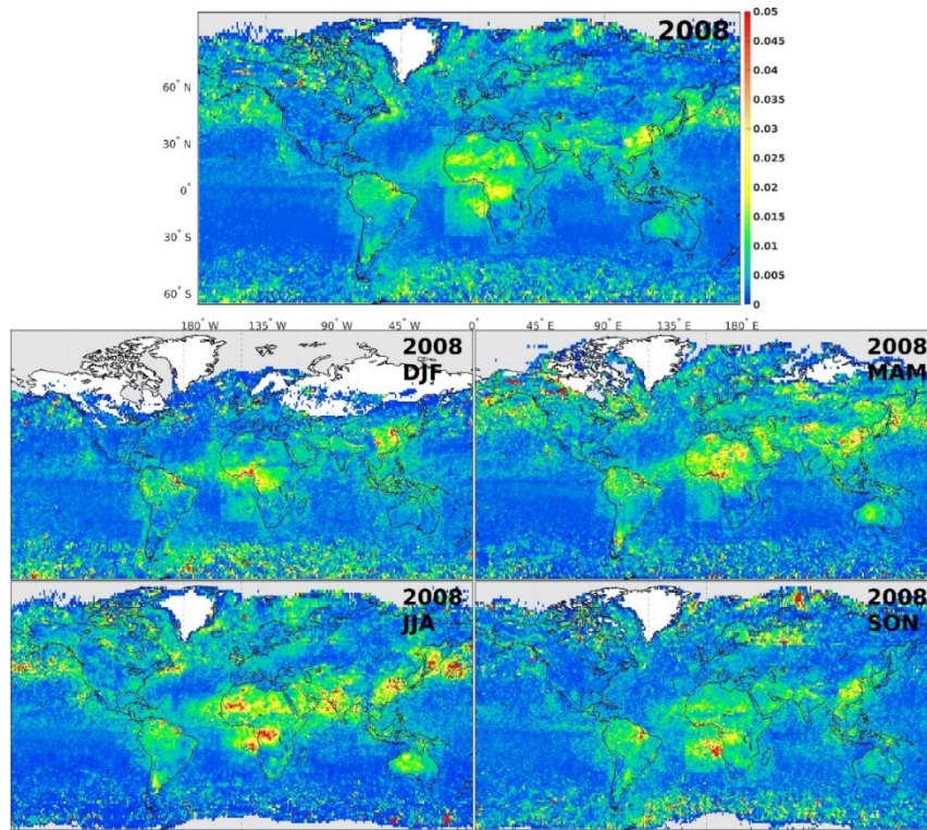
Figure 10. Seasonal and annual structural uncertainties between the L3 merged product (M, approach 2: RM2, "all") and other L3 merged products calculated with the approaches 1 and 2 for year 2008.
