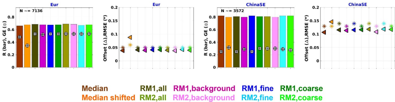
Figure 8. AERONET comparison statistics: correlation coefficient R , bar; fraction of pixels satisfying the GCOS requirements, GE, \oplus ; b, d; Offset, \Delta ; root mean square error RMSE, *; for AOD products merged with different approaches, median, shifted median, RM1, RM2 for different aerosol types for Europe and ChinaSE. For all regions, see Fig. S13.
