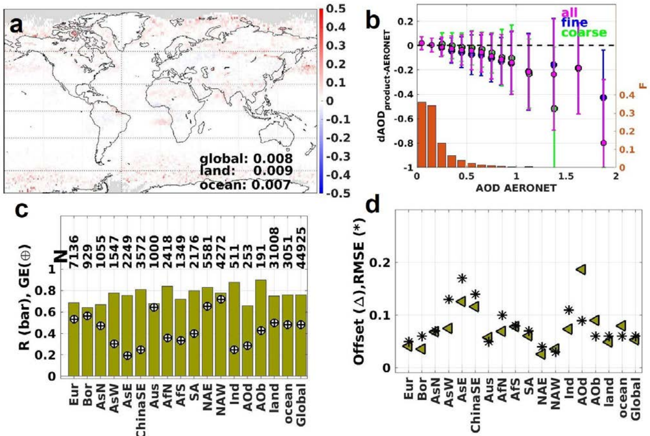
Figure 9. L3 merged (approach 2, RM2, "all") AOD product deviation from the annual median AOD calculated from individual products used for merging (Table 2) for year 2008 (as Fig. S1 for individual products), a; L3 monthly merged AOD product evaluation with AERONET: binned AOD bias for "all" (purple), "background" (AOD<0.2, purple), "fine-dominated" (blue) and "coarse-dominated" (green) aerosol types, b; regional statistics (c: correlation coefficient R, bar; fraction of pixels that fulfil the GCOS requirements, GE, circle; d: Offset, \Delta ; RMSE, *).
