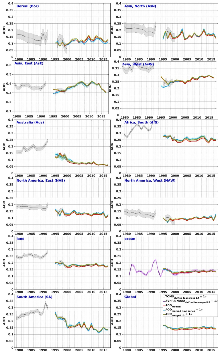
Figure 12. Annual AOD time series merged with two different approaches (red, light blue for approaches 1 and 2, respectively) and AOD time series from the L3 merged data (approach 2, olive) for the selected regions. \pm 1\sigma of the AOD from all uncorrected AOD products is shown as light blue shadow (often small, thus not visible). TOMS over land and AVHRR NOAA over ocean products shifted to the merged time series are also shown (grey and purple dashed lines, respectively), when available.
