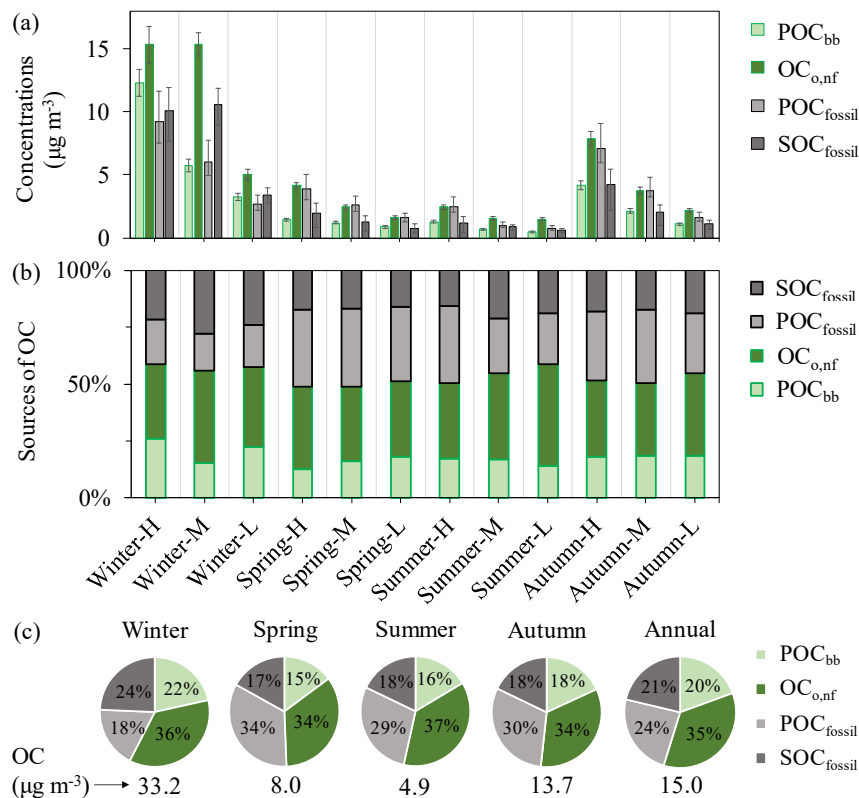
Figure 6. (a) The estimated mass concentrations of POC bb , OC o,nf , POC fossil , SOC fossil ( \mu\text{g m}^{-3} ) in total OC of PM 2.5 samples. The error bars indicate the interquartile range (25th–75th percentile) of the median values. (b) The percentage of POC bb , OC o,nf , POC fossil , SOC fossil in total OC. (c) Average source apportionment results of OC in each season and over the year. The numbers below the pie charts represent the seasonally/annually averaged OC concentrations.
