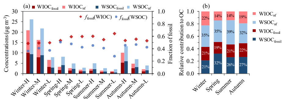
Figure 2. (a) Mass concentrations of WIOC and WSOC from fossil and non-fossil sources ( WIOC_{fossil} , WIOC_{nf} , WSOC_{fossil} and WSOC_{nf} ) as well as fraction of fossil in WIOC and WSOC ( f_{fossil}(WIOC) and f_{fossil}(WSOC) , respectively). (b) Averaged relative contribution to OC (%) from WIOC_{nf} , WSOC_{nf} , WIOC_{fossil} , and WSOC_{fossil} in each season.
