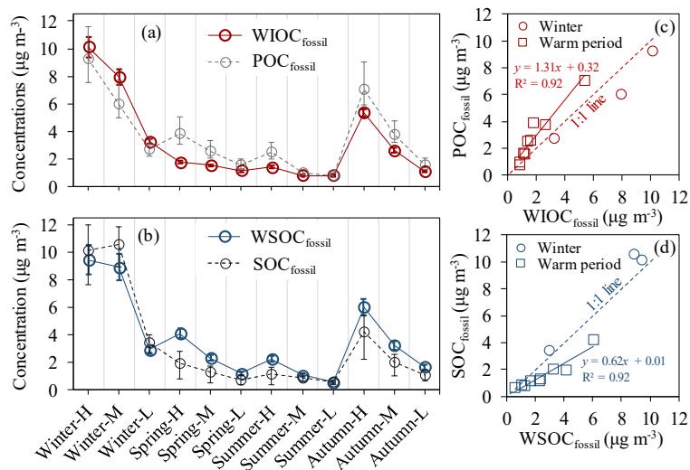
Figure 8. (a) Concentrations of WIOC and POC from fossil sources ( \text{WIOC}_{\text{fossil}} and \text{POC}_{\text{fossil}} , respectively). Panel a has the same x axis with panel b. (b) Concentrations of WSOC and SOC from fossil sources ( \text{WSOC}_{\text{fossil}} and \text{SOC}_{\text{fossil}} , respectively). (c) A scatter plot of \text{WIOC}_{\text{fossil}} concentrations versus \text{POC}_{\text{fossil}} concentrations. (d) A scatter plot of \text{WSOC}_{\text{fossil}} concentrations versus \text{SOC}_{\text{fossil}} concentrations.
