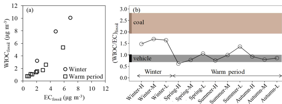
Figure 7. (a) A scatter plot of EC concentrations from fossil sources ( EC_{fossil} ) versus WIOC concentrations from fossil sources ( WIOC_{fossil} ) in winter (circle) and warm period (square). (b) The WIOC to EC ratio from fossil sources ( (WIOC/EC)_{fossil} ) over all the selected samples throughout the year. The dashed areas indicate typical primary OC/EC ratios for coal combustion (brown) and vehicle emissions (black).
