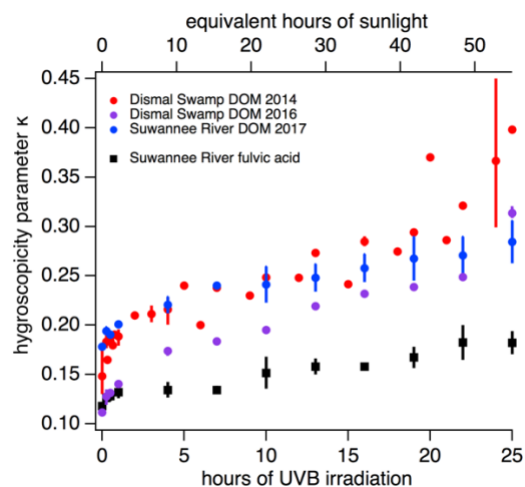
Figure 1. The CCN ability of DOM and of SRFA increases as a function of irradiation. The experimental conditions are equivalent to up to 25 h of UVB exposure (~55 hours of sunlight in the atmosphere). The colors indicate different source material (DS 2014 in red, DS 2016 in purple, SR 2017 in blue and SRFA in black) and the symbols indicate the material was field-collected (circles) or commercially available (squares). The instrumental uncertainty in \kappa = \pm 0.01 . To show the spread of the measurements, the variance from multiple independent experiments are illustrated as bars. The variance was used since not every point had triplicates for standard deviations to be calculated.
