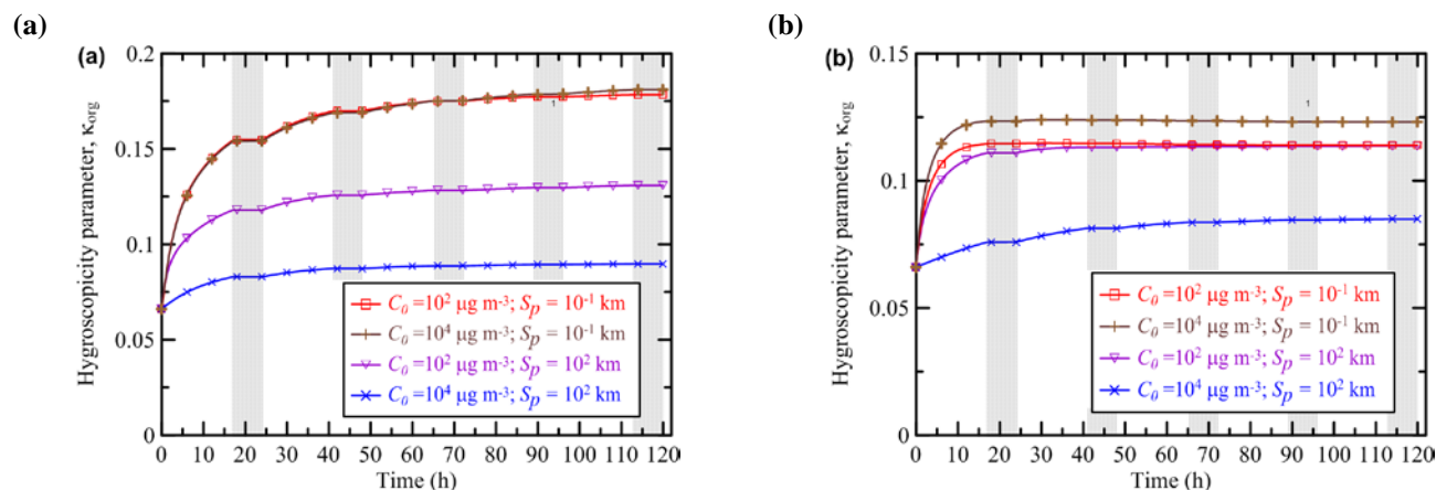
Figure 4: Evolution of the hygroscopicity parameter \kappa simulated as a function of time with different values of the initial BB OA mass concentration, C_0 and the initial BB plume size, S_p , using the (a) T18 and (b) T18f schemes.
