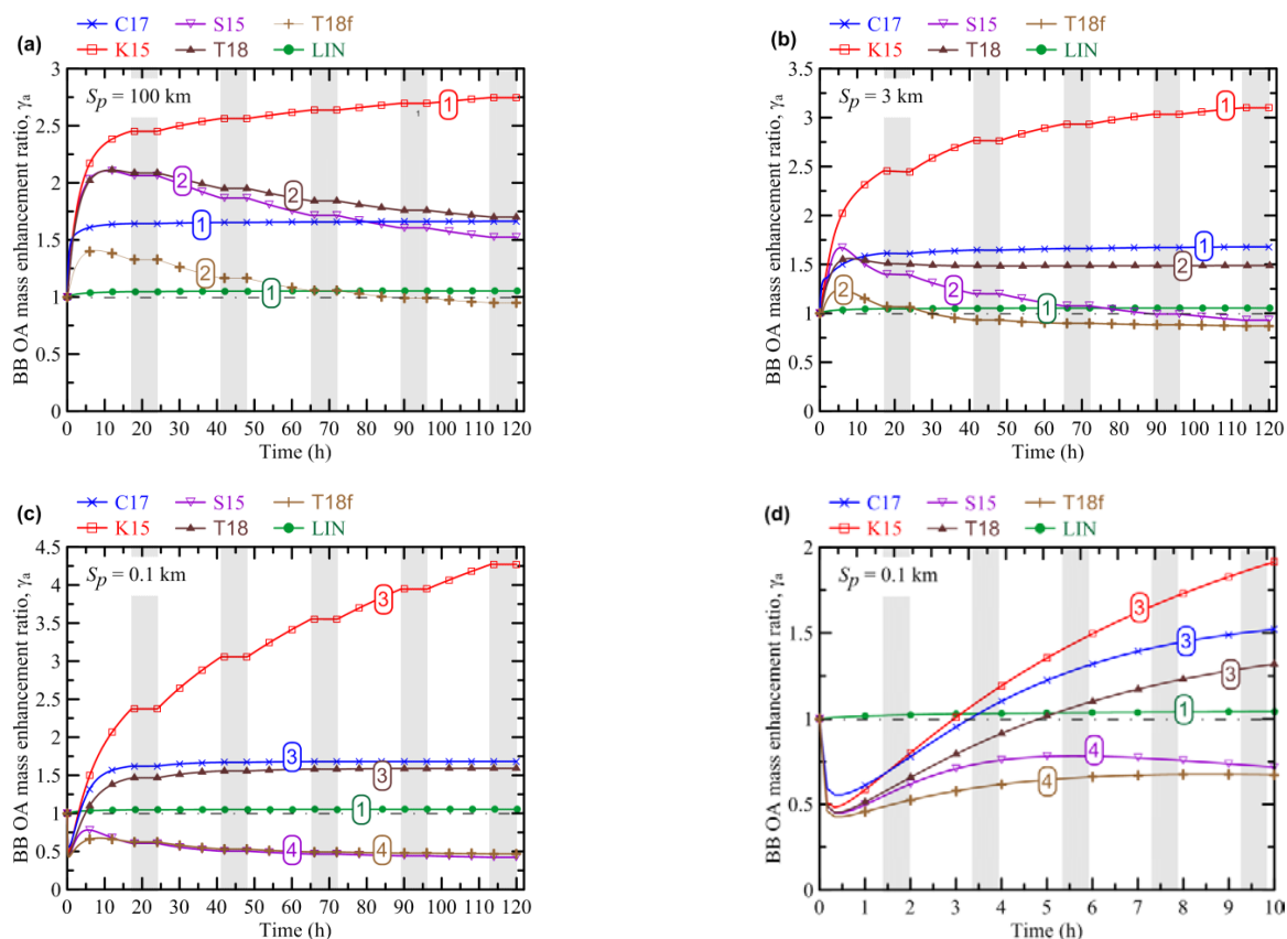
Figure 2: Evolution of the BB OA mass enhancement ratio ( \gamma_a ) according to the simulations performed with the different OA schemes and with different values of the initial plume size: (a) S_p = 100 km, (b) S_p = 3 km, (c, d) S_p = 0.1 km. The initial BB OA concentration, C_0 , was fixed at 10^3 \mu\text{g m}^{-3} in all the simulations. Note that the plot (d) shows a zoomed fragment of the simulations presented in the plot (c). Shaded bands depict nighttime periods when no oxidation reactions were allowed to occur. The numbers on the curves denote the different dynamical regimes of BB OA evolution according to the definitions in Sect. 3.1.
