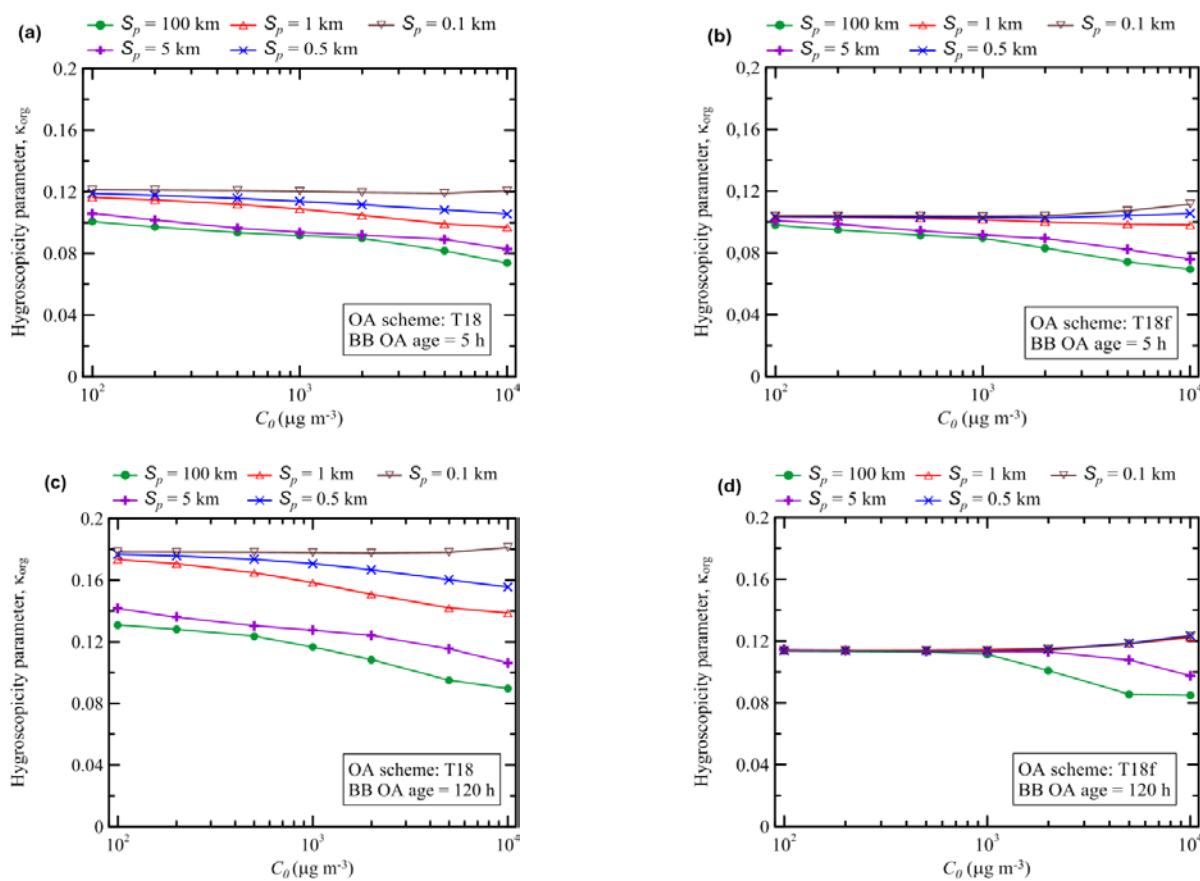
Figure 8: Dependencies of the hygroscopicity parameter, K_{org} , after (a, b) 5 hours and (c, d) 120 hours of BB OA evolution simulated using the (a, c) T18 and (b, d) T18f schemes.
