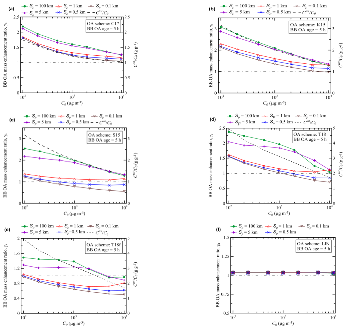
Figure 6: Simulated dependencies of the BB OA enhancement ratio after 5 hours of evolution on the initial BB OA mass concentration, C_0 . The dependencies are obtained with different OA schemes (see Table 1) and with different values of the initial plume size, S_p . Dashed lines show the ratio of the total initial mass concentration of SVOCs ( C^{tot} ) to the initial BB OA concentration ( C_0 ) at thermodynamic equilibrium according to Eq. (18).
