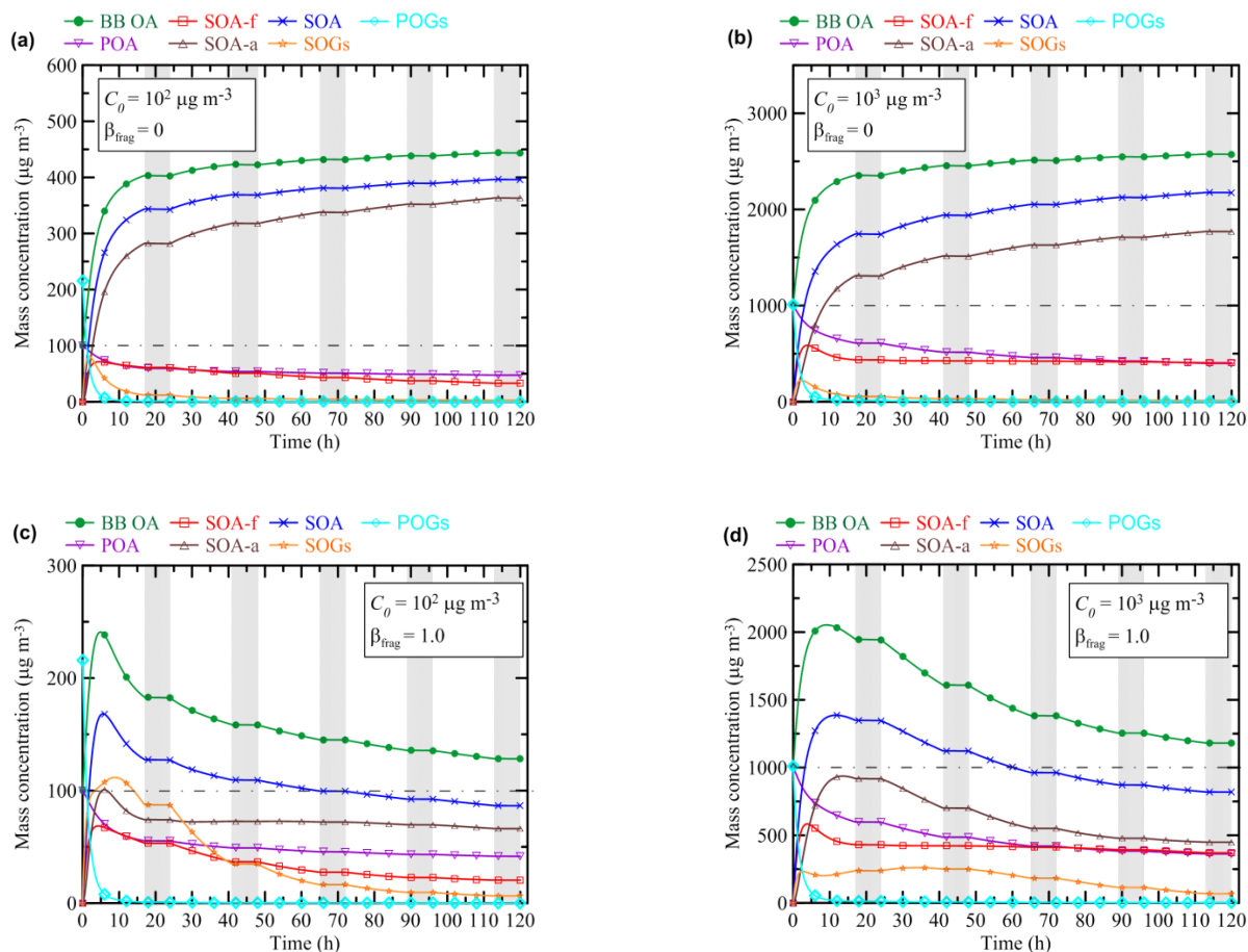
Figure 10: Evolution of the mass concentration of BB OA and its components, including POA, “fresh” SOA (SOA-f), and “aged” SOA (SOA-a) according to the simulations performed with the S15 scheme. Also shown are the total mass concentration of SOA and mass concentrations of POGs and SOGs. The simulations were done with two different values of \beta_{\text{frag}} : (a, b) \beta_{\text{frag}} = 0 , (c, d) \beta_{\text{frag}} = 1 and two different values of C_0 : (a, c) C_0 = 10^2 \mu\text{g m}^{-3} , (b, d) C_0 = 10^3 \mu\text{g m}^{-3} . The initial plume size was set at 100 km in all the simulations.
