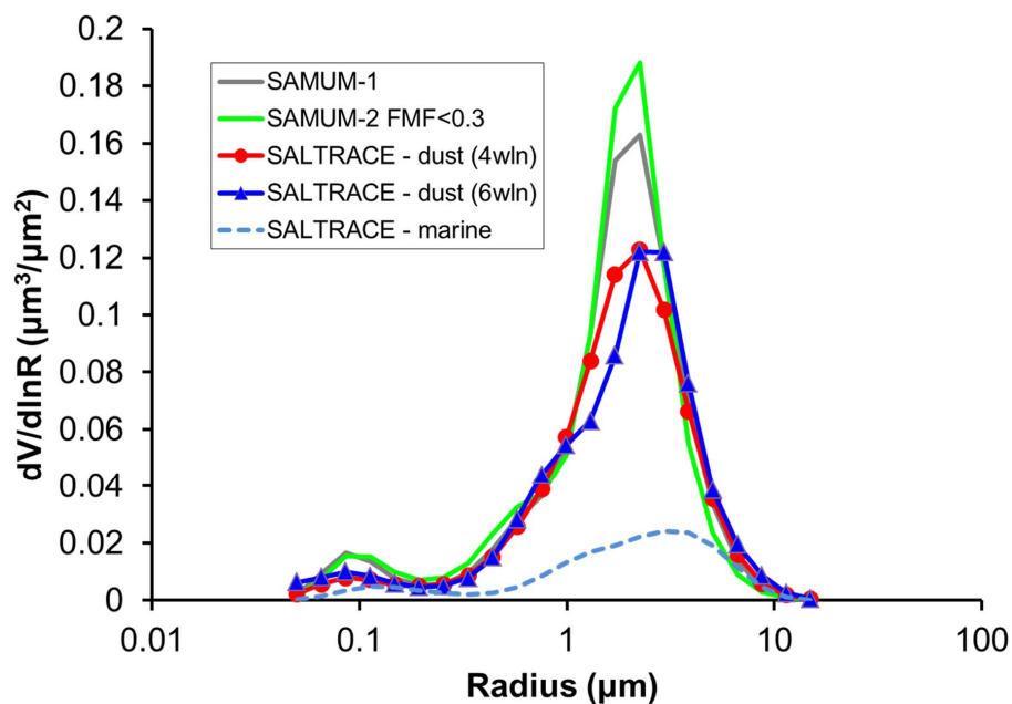
Figure 5. Volume particle size distributions ( dV/d\ln R ) for SALTRACE as well as SAMUM campaigns. Average values for dust cases in each campaign are provided, based on inversion of Cimel sun photometer data . For SAMUM-2 only cases with low fine mode fractions (FMF) between 0.16 and 0.30 are considered.
