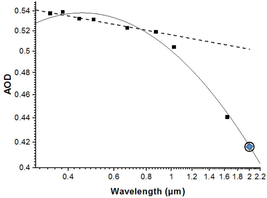
Figure 2. Aerosol optical depth as a function of wavelength in log-log scale for 26 11 June 2013 at 11:12UTC. Solid line indicates the 2nd order fit over the range 340-1640nm whereas the dashed line indicates the 1st order fit over the range 440-870nm, corresponding to the Ångström formula (Ångström, 1961). The extrapolated value of AOD at 2μm wavelength using the 2nd order fit is indicated with a circle.
