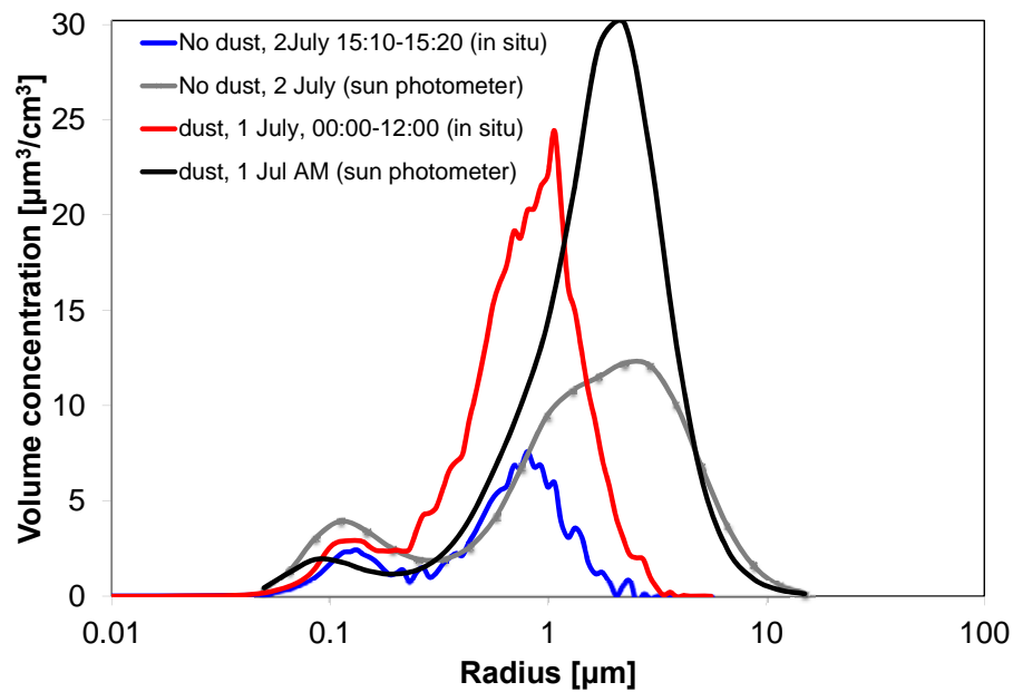
Figure 8. Volume particle size distributions for 1st July 2013 (dust case) and 2nd July 2013 (no-dust case) measured in-situ (left-axis) and by inversion of sun photometer data. The latter have been converted to concentration using a scale height derived from the co-located lidar observations (right-axis see details in the text).
