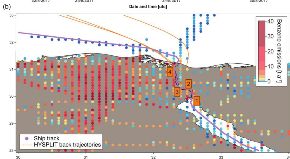
Figure 5: (a) C_3 carbonyls/propane ratio, C_5 carbonyls/pentane ratio, toluene/benzene ratio, relative humidity, solar irradiation, wind direction, speciated and measured OH reactivity in the Suez Canal. Error bars of total OH reactivity display the total uncertainty of the measurement. (b) Ship track of the cruise in the Suez Canal with HYSPLIT air mass back trajectories and numbered labels of case study points. Benzene emissions as an indicator for anthropogenic sources from the EDGAR database ( http://edgar.jrc.ec.europa.eu , for 2012) are shown on a logarithmic colour scale.
