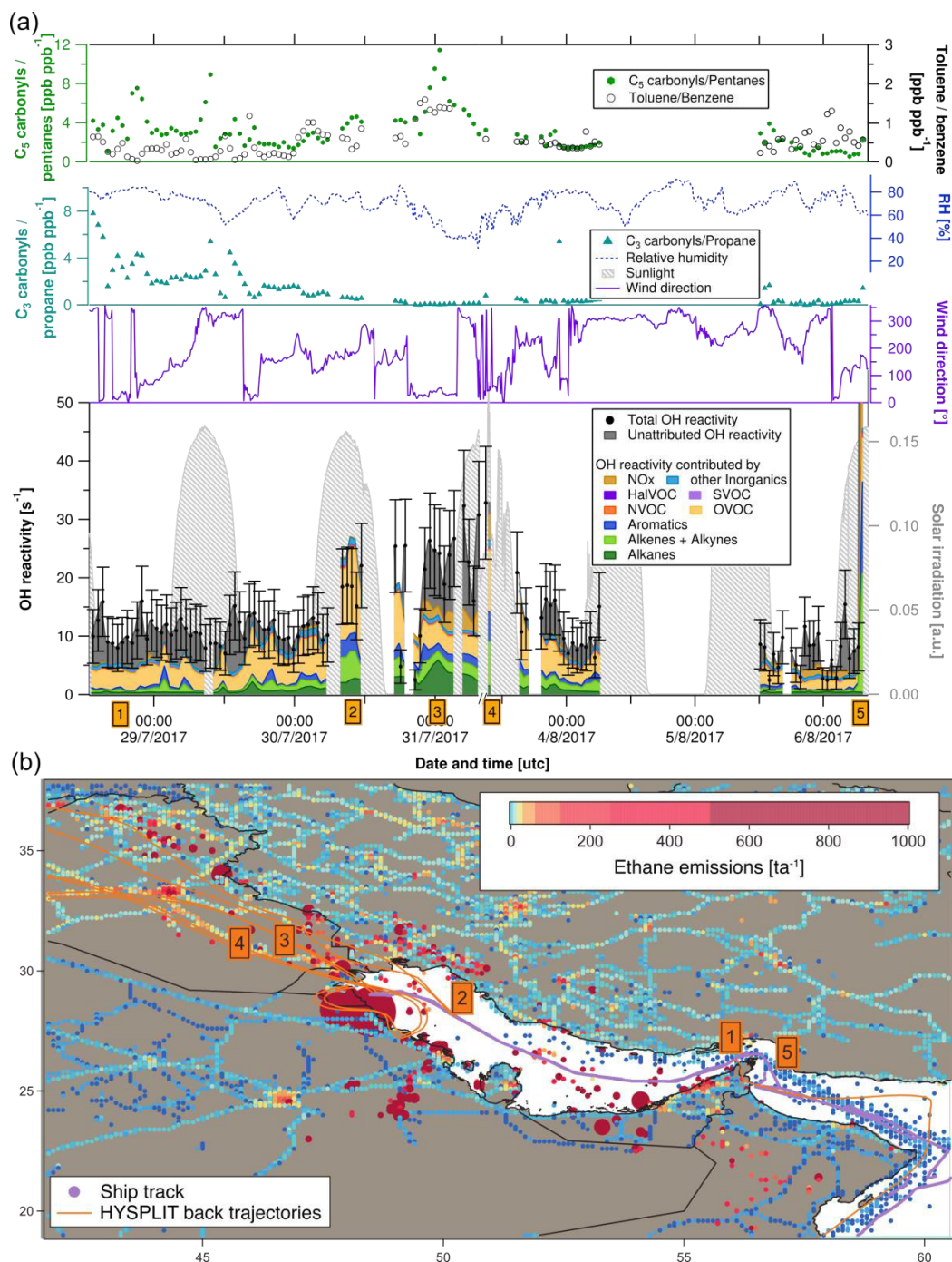
Figure 4: (a) C_3 carbonyls/propane ratio, C_5 carbonyls/pentane ratio, toluene/benzene ratio, relative humidity, solar irradiation, wind direction, speciated and measured OH reactivity in the Arabian Gulf. Error bars of total OH reactivity display the 1\sigma total uncertainty of the measurement. (b) Ship track of the campaign in the Arabian Gulf with HYSPLIT air mass back trajectories and numbered labels of case study points. Ethane emissions from the EDGAR database ( http://edgar.irc.ec.europa.eu , for 2012) as an indicator for petroleum extraction/processing and other anthropogenic sources are shown on a logarithmic colour scale. Emissions out of scale ( > 1000 \text{ t a}^{-1} ) are shown with larger circles.
