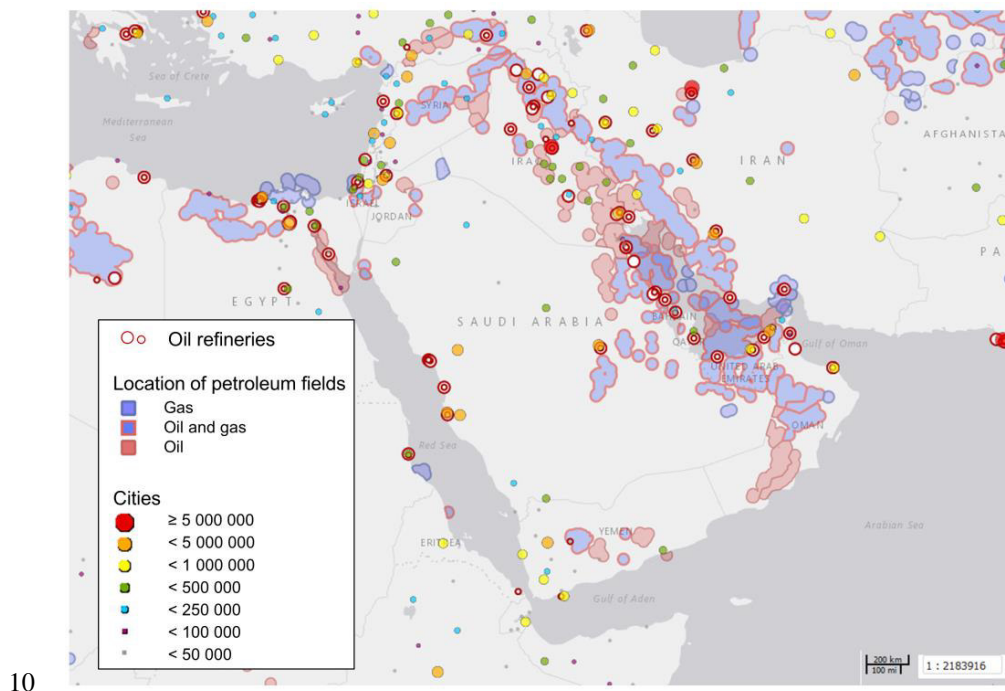
Figure 2: Oil refineries, petroleum fields and cities in the Arabian Basin. City markers are scaled with the number of inhabitants as denoted in the legend. Source: Harvard WorldMap Project ( https://worldmap.harvard.edu/maps/6718/dJT ).
