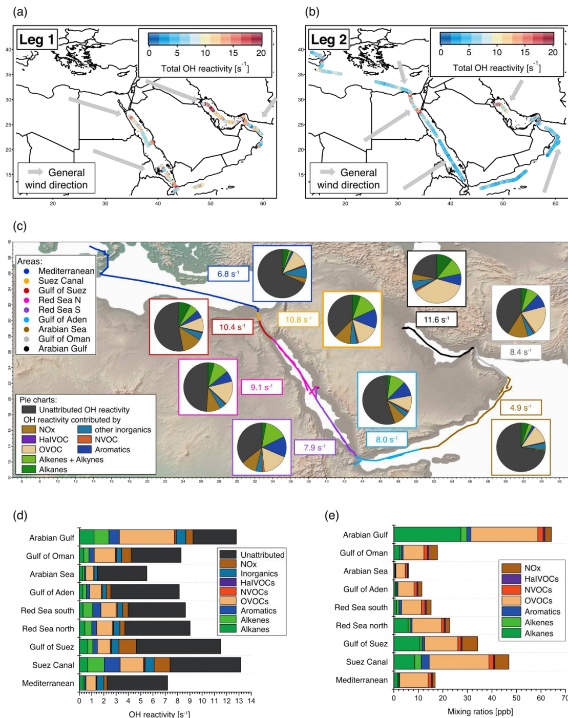
Figure 1: Overview of total OH reactivity around the Arabian Peninsula during the AQABA campaign. OH reactivity during (a) leg 1 (July 5–July 31, 2017) and (b) leg 2 (August 3–August 31, 2017). The maximum in the color scales is set to 20 s -1 for better visibility of differences, although there are a few datapoints above this value. Arrows depict general wind directions for the respective regions. (c) Total OH reactivity medians by region, and pie charts showing the contribution of compound classes for
