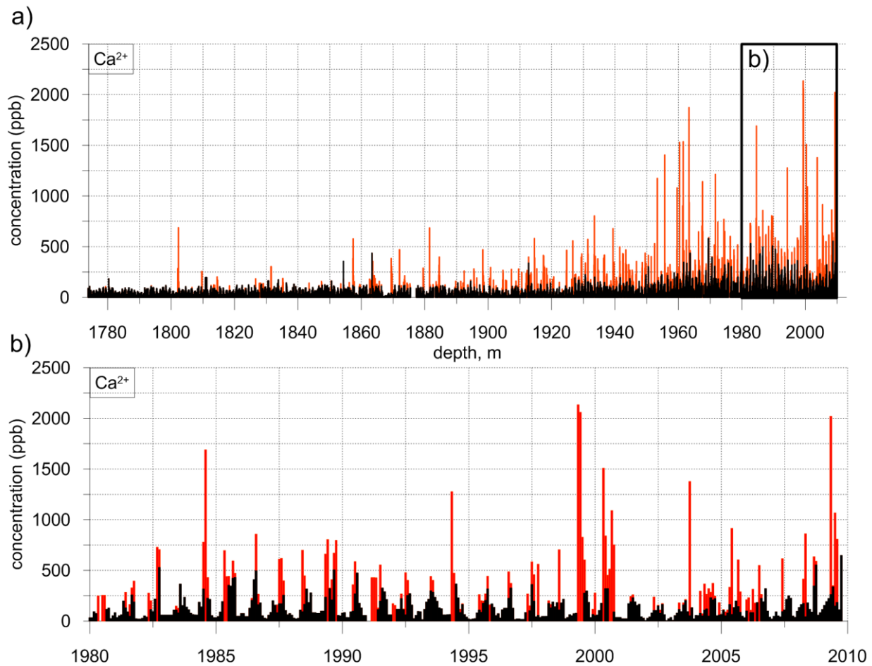
5 Figure 4: (a): Total (red) and background (black) \text{Ca}^{2+} concentrations (ppb) in Elbrus ice core samples. The full record (a) and the upper section of the ice core (b) are shown. Note: background concentration values reflect removal of samples which were found to have been influenced by large dust deposition events.
