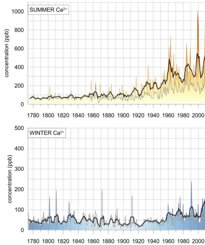
Figure 6: Total and background (grey lines) Ca 2+ concentrations in Elbrus ice core during summer and winter. Five-year moving averages are shown as black lines.
