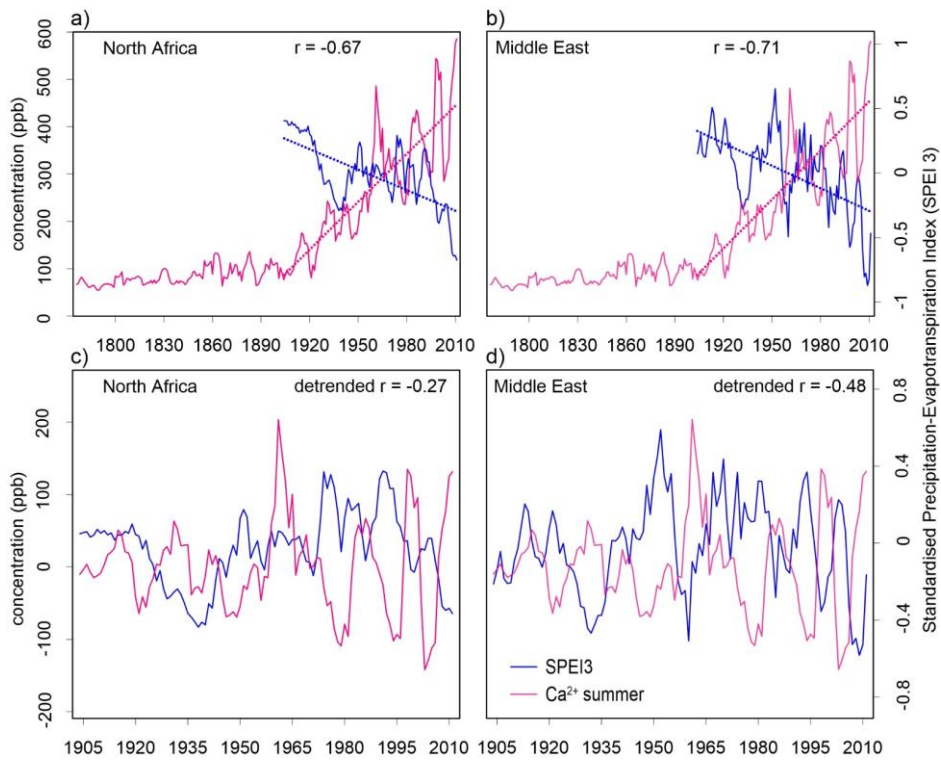
5 Figure 11: \text{Ca}^{2+} and Standardised Precipitation-Evapotranspiration Index (SPEI3) averaged over the regions of (a), (c) North Africa (20-35°N; 0-35°E; and (b), (d) the Middle East (32-37°N; 38-45°E). Outlines of the regions are presented on Figure 10. Detrended records are shown at the bottom graphs.
