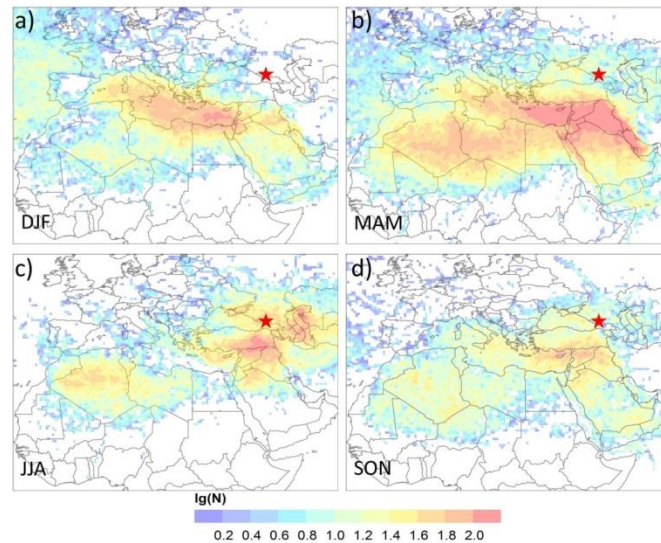
Figure 3: NOAA HYSPLIT_4 10-day backward trajectories density plots for the period 1948-2013 for December – February (a), March-May (b) June-August (c) and September – November (d) using NCEP/NCAR Reanalysis. Trajectories were run every 6 hrs. Only backward trajectories within the boundary layer were considered..
