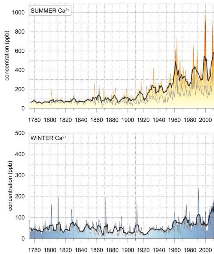
Figure 6: Total and background (grey lines) \text{Ca}^{2+} concentrations in Elbrus ice core in summer and winter. 5-year moving averages are shown as black lines.
