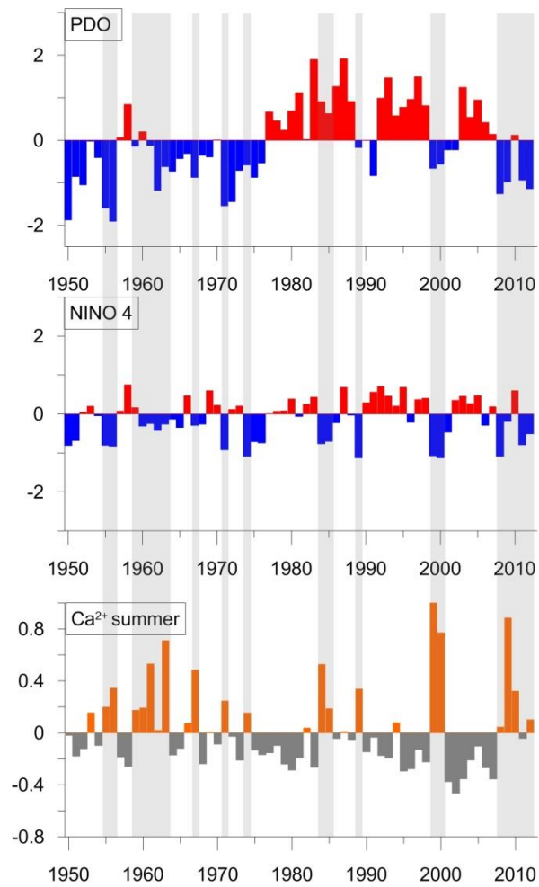
Figure 12: PDO (a) and Niño 4 (b) indices (December-June average), and normalized Ca 2+ record (c). Grey shading indicate years when high dust concentrations coincided with negative Niño 4 phases.
