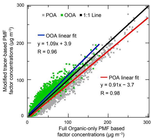
Figure 8. This figure shows the comparison of the modified tracer-based OOA and POA concentrations with those obtained from organic-only PMF. The strong linear correlation and slope close to 1 point to the usefulness of the tracer approach for real-time source apportionment.
