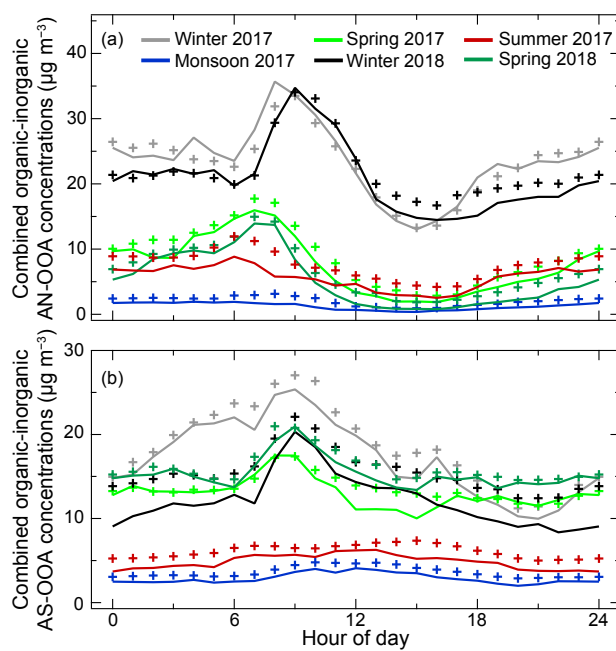
Figure 6. Seasonally representative diurnal mean (+) and median (lines) concentrations of (a) AN-OOA (b) AS-OOA from organic-inorganic combined PMF analysis. Compared to AN-OOA, AS-OOA concentrations remain relatively stable throughout the day, particularly in warmer months.
