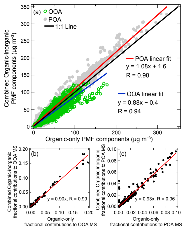
Figure 3. a) Time series correlation of POA and OOA from organic-inorganic PMF and organic-only PMF analysis ( \mu\text{g m}^{-3} ) b) and c) Mass spectral correlations of OOA and POA from organic-inorganic PMF and organic-only PMF analysis. Strong correlations suggest an agreement between the analysis.
