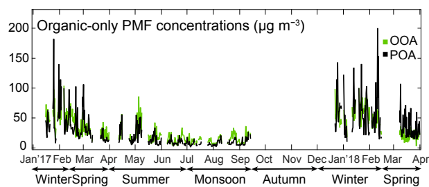
Figure 2. The 12 h averaged concentration time series (TS) of organic-only PMF oxidized organic aerosol (OOA) factor and primary organic aerosol (POA) factor ( \mu\text{g m}^{-3} ). Factor concentrations show strong seasonal and diurnal variations.
