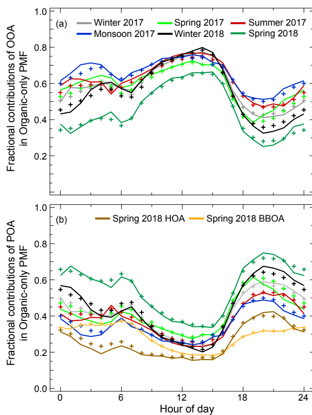
Figure 7. a) Diurnal mean (+) and median (lines) fraction of OOA from organic-only PMF analysis in different seasons. Fractional contributions vary between 32–80%, except spring 2018. This is likely due to the separation of BBOA mixed into the oxidized organics in other seasons. b) Diurnal mean and median composition of POA from organic-only PMF analysis. Spring 2018 has a relatively higher POA fraction, due to the unmixing of a separate BBOA profile.
