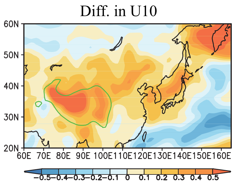
Figure 11. Spatial distribution of the MAM composite difference between the strongest and weakest TPSH years (strongest–weakest) for the model in 10-m wind speed ( U_{10} , \text{m s}^{-1} ). The green-contour area indicates the plateau above 2500 m.
