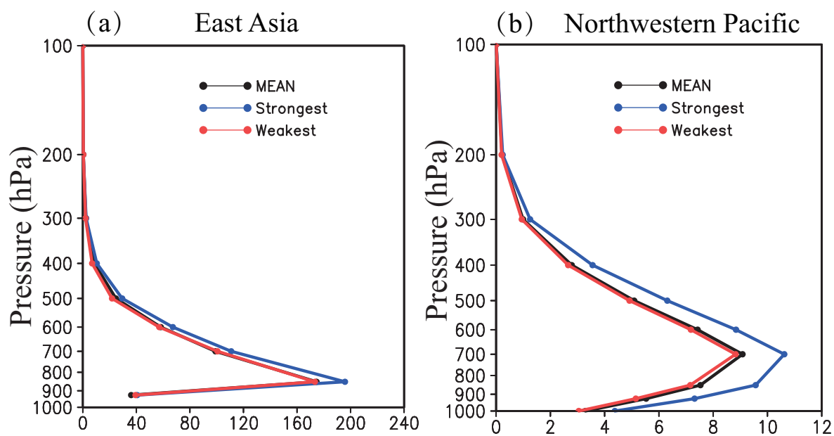
Figure 5. Simulated vertical profile of the MAM dust concentration ( \mu\text{g kg}^{-1} ) from the model for the mean, strongest and weakest years (a) over East Asian dust source area and (b) over the northwestern Pacific.
