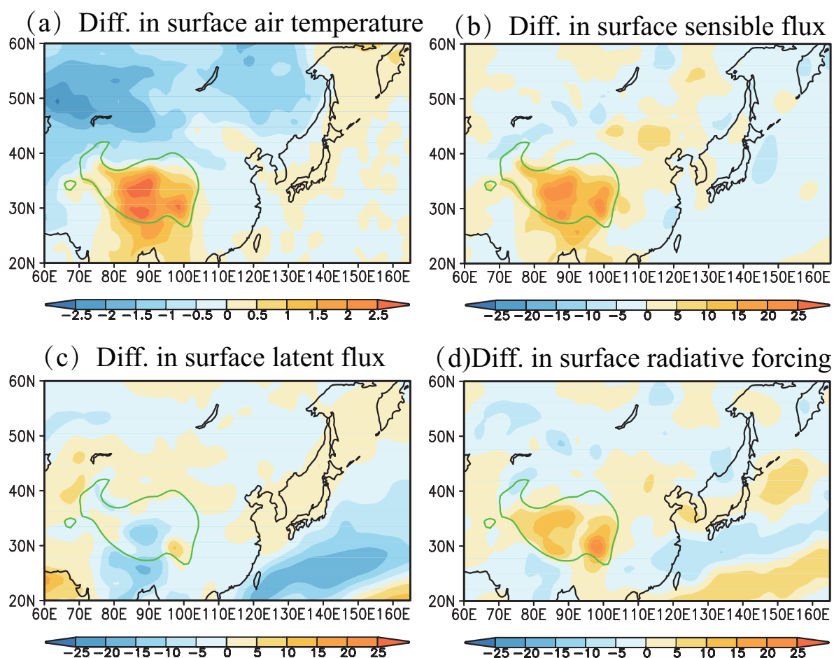
Figure 7. Spatial distribution of the MAM composite difference between the strongest and weakest TPSH years (strongest–weakest) for the model in (a) the surface air temperature (°C), (b) the surface sensible heat (W m -2 ), (c) the surface latent heat (W m -2 ), and (d) the surface radiative forcing (W m -2 ). The green-contour area indicates the plateau above 2500 m.
