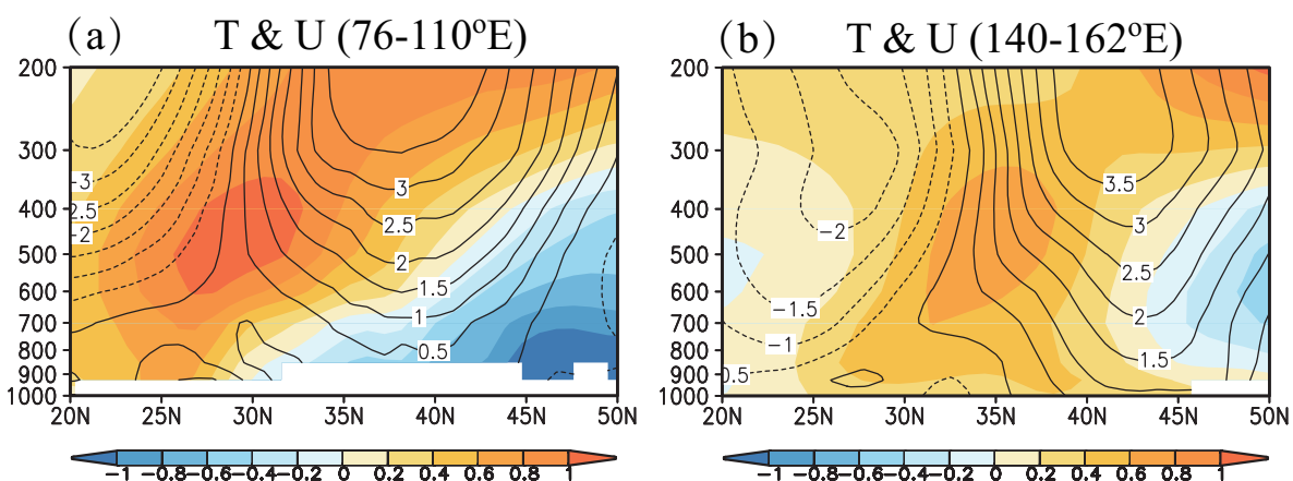
Figure 10. Height-latitude cross-section of the MAM composite difference between the strongest and weakest TPSH years (strongest–weakest) for the model in atmospheric temperature (shaded, °C) and zonal winds (contoured, m s -1 ) along (a) 76–110° E and (b) 140–162° E.
