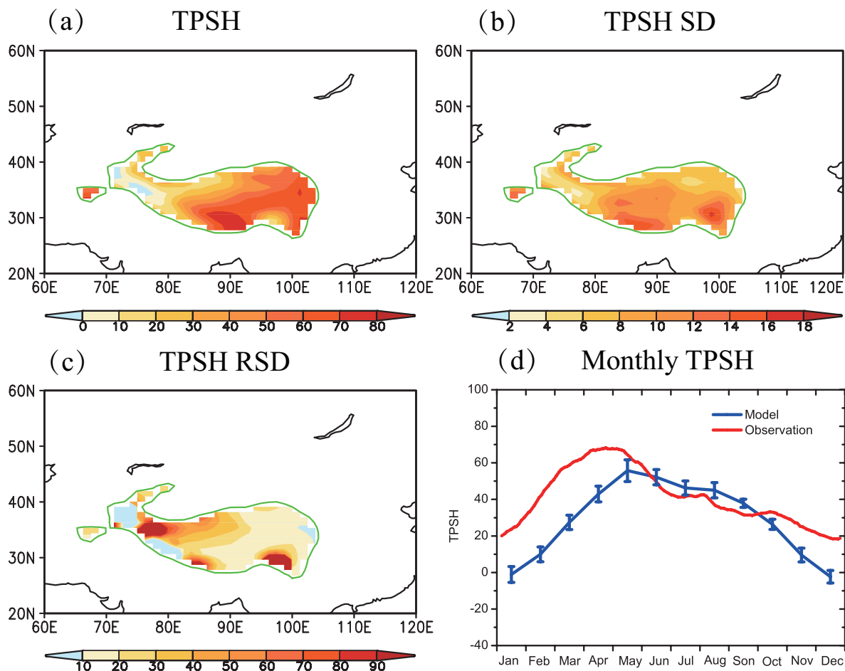
Figure 1. Spatial distribution of (a) the MAM mean sensible heat over the TP (TPSH, W m^{-2} ), (b) the standard deviation of TPSH (SD, W m^{-2} ), and the relative standard deviation of TPSH (RSD, %) in MAM calculated for 30 model years. (d) Annual cycle of TPSH from the model averaged over the TP region above 2500m and the observations averaged over the 73 stations over the TP (Duan et al., 2017). Note that the error bars (d) represent the standard deviation of the simulated TPSH for 30 model years. The green-contour area indicates the plateau above 2500 m.
