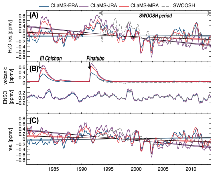
Figure 9. Comparison of residual variability after removing the AC, QBO and SAH from H_2O entry values (mean H_2O mixing ratios on \theta = 400 K averaged over 20°S-20°N) based on CLaMS simulations and SWOOSH. Panel A shows the residual term ( \chi_{res} ) after applying a 3-month running mean. The long-term linear fit is plotted as a solid line with \pm 2\sigma uncertainties. Panel B shows additional components of the multiple linear regression, including the influences of variations in volcanic aerosol (upper set of lines) and ENSO (lower set of lines). Panel C shows the residuum of A after subtracting all contributors shown in B, along with the corresponding trend.
