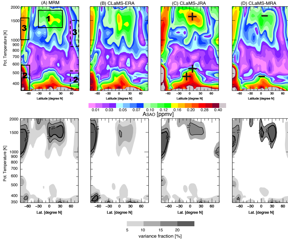
Figure C1. The top row shows SAH amplitudes in the same way as in the second row of Figure 7. The bottom row shows the fraction of SAH variance relative to total variance, similar to the bottom row of Figure 9.
