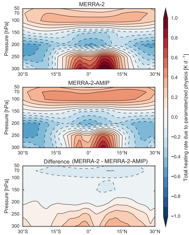
Figure D1. Comparison of time-mean zonal-mean diabatic heating rates in the tropical (30°N-30°S) lower stratosphere between the MERRA-2 reanalysis (top panel) and the MERRA-2 AMIP ensemble mean (middle panel) over 1980–2017. Differences between MERRA-2 and MERRA-2 AMIP are shown in the bottom panel.
