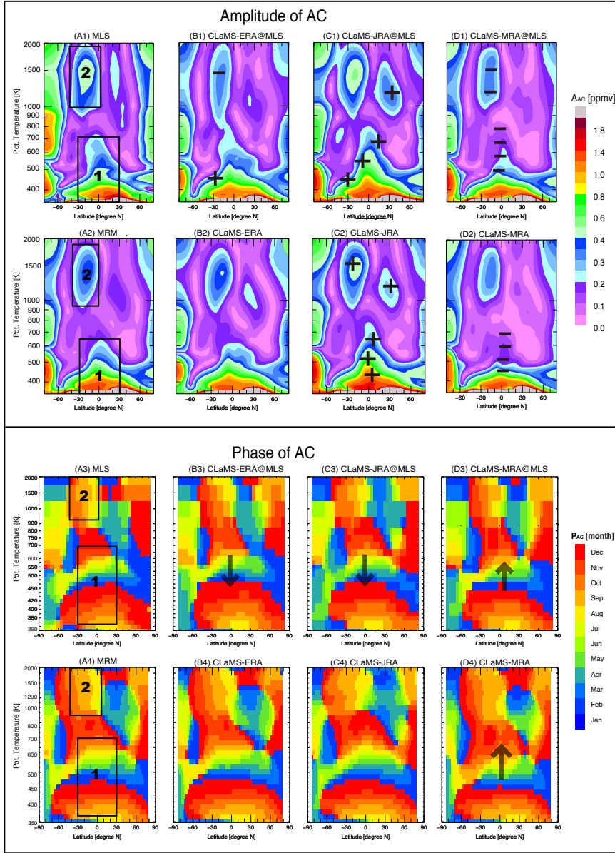
Figure 7. AC amplitudes ( A_{AC} ) and corresponding phases ( P_{AC} ) during the MLS period ( \sim 2005-2013 , the first and third row) and the entire CLaMS period (1980-2013, the second and fourth row). The leftmost panels show A_{AC} and P_{AC} based on Aura MLS observations (A1,A3) and the mean of the three reanalysis-driven models (MRM, A2 and A4). The corresponding A_{AC} values from CLaMS-ERA, CLaMS-JRA and CLaMS-MRA are shown in the rightmost three panels of each row. Overprinted ‘+’ and ‘-’ in panels (B1)-(D1) and (B2)-(D2) demonstrate major differences by more than \pm 30\% in simulated A_{AC} relative to the benchmark estimate shown in the corresponding leftmost panel. Arrows in panels (B3)-(D3) and (B4)-(D4) indicate the major region with phase differences by more than 1 month against the benchmark estimate of P_{AC} shown in the corresponding leftmost panel. The upward arrows show phase lagging behind of the benchmark phase while the downward arrows show phase ahead of the benchmark phase.
