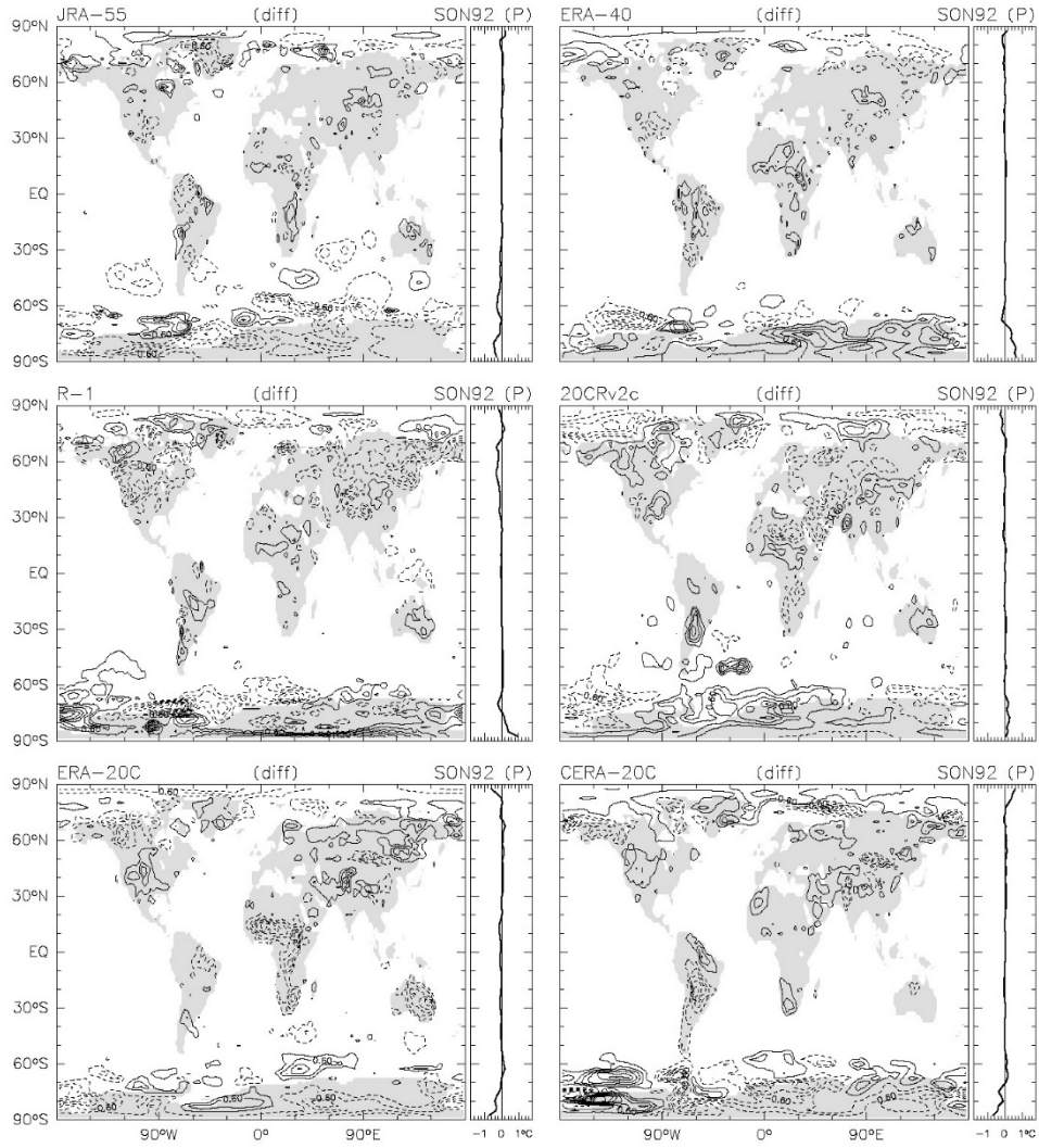
Figure R6. Geographical and zonal-mean distributions of the difference from the REM (shown in Figure R5) for each of the 6 reanalysis data sets shown in Figure 6.
