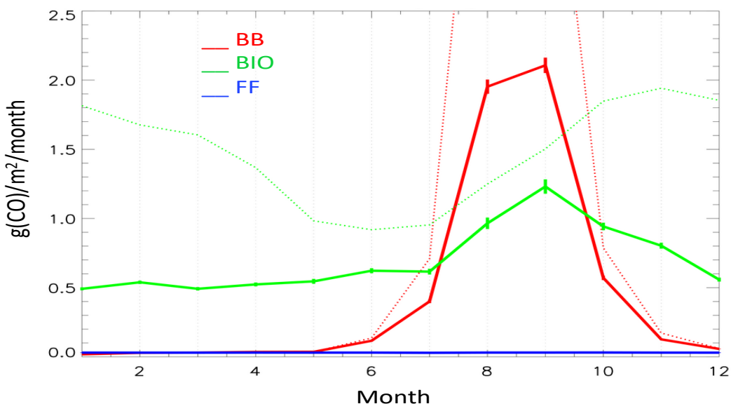
Figure S8. A posteriori (solid lines) and a priori (dotted lines) CO fluxes averaged for each month over 2005-2012 for the S. American tropical Andes piedmont (Fig. S7) region for biomass burning (BB, red), biogenic (BIO, green) and fossil fuel (FF, blue) sectors. Errors on the 8-yr average fluxes for this region are indicated for each sector and month, with values around 3.1% for BIO, 2.7% for BB and 5.7% for FF.
