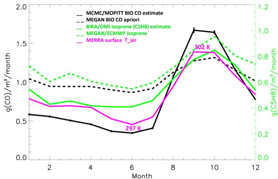
Figure S6. Average monthly CO (black) and C5H8 (green) fluxes and surface air temperatures (magenta, with minimum and maximum values indicated) for 2005-2012 for the S. America Amazon region (Fig. S4). Solid black and green lines show the posterior "top-down" fluxes while dashed black and green lines show the emissions predicted by MEGAN with associated meteorological fields.
