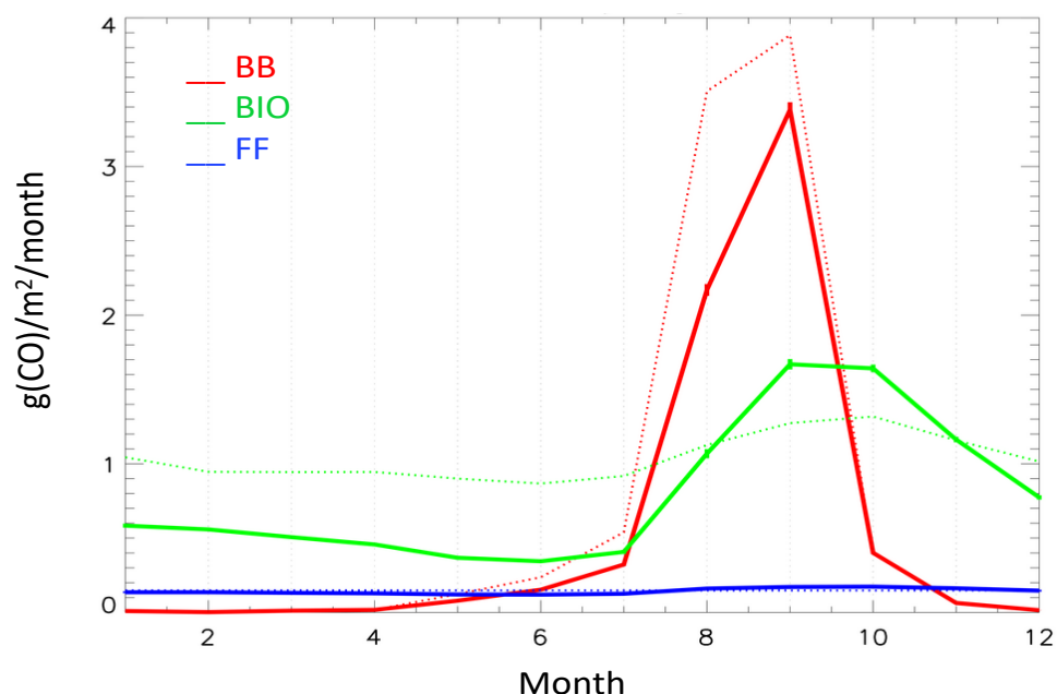
Figure S5. A posteriori (solid lines) and a priori (dotted lines) CO fluxes averaged for each month over 2005-2012 for the S. American Amazon (Fig. S4) region for biomass burning (BB, red), biogenic (BG, green) and fossil fuel (FF, blue) sectors. Errors on the 8-yr average fluxes for this region are indicated for each sector and month, with values around 2.2% for BIO, 1.7% for BB and 4.2% for FF.
