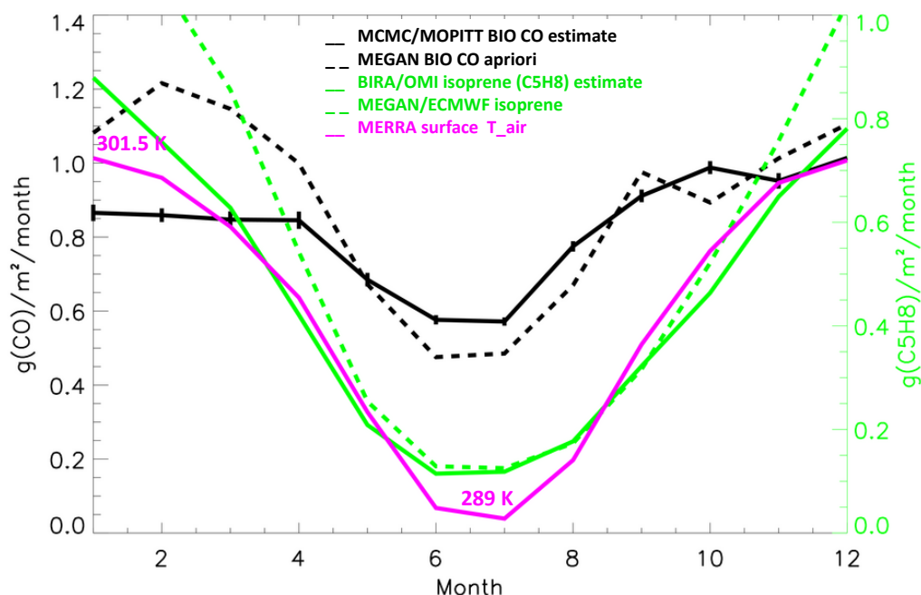
Figure S12. Average monthly CO (black) and C5H8 (green) fluxes and surface air temperatures (magenta, with minimum and maximum values indicated) for 2005-2012 for the Australian tropics and subtropics region (Fig. S10). Solid black and green lines show the posterior “top-down” fluxes while dashed black and green lines show the emissions predicted by MEGAN with associated meteorological fields.
