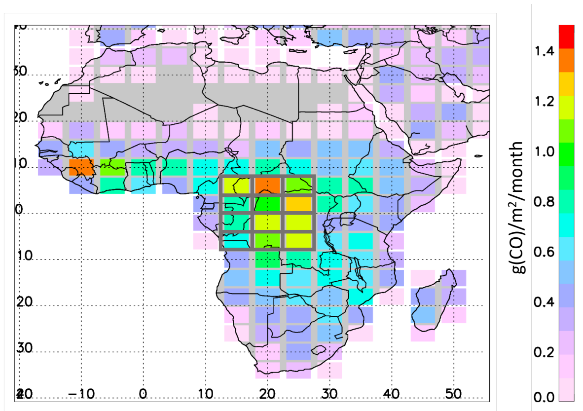
Figure S1. Map of a posteriori biogenic CO fluxes. Grey boxes indicate the Equatorial Africa region used for the 2005-2012 average computed for each month.
