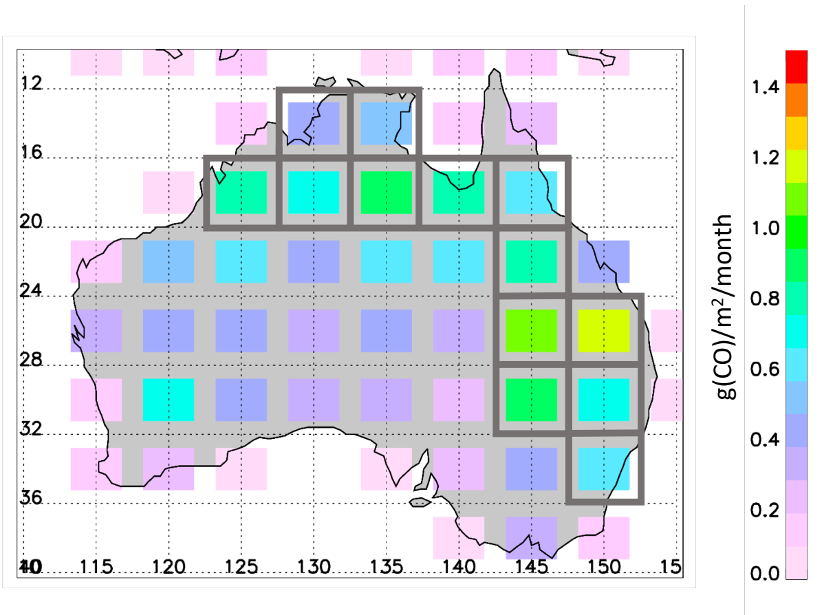
Figure S10. Map of a posteriori biogenic CO fluxes. Grey boxes indicate the Australian regions used for the 2005-2012 average computed for each month.
