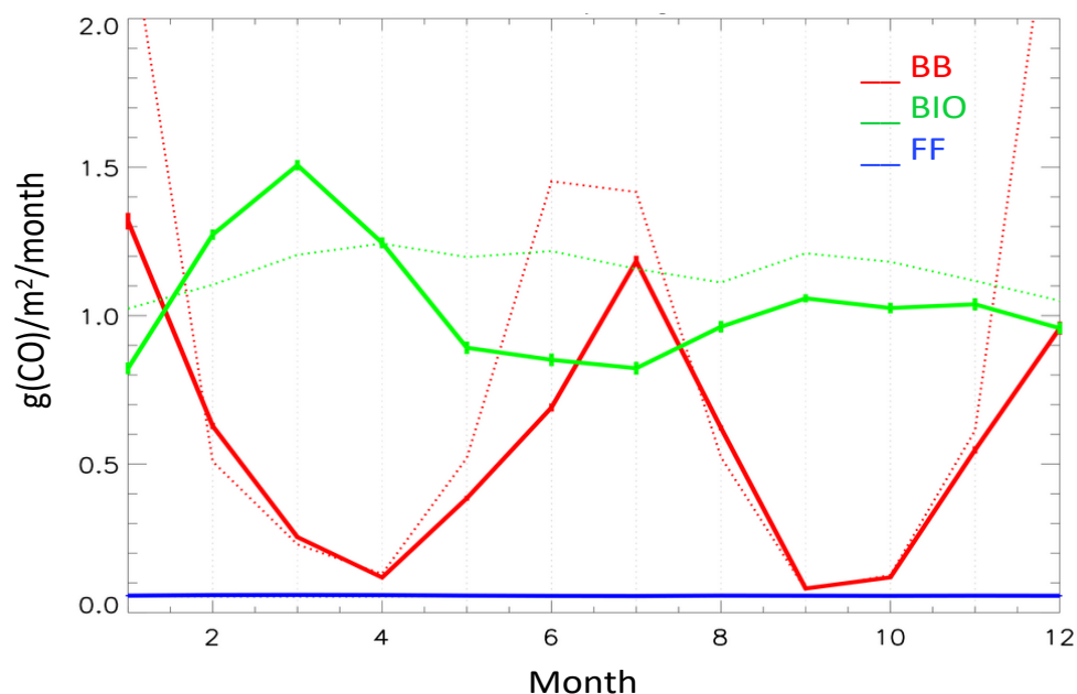
Figure S2. A posteriori (solid lines) and a priori (dotted lines) CO fluxes averaged for each month over 2005-2012 for the Equatorial Africa (Fig. S1) region for biomass burning (BB, red), biogenic (BG, green) and fossil fuel (FF, blue) sectors. Errors on the 8-yr average fluxes for this region are indicated for each sector and month, with values around 1.8% for BIO, 1.9% for BB and 4.2% for FF.
