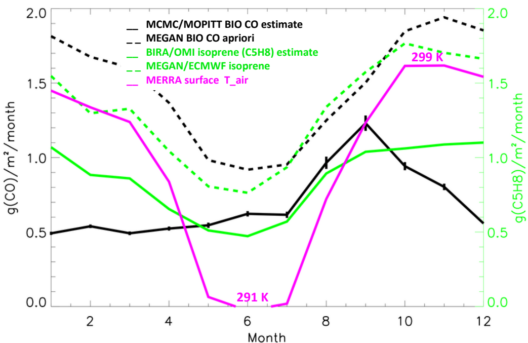
Figure S9. Average monthly CO (black) and C5H8 (green) fluxes and surface air temperatures (magenta, with minimum and maximum values indicated) for 2005-2012 for the S. America tropical Andes piedmont region (Fig. S7). Solid black and green lines show the posterior "top-down" fluxes while dashed black and green lines show the emissions predicted by MEGAN with associated meteorological fields.
