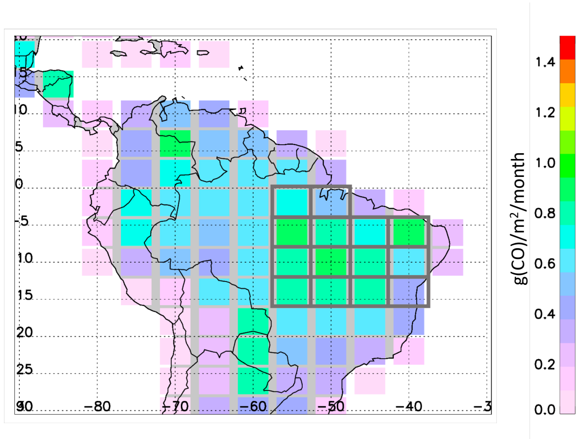
Figure S4. Map of a posteriori biogenic CO fluxes. Grey boxes indicate the S. American Amazon region used for the 2005-2012 average computed for each month.
