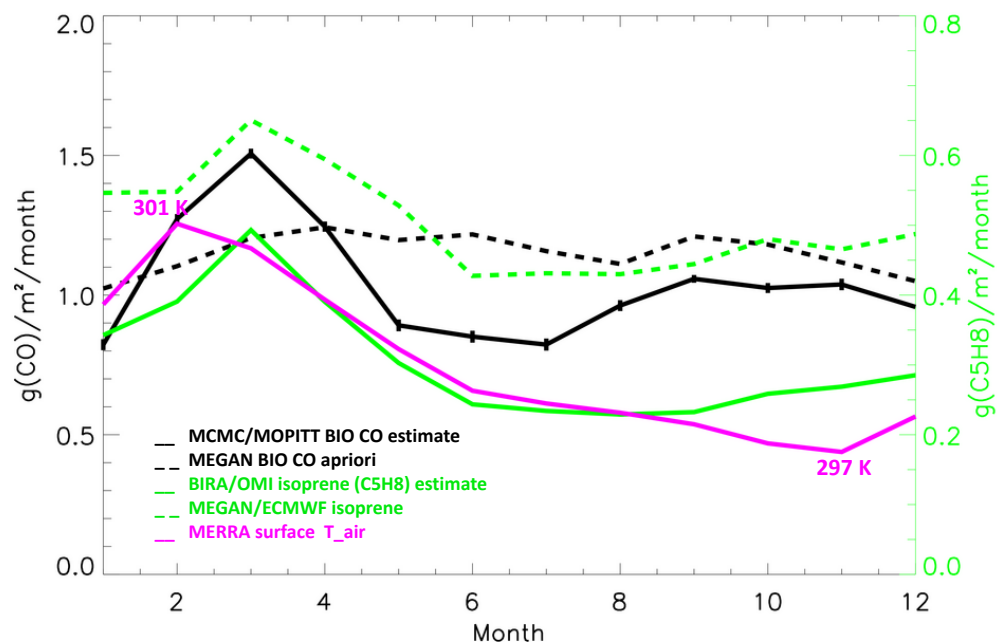
Figure S3. Average monthly CO (black) and C5H8 (green) fluxes and surface air temperatures (magenta, with minimum and maximum values indicated) for 2005-2012 for the Equatorial Africa region (Fig. S1). Solid black and green lines show the posterior "top-down" fluxes while dashed black and green lines show the emissions predicted by MEGAN with associated meteorological fields.
