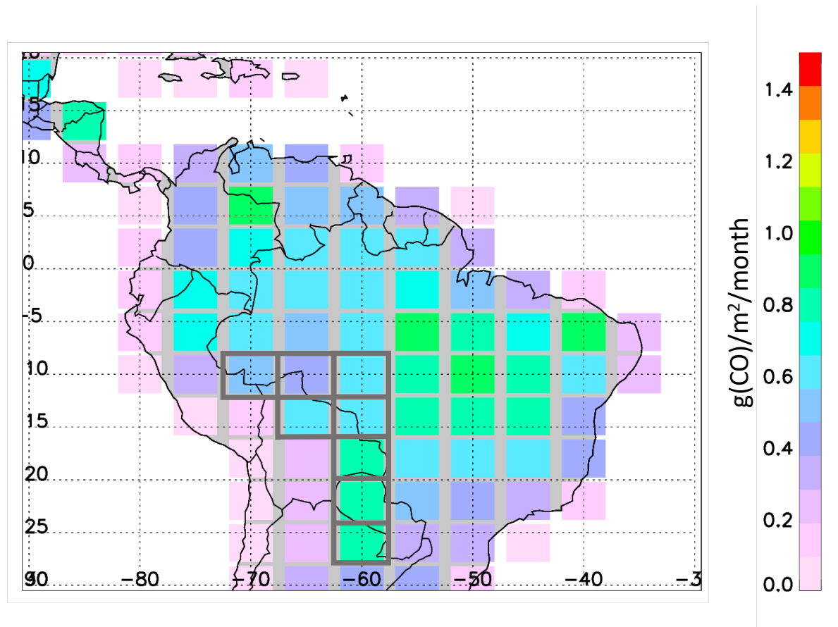
Figure S7. Map of a posteriori biogenic CO fluxes. Grey boxes indicate the S. American tropical Andes piedmont region used for the 2005-2012 average computed for each month.
