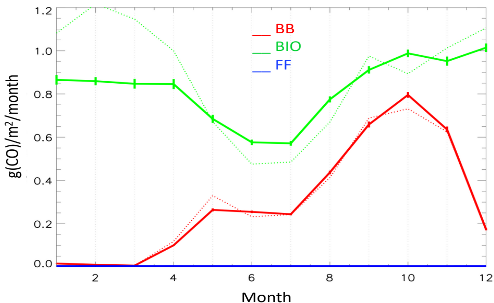
Figure S11. A posteriori (solid lines) and a priori (dotted lines) CO fluxes averaged for each month over 2005-2012 for the Australian tropics and subtropics region (Fig. S10) for biomass burning (BB, red), biogenic (BG, green) and fossil fuel (FF, blue) sectors. Errors on the 8-yr average fluxes for this region are indicated for each sector and month, with values around 2.2% for BIO, 2.1% for BB and 4.4% for FF.
