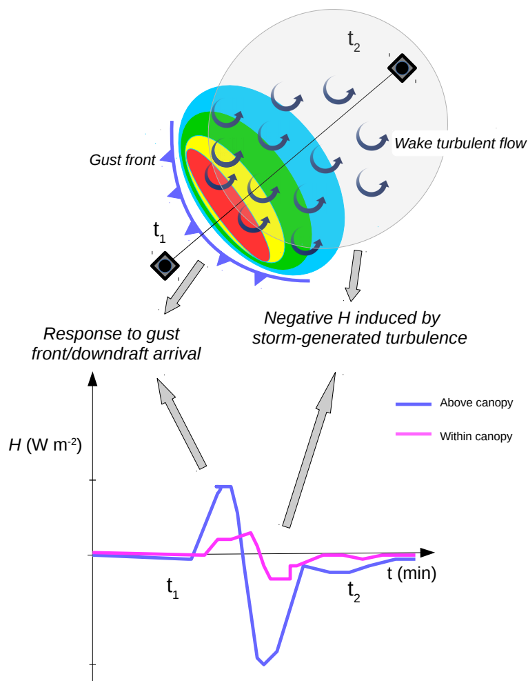
Figure 8. Schematics illustrating the effects of a gust front passage over a tall tower in the forest during nighttime hours. Top: a gust front (blue line with triangles) from a convective storm (color-shaded ellipsoids; cold [warm] colors represent low [high] radar reflectivity values) approaches the tall tower (gray square) at t_1 . At t_2 , the gust front has passed by the tower site which now is embedded in the cold pool's turbulent wake (gray large ellipsoid with circular arrows representing turbulent eddies). Bottom: corresponding sensible heat flux response to gust front passage at tower levels above (blue) and below (pink) the canopy.
