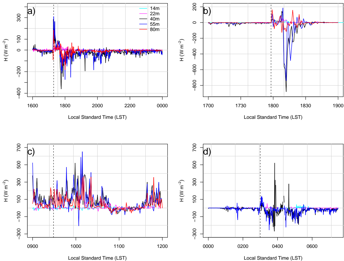
Figure 4. The same as in Fig. 2, but for sensible heat flux.
