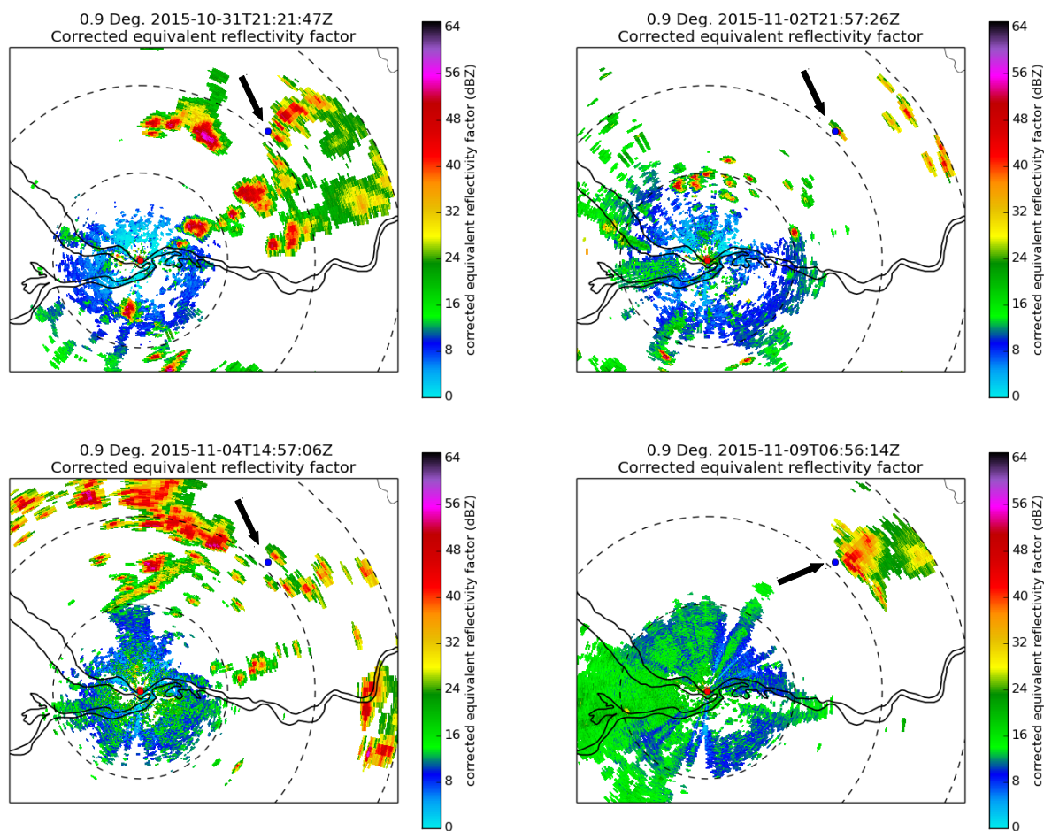
Figure 1. 0.9° PPI reflectivity imagery from the Manaus Doppler radar for the four DMC events studied. (upper left) 1721 on LST 31 Oct 2015, (upper right) 1757 LST on 2 Nov 2015, (lower left) 1057 LST on 4 Nov 2015, and (lower right) 0256 LST on 9 Nov 2015. The red (blue) dot shows the location of Manaus (ATTO tower). The black arrow indicates the convective elements that were sampled at the walk-up tower.
