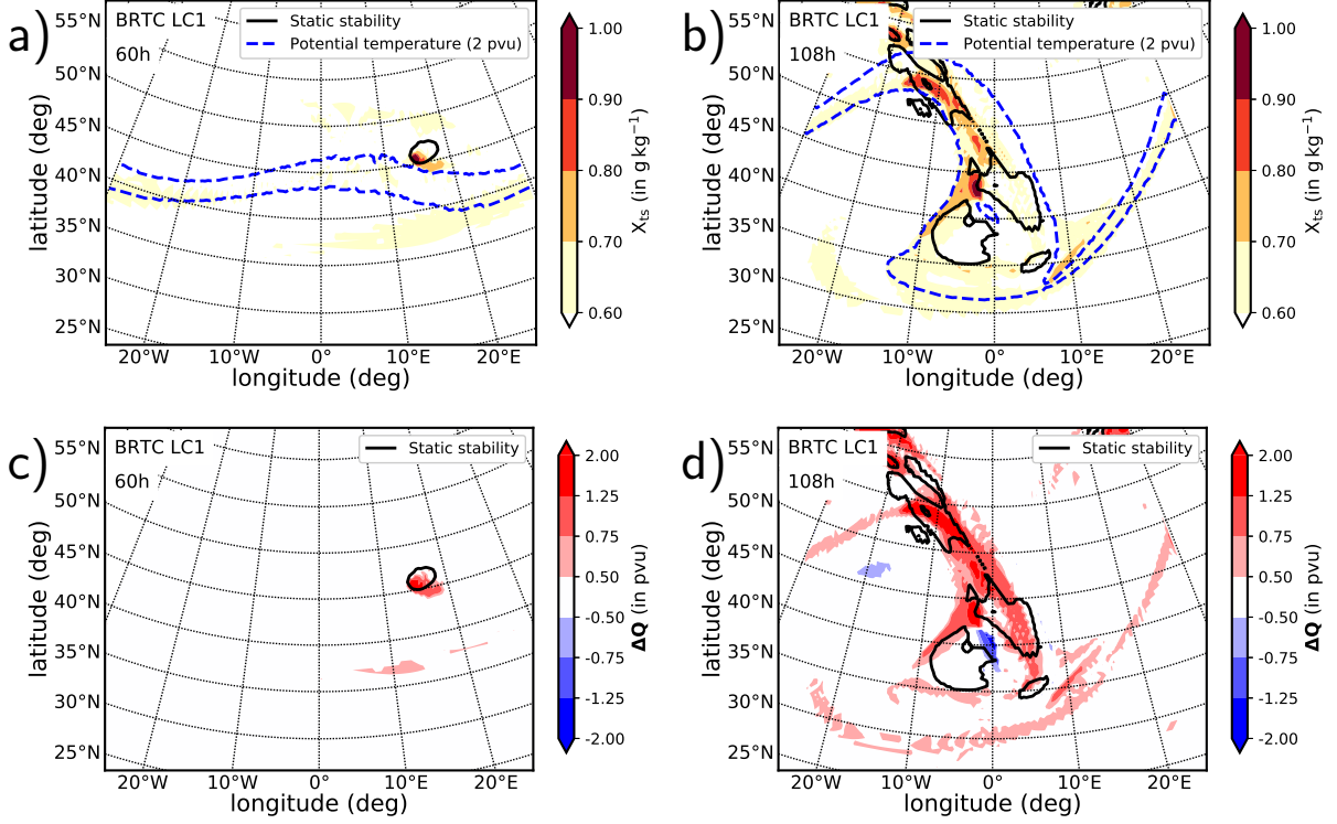
Figure 10. The tropospheric tracer X_{ts} on first full stratospheric level, i.e., the first full level with PV values larger 2 pvu for a) 60 h and b) 108 h after model start. Diabatic change of PV, \Delta Q = Q - Q_{0,\text{adv}} , at the level of the dynamic tropopause with Q_{0,\text{adv}} being the advected initial PV and Q being the full PV for c) 60 h and d) 108 h after model start. The black isoline shows static stability, N^2 = 5.5 \times 10^{-4} \text{ s}^{-2} . The blue dashed lines show isolines of potential temperature for 315 K and 325 K.
