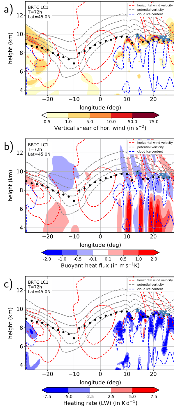
Figure 14. Zonal cross sections of a) vertical shear of horizontal wind S^2 , b) buoyant heat flux w'\Theta'_v , and c) long wave heating rate D\Theta_{\text{LW}}/Dt at 45°N and after 72 h of model integration. For the description of isolines it is referred to Figure 11.
