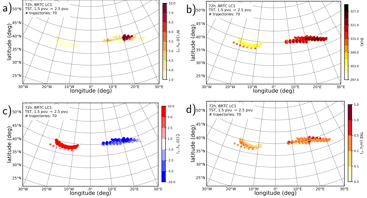
Figure 12. Trajectories starting 66 h and ending 72 h after model start which increase their PV from values smaller than 1.5 p.u. to values larger 2.5 p.u. within the six hour interval. Panels show a) static stability (in 10^{-4} \text{ s}^{-2} ), b) potential temperature (in K), c) relative vorticity (in 10^{-5} \text{ s}^{-1} ), and turbulent kinetic energy (in \text{m}^2 \text{ s}^{-2} ) along the trajectories for each hour.
