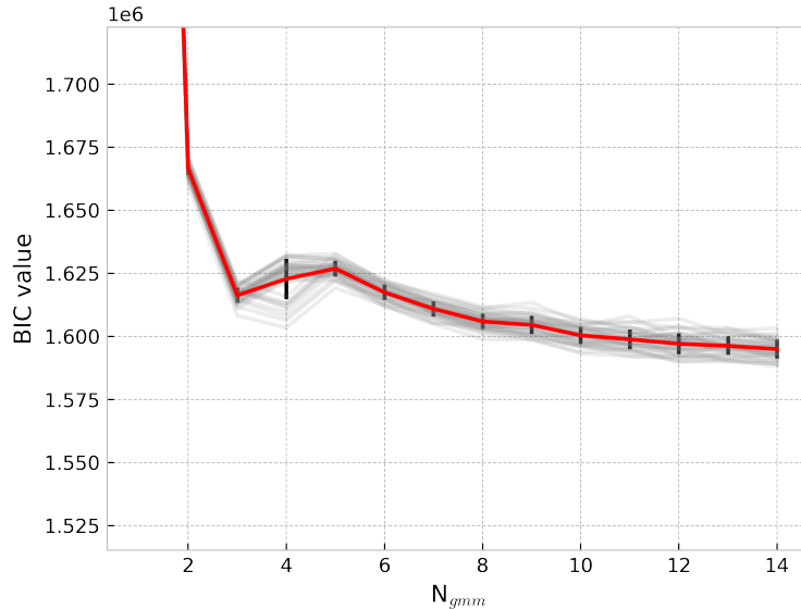
Figure 8. Bayesian Information Criterion (BIC) for different N_{GMM} choices applied to OceanRAIN. The mean BIC is shown in red with the standard deviation in black. Gray lines indicate GMM tests with limited samples, each a randomly chosen subset making up a third of the total data set.
