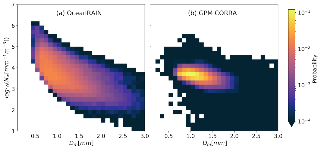
Figure 4. Probability histograms for OceanRAIN (a) and GPM CORRA (b) for observations of the normalized intercept parameter ( N_w ) and the mass-weighted mean diameter ( D_m ). Areas in white indicate no data.
