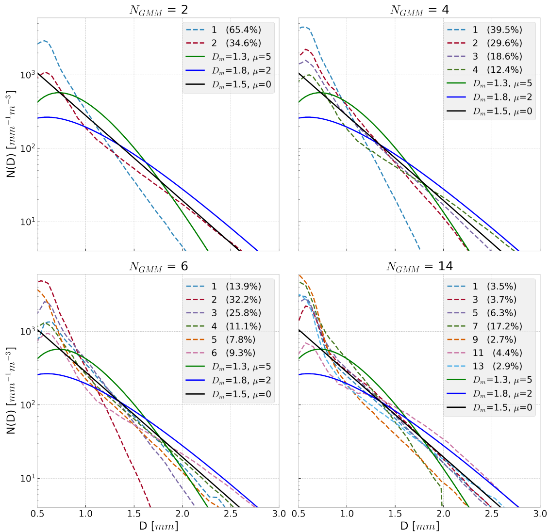
Figure 7. Panels show resultant DSDs for different GMM realizations (dashed lines) ranging from N_{GMM} of 2 to 14. The last panel shows only odd numbered GMM states to reduce clutter. Each panel has an identical set of NG curves with different \mu and D_m values (solid lines) for the sake of comparison. All curves have equal RWC. The frequency of occurrence for each GMM shape is given in the legend.
