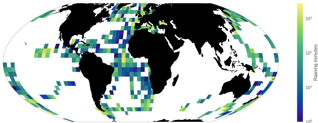
Figure 1. Raining minutes from OceanRAIN, selected by the sampling criteria of this study as described in Section 2.2, viewed on a regular 5° grid. Grid cells in white signify that no data points were used.
