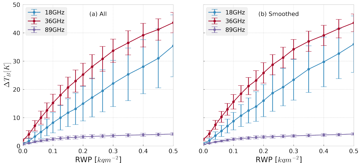
Figure 9. Simulated brightness temperatures ( T_B ) through a modeled atmosphere for warm rain, with a liquid cloud layer of 0.2 \text{ kg m}^{-2} from 1 to 2 km altitude and rain in the lowest kilometer. The RWC in the rain layer and the DSD are directly from disdrometer observations and constant in the rain layer. Given are the means (dots) and standard deviations ( \pm 1\sigma , shown as bars) of \Delta T_B per rain water path (RWP) bin, where the difference in T_B is defined relative to RWP = 0 . The left panel (a) uses all OceanRAIN observations, the right panel (b) shows results when averaging over consecutive 6 minute observation windows to approximate a satellite footprint.
