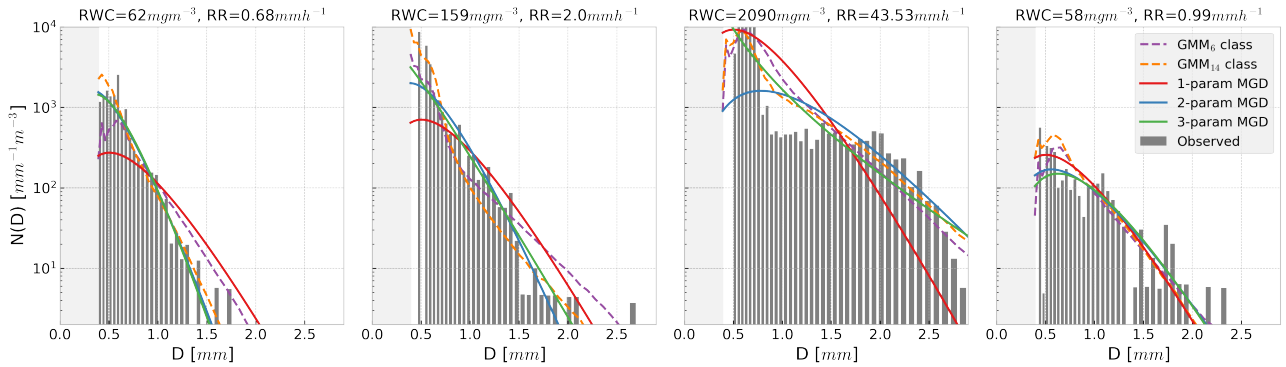
Figure 6. Each panel gives an OceanRAIN observed DSD, seen in the solid bars. Various fitted curves with identical RWCs are also given, including GMM-derived DSDs for N_{GMM} of 6 and 14, and 3 MGD curves. For the 1-parameter MGD and GMM curves only RWC is provided, and for the 1- and 2-parameter MGD curves \mu = 3 . The 2-parameter MGD has the calculated D_m while the 3-parameter MGD (i.e. NG) also has the fitted \mu . Each data point is identified by its RWC and rain rate. The light gray shaded region indicates an area of no OceanRAIN sensitivity.
