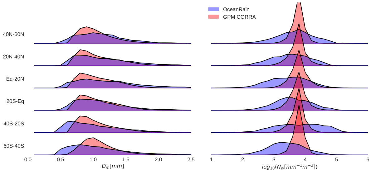
Figure 5. Normalized histograms of D_m (left) and \log_{10}(N_w) (right) for GPM CORRA and OceanRAIN, separated by latitude. All histograms use a linear y-axis of height 20%. GPM data are from the 3B CMB monthly gridded product.
