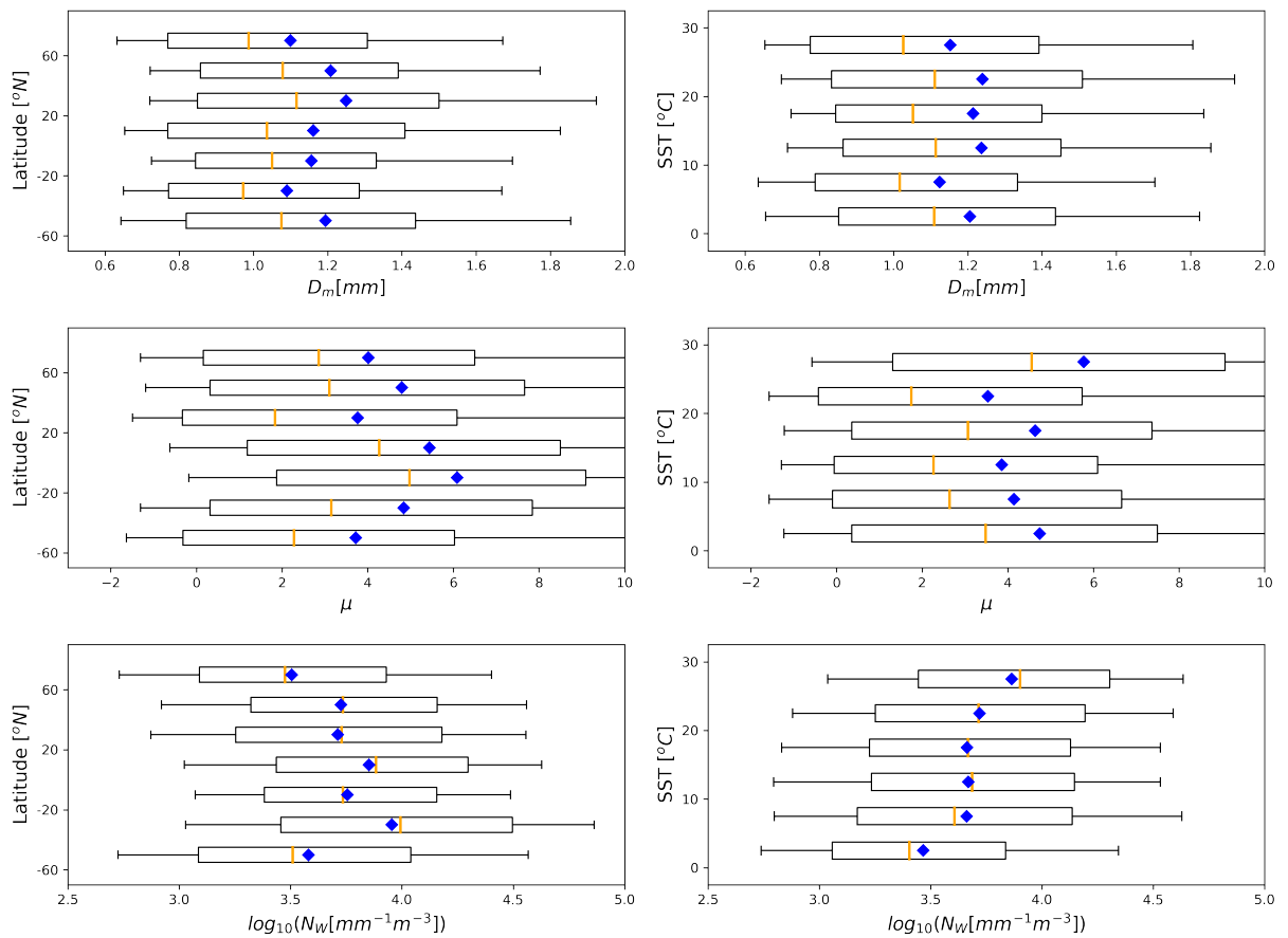
Figure 2. Distribution of DSD parameters following Eq. 3. The boxes define the standard deviations ( \pm 1\sigma ), the whiskers define the 10% and 90% bounds, orange lines denote the median, and blue diamonds the mean. Observations are divided according to latitude with 20^\circ bins (left) and sea surface temperature with 5^\circ\text{C} bins (right).
