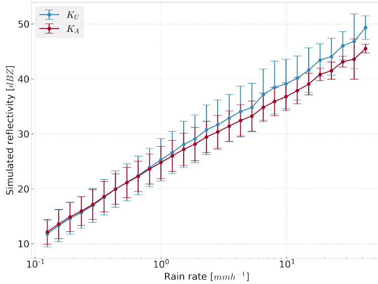
Figure 10. Simulated radar reflectivities at the two DPR frequencies, K_U and K_A bands, shown as means (dots) and standard deviations ( \pm 1\sigma , shown as bars) binned by rain rate. The rain rate and the DSD are directly from OceanRAIN observations.
