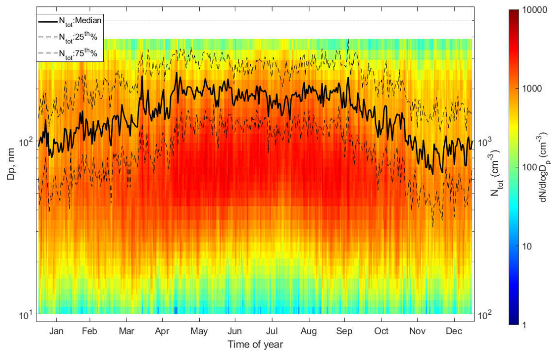
5 Figure 1: Seasonal variation of the aerosol number size distribution between 10-390nm presented as daily median aerosol number size distribution for the whole study period, 2000-2017. Superimposed on the surface plot is the median and quartile ranges of integral number concentration.
