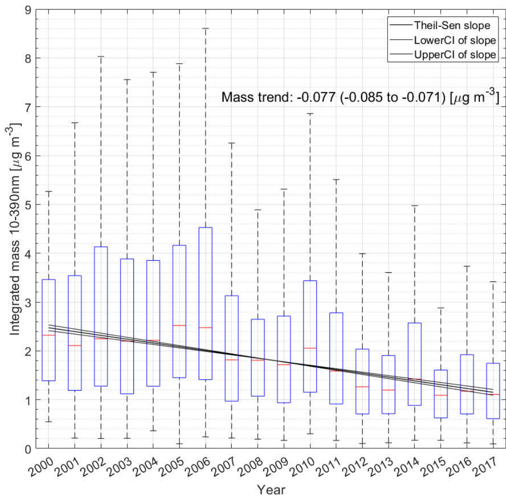
Figure 11: Box-Whisker plot of daily mean mass concentration 10-390nm assuming density of 1 \text{ g cm}^{-3} for Aspvyreten 2000-2017. Theil-Sen estimator slope and associated 95%CI of slope is indicated in figure by solid black lines. Note that outliers are excluded in the figure for improved clarity. Upper and lower bounds of boxes show 25 th -75 th percentile range, and whiskers 5 th -95 th percentile ranges of data. Red lines show median.
