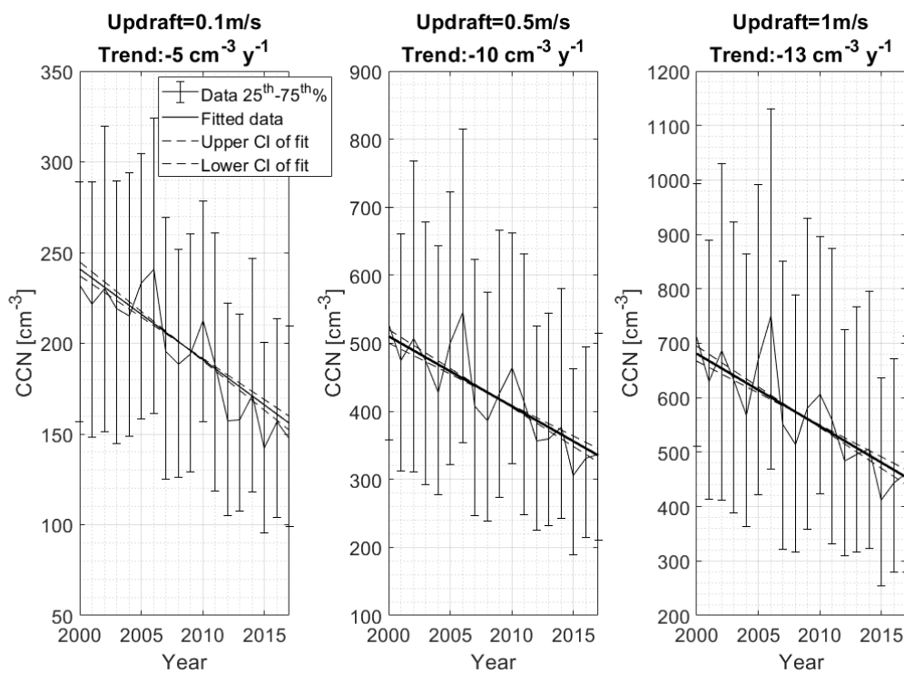
Figure 13: Trend of calculated CCN for different updrafts assuming a chemical composition ratio NH 4 SO 4 :Organic of 50:50. Figure shows median calculated CCN per year and corresponding 25 th -75 th percentile interval. Calculated linear trend as Theil-Sen slope and associated 95% confidence intervals are indicated by solid and dashed lines, respectively. Slope indicated in figure title. See text for further details.
