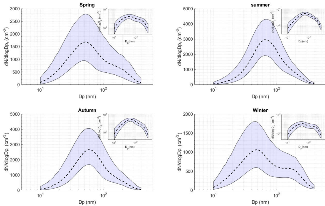
5 Figure 2: Seasonally average size distributions observed at Aspvreten 2000-2017. Shaded blue area gives 25 th -75 th percentile ranges, and dashed line median size distribution. Shown in the sub-frames are same data, but now in log-log scale. Spring=March-May; Summer=June-August; Autumn=September-November; Winter=December-February.
