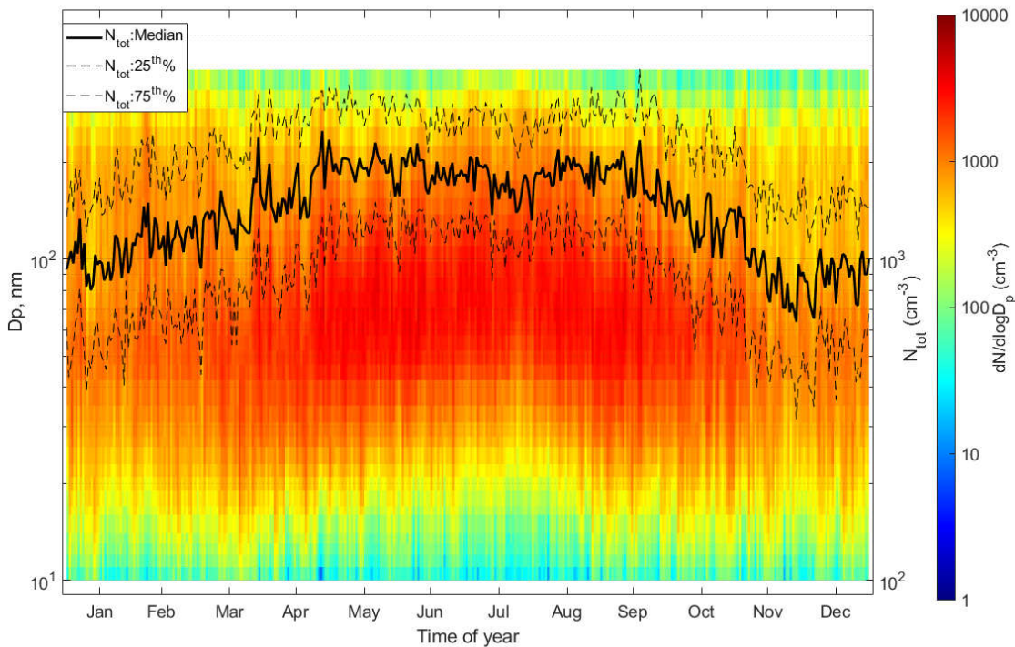
Figure 1: Seasonal variation of the aerosol number size distribution between 10-390nm presented as daily median aerosol number size distribution for the whole study period, 2000-2017. Superimposed on the surface plot is the median and quartile ranges of integral number concentration.
