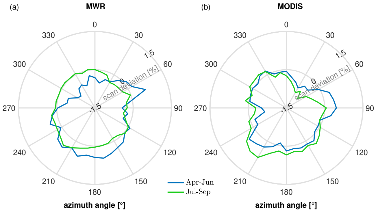
Figure 3. (a) Mean values of the MWR water vapor deviation (integrated up to the CBL height) from the mean per scan between 12–17 UTC for April–June (99 scans) and July–September (123 scans). (b) Same as (a) but for the MODIS IWV deviations including 22 overpasses (April–June) and 36 overpasses (July–September), respectively.
