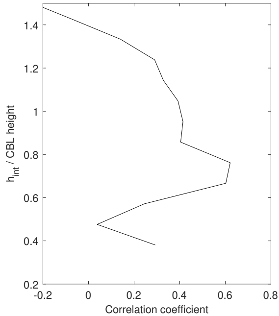
Figure 6. Correlation between 10^\circ sector estimates of term II of Eq. (2) and the slant path integrated water vapor at 30^\circ elevation and 10^\circ azimuth steps. h_{int} is the maximum height of the slant path that is used for the integration and is normalized by the CBL height.
