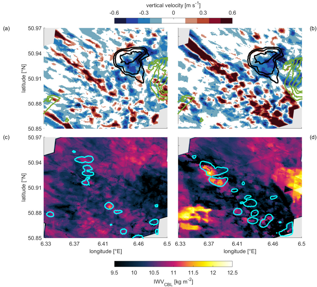
Figure 7. ICON-LEM vertically averaged vertical velocity (top) and integrated humidity (bottom) up to the CBL height of the ICON1 (a,c) and ICON2 (b,d) simulations. Contours in (a), (b) refer to the topography relative to JOYCE in ma.s.l. between -200 m to 0 m (green) and 0 m to 200 m (black) in 50 m steps. Contours in (c), (d) show areas with total column integrated cloud water values above 10 \text{ g m}^{-2} . The results are averaged between 12–13 UTC.
