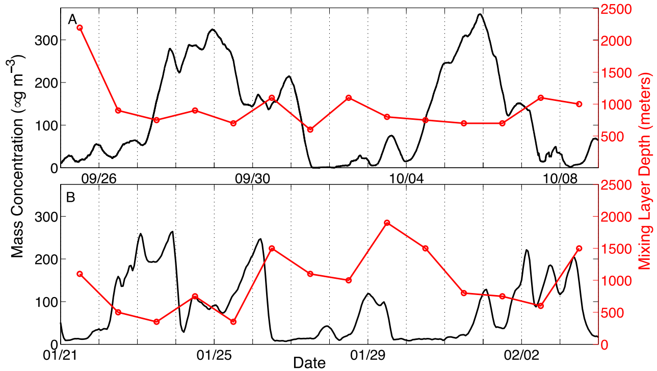
Figure S1. A comparison of the mixing layer depth (m) determined by the HYSPLIT model and the mass concentration ( \mu\text{g m}^{-3} ) in (A) Autumn 2013 and (B) Winter 2015.
