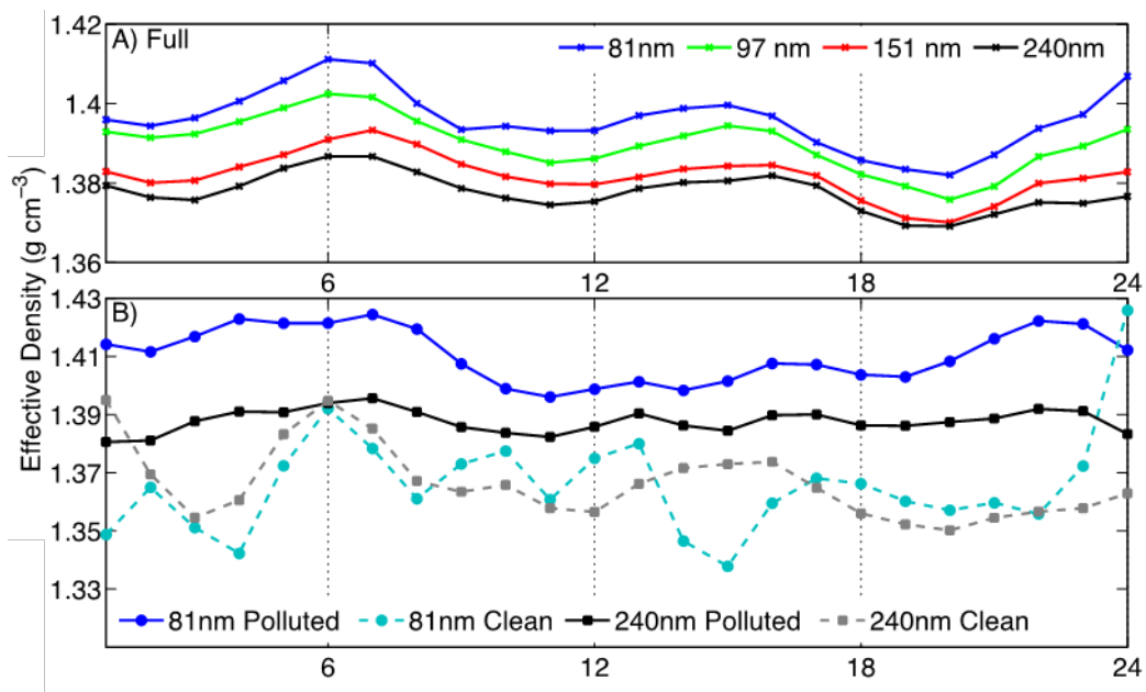
Figure 4. (A) The diurnal variation of the effective density ( \text{g cm}^{-3} ) of the four particle sizes from the full observational period.
