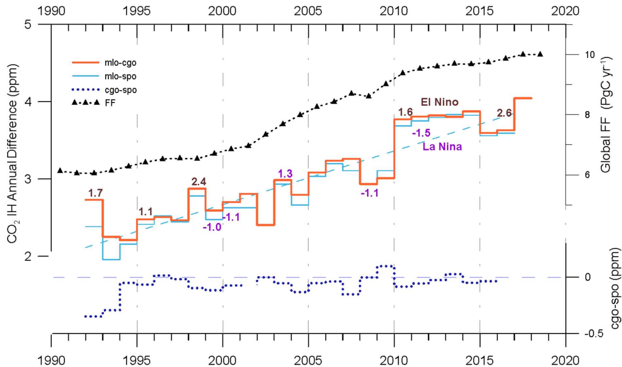
Figure 9: Annual changes in the baseline CO 2 difference between sites. Interhemispheric differences are plotted on the left axis. The peak magnitudes of strong El Niños (brown, ONI index > 1) and strong La Ninas (purple, ONI index < -1) are indicated. The cgo-spo annual differences are plotted on a doubled right-hand scale. Annual Fossil Fuel emissions from FF18, are shown on the top right axis.
