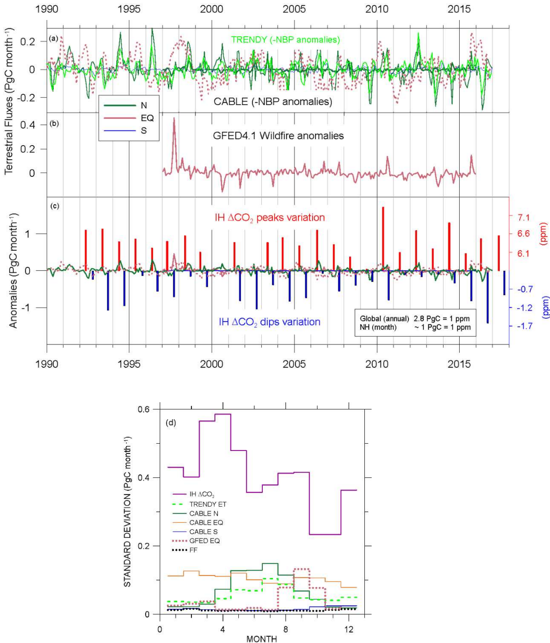
Figure 4: Comparison of the timing and amplitude of terrestrial emission anomalies (i.e. mean seasonality subtracted) with variations of the peaks and dips in Figure 3. (a) shows seasonal anomalies in CABLE emissions (dark green) and in 16-DGVM TRENDY extra-tropical emissions (Bastos et al., 2018; light green) and (b) shows GFED4.1 wild fire seasonal anomalies, for NH (green), EQ (pink) and SH (blue, SH/EQ for GFED4.1). In (c) The largest anomalies (CABLE NH, CABLE EQ, and GFED4.1 EQ) on the left axis are compared to the ppm variation in peaks (red) and dips (blue) on separate right axes. The axes scaling equates 1 PgC with 1 ppm (see text). To highlight seasonal differences, Figure 4(d) shows the standard deviation in the seasonal anomalies for each month, including those in anthropogenic emissions (Oda et al., 2017).
