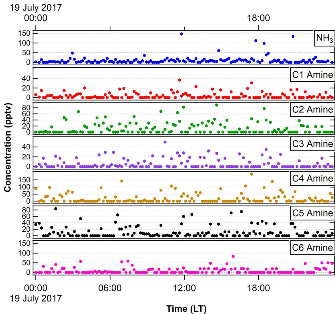
Figure 2. \text{NH}_3 and amines measured with the ethanol-CIMS in the FT-1 during the 2017 IOP in a very similar experimental condition as in 2018 IOP. We show here as an example one day of measurements (July 19, 2017).
