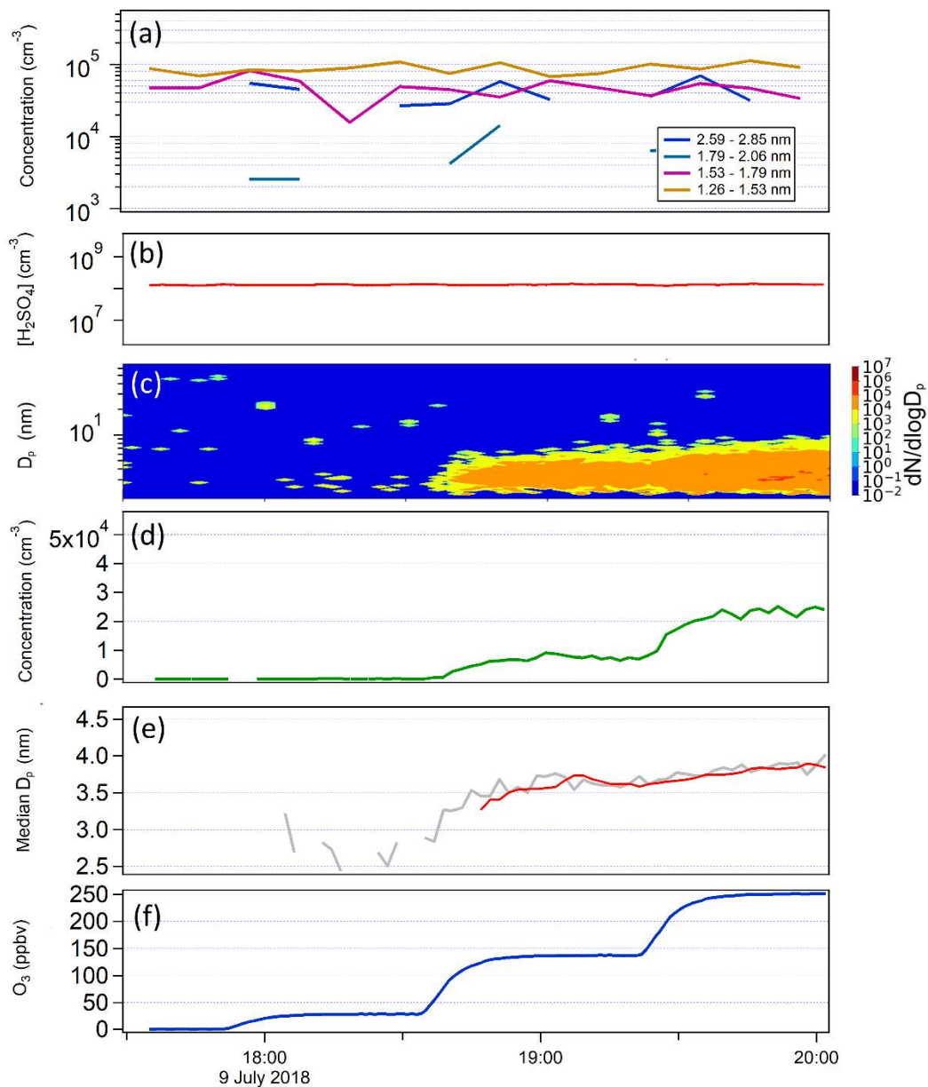
Figure 7. The same as Figure 6, except that FT-1 and FT-2 had a constant the same temperature in this test. Total particle concentration at the end of FT-1 was 1.7 \times 10^5 \text{ cm}^{-3} with a mean D_p of 1.9 nm and [\text{H}_2\text{SO}_4] in the FT-1 was 1.3 \times 10^8 \text{ cm}^{-3} . In FT-2, the [\text{H}_2\text{SO}_4] was estimated to be 2.5 \times 10^6 \text{ cm}^{-3} .
