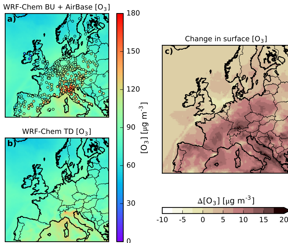
Figure 10. Monthly-averaged 12:00 h UTC surface O_3 concentration with bottom-up (BU, panel a) and top-down (TD, panel b) NO_x emissions. Panel c shows the difference between the two monthly averages (TD - BU).
