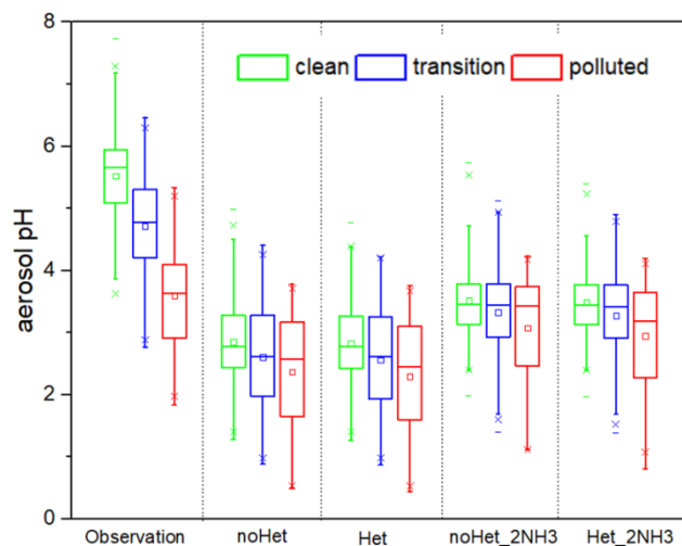
5 Figure 8: Box and whisker plot of observed and predicted aerosol pH by scenario and period.
