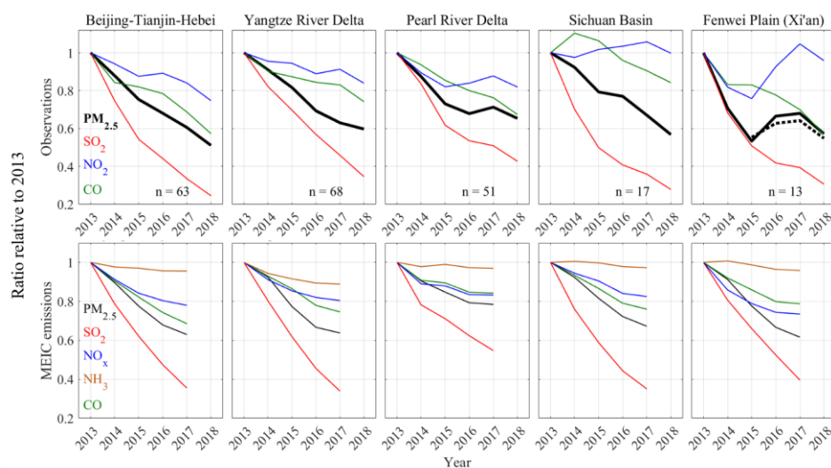
Figure 2. Relative trends of 2013-2018 observed concentrations and 2013-2017 MEIC emission estimates for the five target regions of Figure 1. The observed PM_{2.5} trends are shown as thick lines. Values are annual means referenced to 2013. The observed concentrations are averaged over all sites in each region with at least 70% data coverage for each year. The number of sites for each region is indicated. Fenwei Plain trends are for Xi'an as other sites did not start operating until early 2015. Post-2015 relative PM_{2.5} trends at these other sites are shown as the dashed line.
