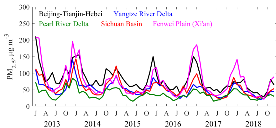
Figure 3 2013-2018 time series of monthly mean PM 2.5 concentrations over the five target regions. Values are averages from all sites in the region with over 70% data coverage for each of the six years.
