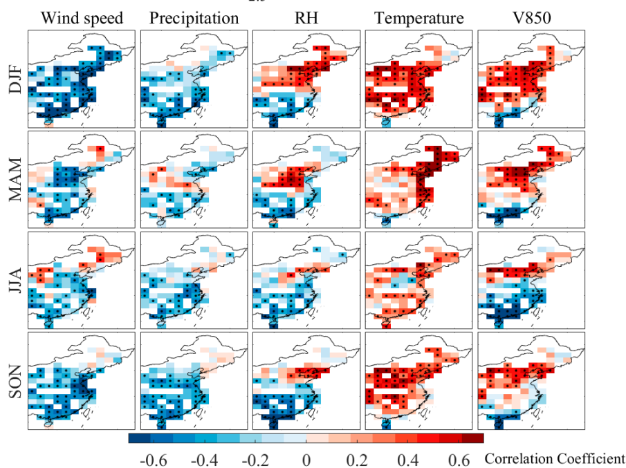
Figure 4 Correlation coefficients ( r ) of PM 2.5 concentration with the individual meteorological variables used in the MLR model: surface wind speed ( \text{m s}^{-1} ), precipitation ( \text{mm d}^{-1} ), relative humidity (RH; %), surface air temperature ( ^{\circ}\text{C} ), and 850hPa meridional wind velocity ( \text{m s}^{-1} ) for different seasons in China. The correlations are based on 10-day average observations on a 2^{\circ} \times 2.5^{\circ} grid. Dots indicate statistically significant correlations ( p < 0.05 ).
