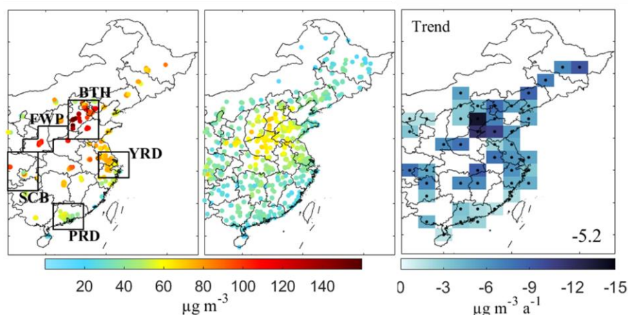
Annual mean PM 2.5 concentrations and trends, 2013-2018
