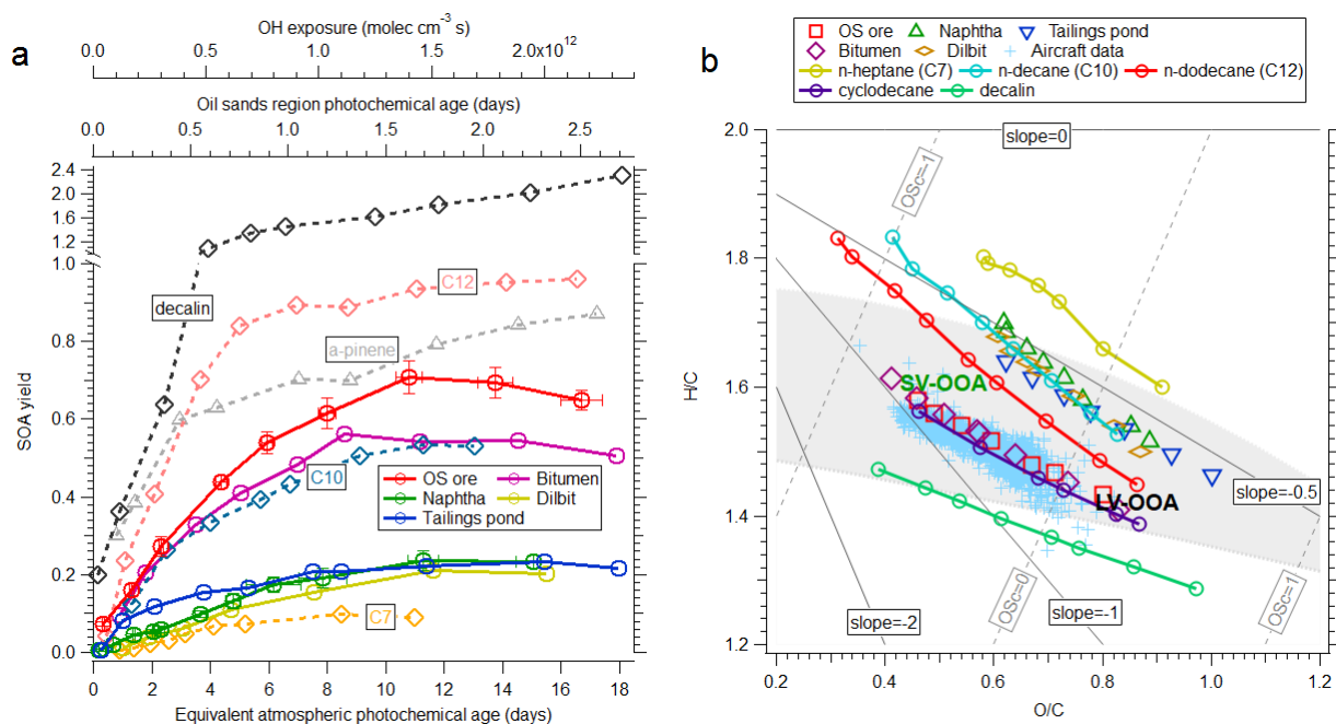
Figure 6. (a): LVOCs fate corrected SOA yield of OS-related precursors, alkanes and \alpha -pinene for AS seeded experiments. Representative error bars indicate \pm 1\sigma uncertainty in measurements. (b): Van Krevelen diagram for the SOA formed from OS-related precursors, selected alkanes and recent aircraft data in oil sands plumes (Liggio et al., 2016). The shaded area represents the elemental ratio space associated with ambient OOA (Ng et al., 2011).
