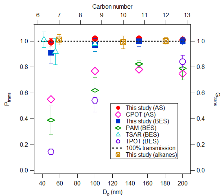
Figure 1. Particle (left and bottom axis) and gas (right and top axis) transmission efficiencies ( P_{trans} and G_{trans} ) for the ECCC-OFR. Particle transmission efficiencies of other OFRs are shown for comparison: PAM (Lambe et al., 2011), TPOT (Lambe et al., 2011), TSAR (Simonen et al., 2017), and CPOT (Huang et al., 2017).
