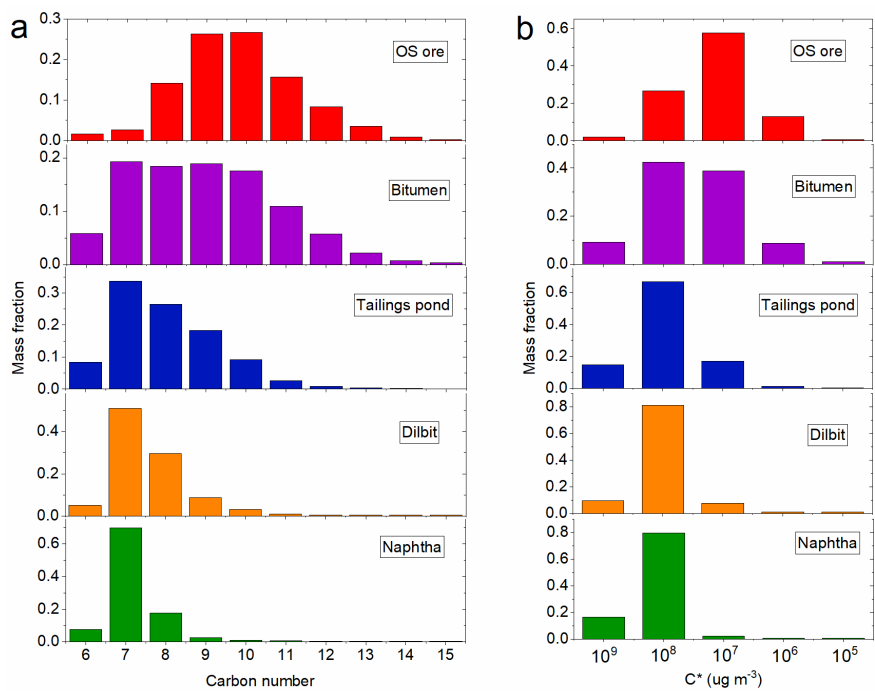
Figure 5. Volatility distribution of the OS-related precursors binned by carbon number (a) and effective saturation concentration C^* (b).
