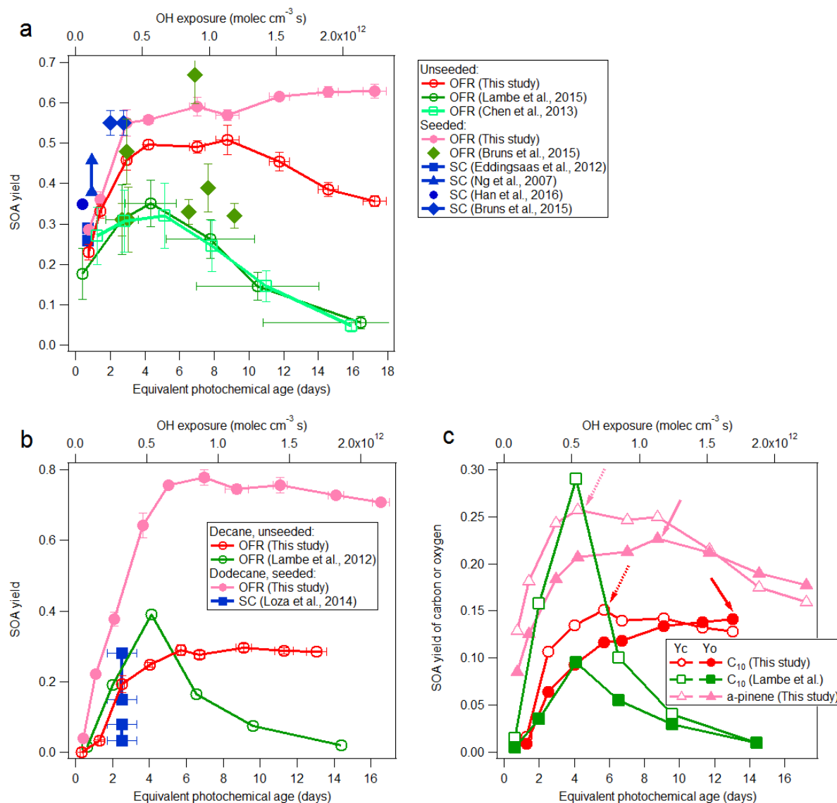
Figure 2. Low- \text{NO}_x SOA yields of \alpha -pinene (a), n -decane ( \text{C}_{10} ) and n -dodecane ( \text{C}_{12} ) (b), compared to previous studies using OFRs and smog chambers (SCs) (Ng et al., 2007; Eddingsaas et al., 2012; Lambe et al., 2012; Chen et al., 2013; Loza et al., 2014; Lambe et al., 2015; Bruns et al., 2015; Han et al., 2016). The details regarding these comparisons are shown in Table 2. (c): SOA carbon and oxygen yields ( Y_C and Y_O ) for single precursors for unseeded experiments in the current study and in a previous study (Lambe et al., 2012). Dashed and solid arrows indicate the maximum of Y_C and Y_O , respectively.
