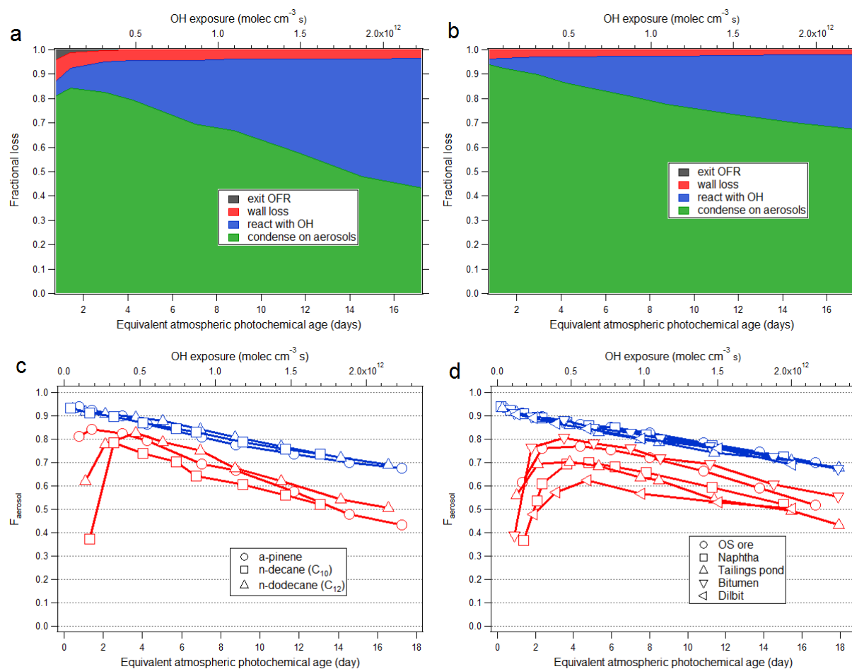
5 Figure 3. (a, b): The modeled fate of LVOCs in the current OFR as a function of photochemical age, for \alpha -pinene oxidation, in the absence (a) and presence (b) of AS seed particles. (c, d): Fraction of LVOCs that condense on aerosol ( F_{\text{aerosol}} ) in the OFR during the oxidation of the single precursors (c) and various OS-related precursors (d) (blue: seeded experiments; red: unseeded experiments).
