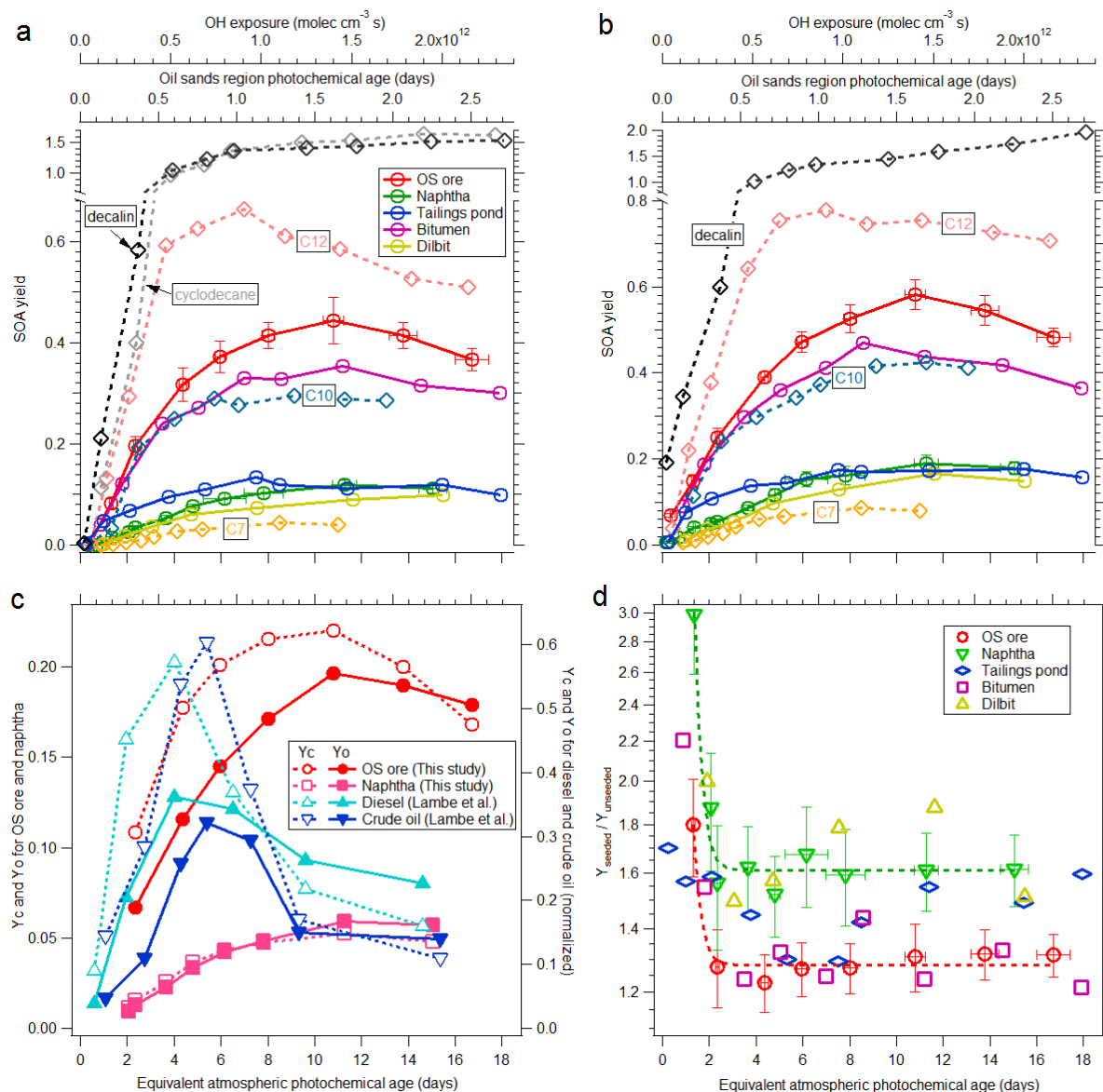
5 Figure 4. (a): SOA yields of OS-related precursors (OS ore, naphtha, tailings pond water, bitumen and dilbit) for unseeded experiments as a function of equivalent photochemical age and OH exposure. SOA yield of C 7 , C 10 and C 12 n -alkanes, cyclodecane and decalin are also shown for comparison. (b): SOA yields as in (a) in the presence of ammonium sulfate seed particles. (c): SOA carbon and oxygen yields ( Y_c and Y_o ) for the OS precursors of lowest and highest volatility (OS ore and naphtha solvent) compared to diesel and crude oil (Lambe et al., 2012). (d): Yield enhancement factor due to seed particles for OS-related precursors; dashed lines are exponential fittings for naphtha and OS ore data. Error bars indicate \pm 1\sigma uncertainty in measurements.
