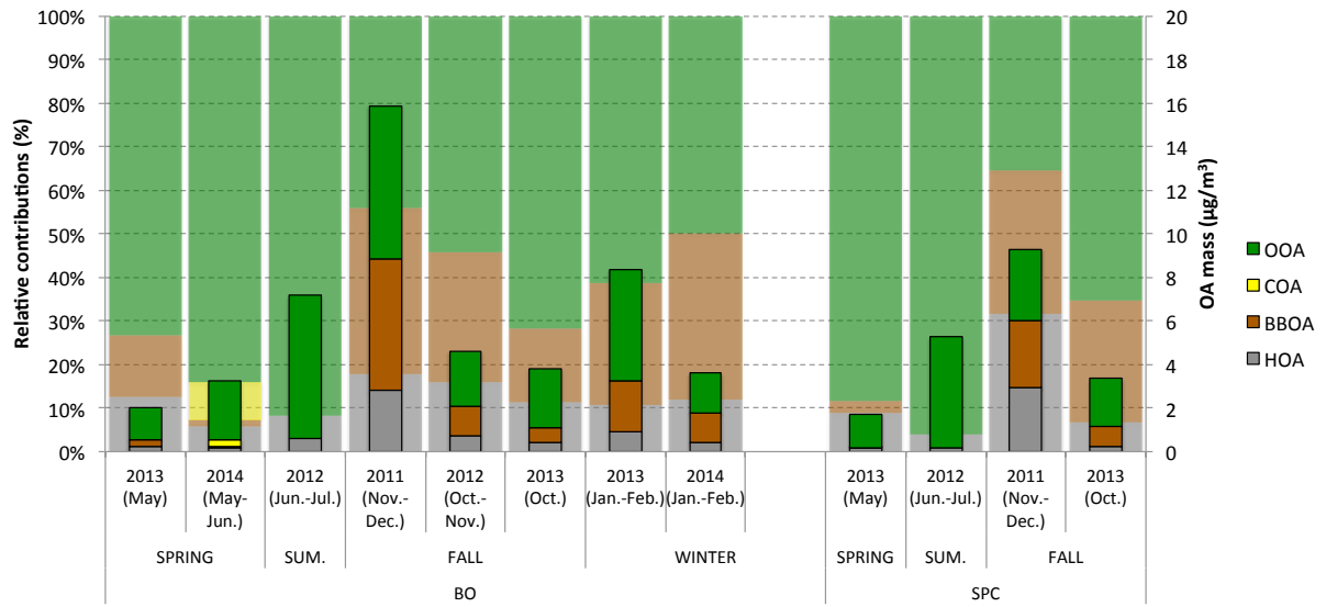
Figure 5: Organic aerosol sources contribution for each site and each SUPERSITO campaign. Relative contributions are reported as shaded histograms (referring to the left axis) in the background of the absolute ones (referring to right axis).
