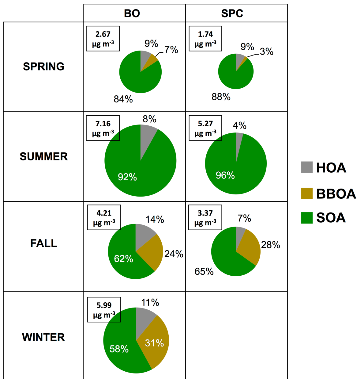
5 Figure 5: Seasonal relative contribution of the main OA sources in both urban and rural site. Pie-charts area is proportional to the total average concentration of OA (reported in the upper-left side of each box in term of \mu\text{g m}^{-3} ) and the individual portions are the average between the different campaigns made in the site in one season.
