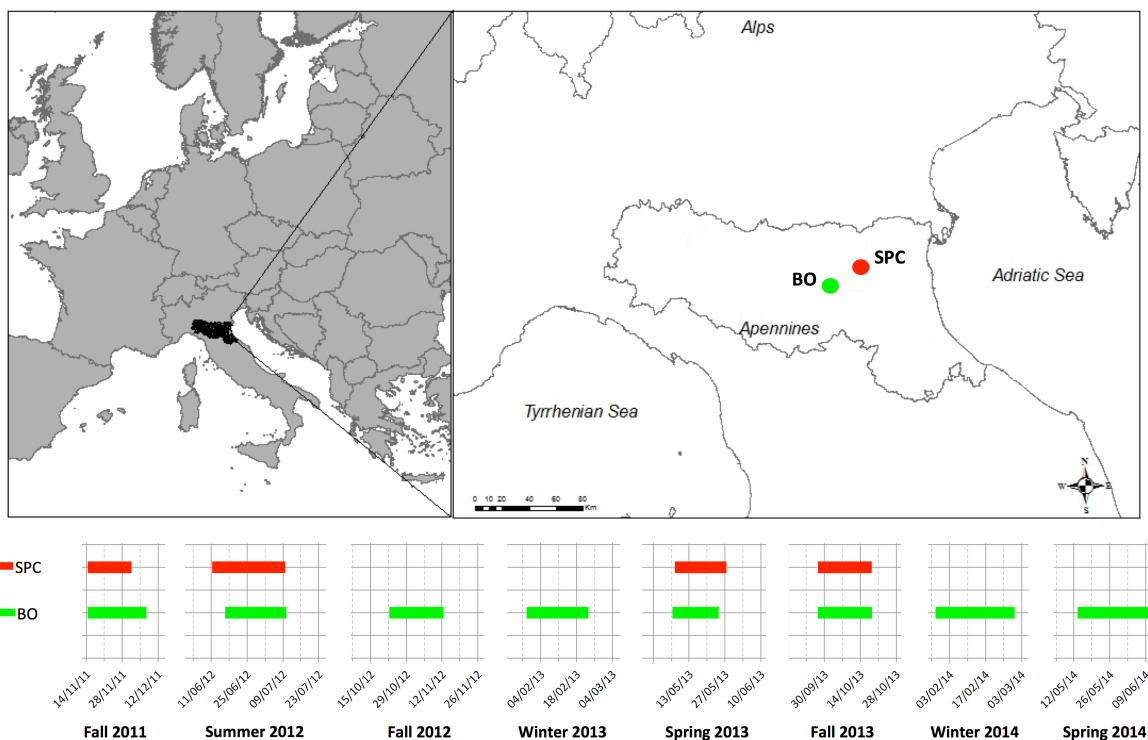
Figure 1: SUPERITO field campaigns: map of the sites and measurement periods considered in this study.
