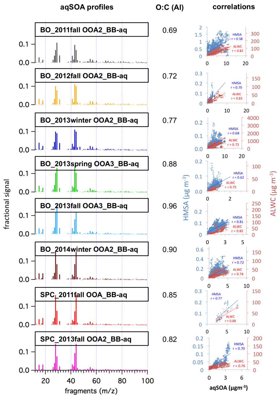
5 Figure 8: OOA x BB-aq main features: left column shows the mass spectral profile of each BB-aqSOA component identified during the SUPERSITO campaigns; the OOA factors are numerically ordered for each campaign based on their O:C ratios; central column reports the O:C elemental ratios of the same factors; right column illustrates the correlation between their concentration time series and the HMSA (in blue) and the ALWC (in red).
