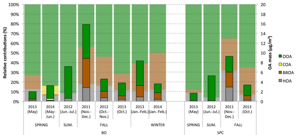
Figure 4: Organic aerosol sources contribution for each site and each SUPERSITO campaign. Relative contributions are reported as shaded histograms (referring to the left axis) in the background of the absolute ones (referring to right axis).
