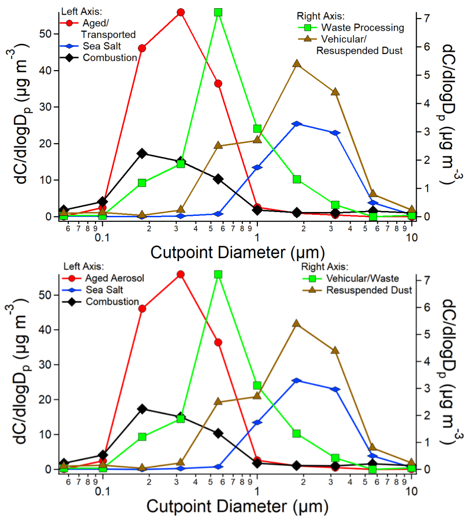
Figure 9. Reconstructed mass size distributions using PMF for the five major source profiles.
