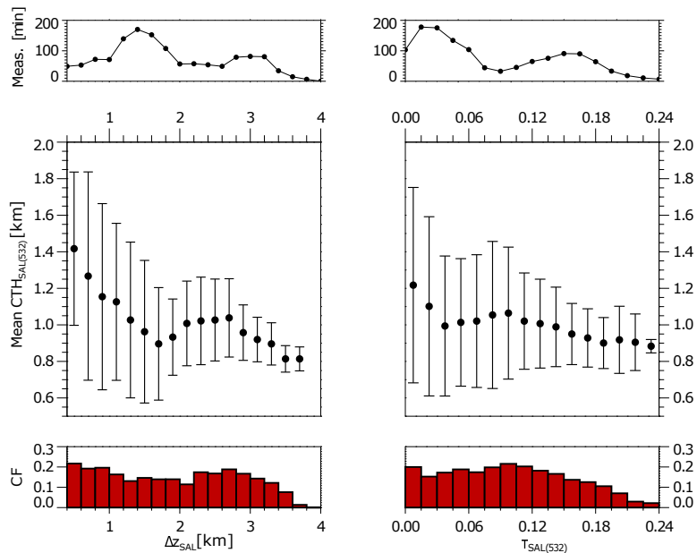
Figure 8. Left: Mean cloud top heights (middle) and cloud fraction (bottom) of clouds detected below Saharan dust layers as a function of Saharan dust layer vertical extent ( \Delta z_{SAL} ) - bin-interval: 0.2 km, Right: Mean cloud top heights (middle) and cloud fraction (bottom) of clouds detected below Saharan dust layers as a function of Saharan dust layer optical depth ( \tau_{SAL(532)} ) at 532 nm wavelength - bin-interval: 0.015. Bars mark respective standard deviations of mean cloud top heights ( 1\sigma ). The uppermost graphs illustrate summed measurement-times in each interval.
