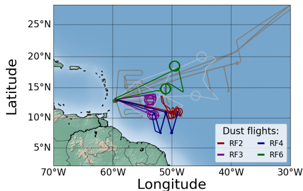
Figure 1. NARVAL research flight tracks: NARVAL-II dust-flights (color coded), NARVAL-II dust-free flights (light-grey), NARVAL-I (dark-grey).
