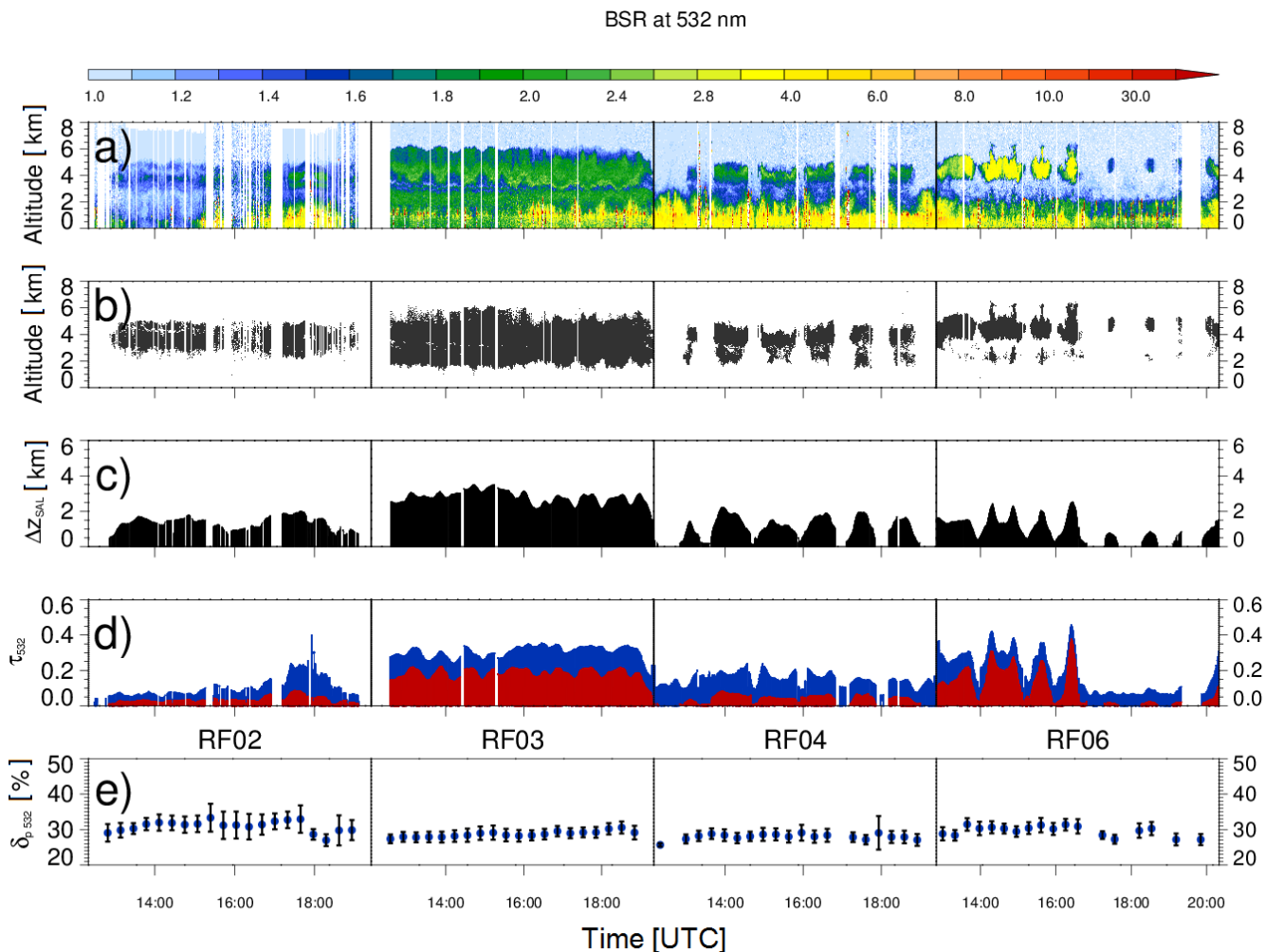
Figure 2. Overview of the four NARVAL-II research flights leading over Saharan dust-laden trade wind regions. (a) Cross sections of measured BSR at 532 nm and (b) applied mineral dust mask. (c) 10-minute boxcar average of the calculated dust layer vertical extent \Delta z_{\text{SAL}} . (d) 10-minute boxcar average of the derived total dust aerosol optical depth from aircraft to ground level \tau_{\text{tot}}(532) (blue) and aerosol layer optical depth \tau_{\text{SAL}}(532) (red). (e) Mean values and standard deviations of the measured 10-minute averaged SAL particle linear depolarization ratio ( \delta_{\text{p}532} ).
