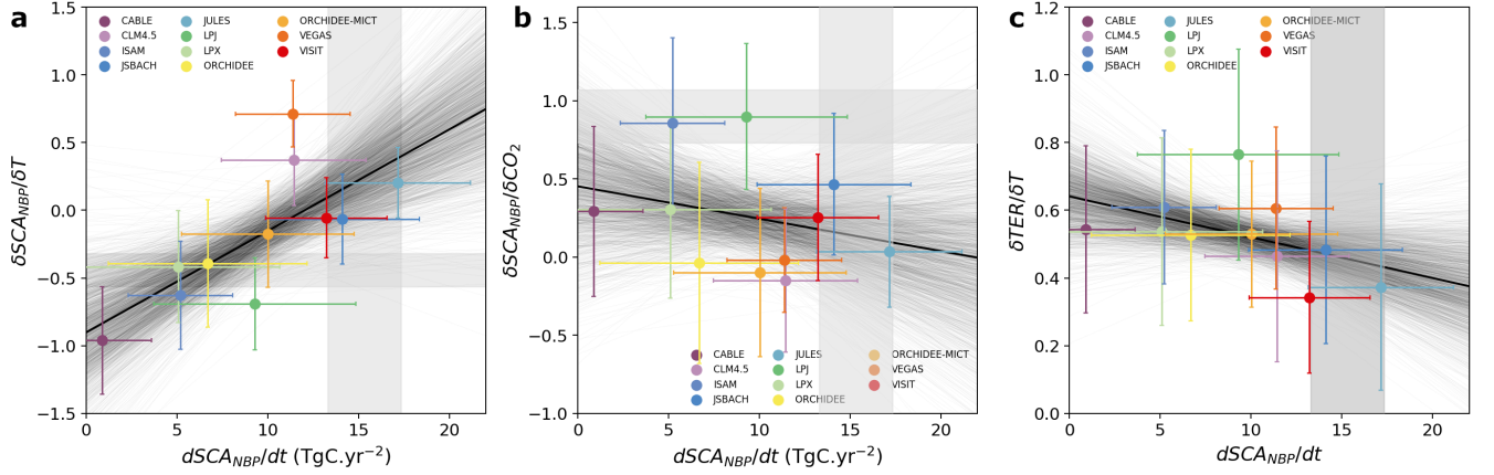
Figure 4. Emerging relationships between LSM sensitivities to climate and \text{CO}_2 and their SCA trends. The SCA_{NBP} trend for L_{>40N} estimated by each inversion (grey intervals) and corresponding responses of SCA_{NBP} to (a) T and (b) \text{CO}_2 (as calculated in Figure 3 but considering the scores of the regression only, shown in Figure S5) are compared to the results from individual models (simulation S3, coloured markers). In (c) the SCA_{NBP} trend for L_{>40N} estimated by individual models is compared with the simulated sensitivity of TER to T. The shaded areas indicate the inversion ranges, and the distribution of the grey lines shows uncertainty in the relationship between each pair of variables.
