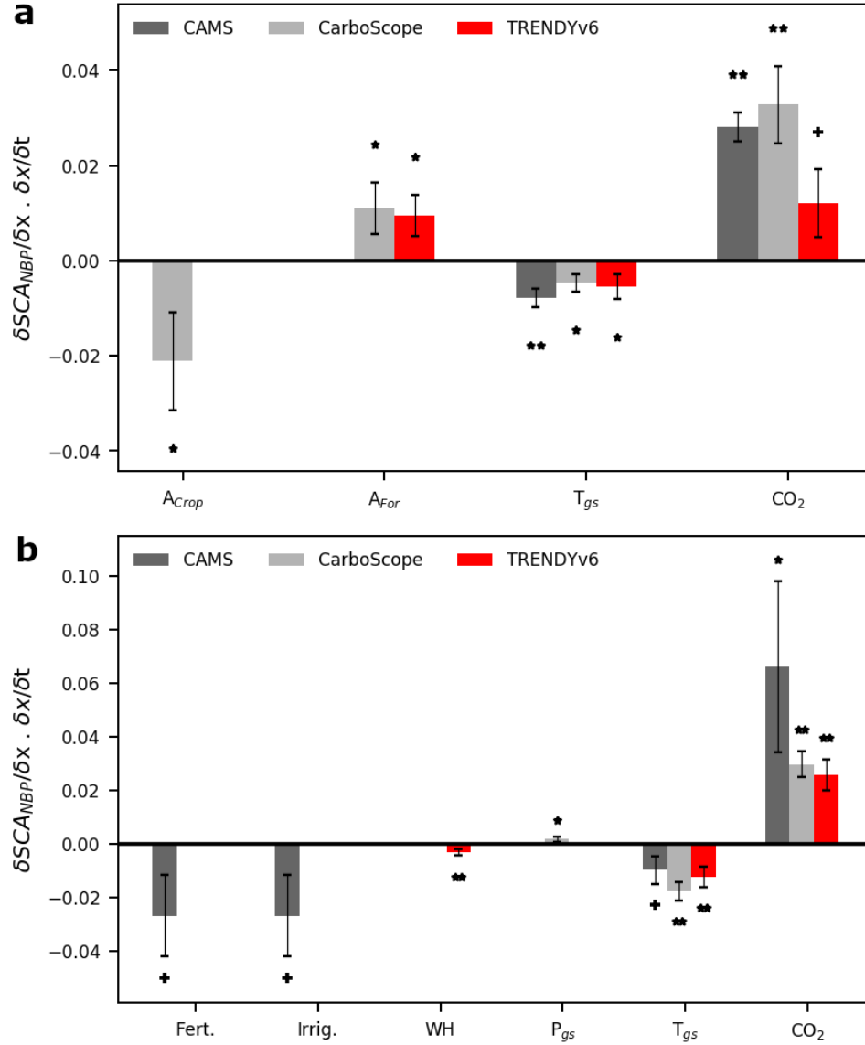
Figure 3. Statistical attribution of drivers of SCANBP estimated by the inversions and LSMs. The main drivers of SCANBP are presented for (a) L_{>40N} and (b) L_{25-40N} and are calculated as the product of the coefficients of a general linear model fit on SCANBP using a number of predictors (normalised) and their corresponding trends. Fertilization, irrigation, wood harvest, growing-season precipitation, growing-season temperature, atmospheric CO_2 concentration were tested as predictors, and the best fit was chosen for each dataset: CAMS (dark grey), CarboScope s76 (light grey), and the MMEM (red). The bars indicate the contribution of each predictor to the trend in SCANBP , error bars indicate the corresponding 95% confidence intervals, and the symbols indicate significant MRLM fits (two, one asterisks and crosses, p < 0.01 , p < 0.05 and p < 0.1 respectively).
