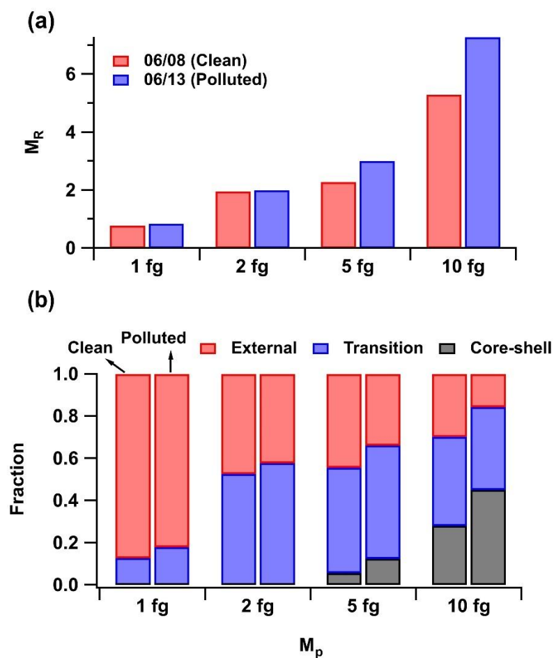
Figure 11. (a) The average M_R (the mass ratio of nonrefractory matter to rBC) under different CPMA setpoints (1 fg, 2 fg, 5 fg, 10 fg). (b) The fraction of different types of rBC-containing particles under different CPMA setpoints under varied pollution conditions.
