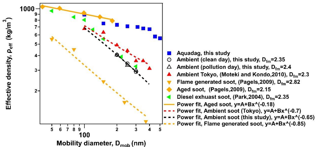
590 Figure 9. Relationship between effective density and mobility diameter of rBC-containing particles. The black circle and triangle denote the fresh rBC-containing particles ( D_p/D_c = 1 ) measured on clean days and polluted days in this study. Other markers denote the data from previous research.
