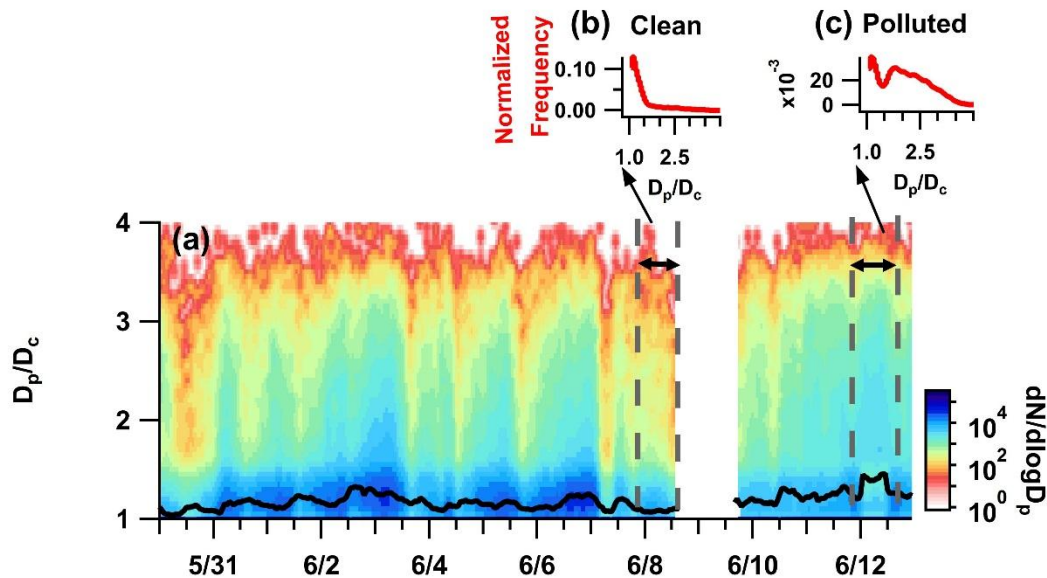
Figure 7. (a) Temporal variation in D_p/D_c , with D_c=180 nm, the image plot denotes the frequency ( dN/d\log D_p ) of rBC-containing particles with varied D_p/D_c . The black line denotes the average D_p/D_c for each hour. (b) The normalized frequency of D_p/D_c for the clean period before the tandem experiment. (c) The normalized frequency of D_p/D_c for the polluted period.
