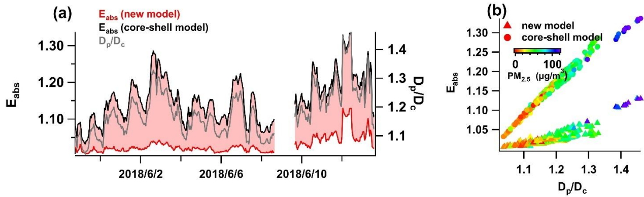
Figure 12. (a) Time series of D_p/D_c with D_c=180\pm 10 nm and E_{\text{abs}} at 550 nm wavelength with D_c=180\pm 10 nm using the core-shell model and the morphology-dependent model. (b) Relationship between E_{\text{abs}} and D_p/D_c . Circles denote the E_{\text{abs}} derived from the core-shell model, and triangles denote the E_{\text{abs}} derived from the morphology-dependent model.
