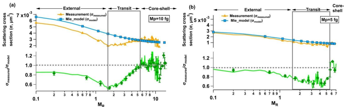
595 Figure 10. (a) Upper panel: scattering cross section of rBC-containing particles as measured by SP2 (yellow line) and calculated by Mie theory (blue line), assuming a core-shell structure. Bottom panel: the ratio (green line) between these two scattering cross sections at a CPMA setpoint of 10 fg as a function of M_R (the mass ratio of nonrefractory matter to rBC). (b) the same as (a) but for a CPMA setpoint of 5 fg.
